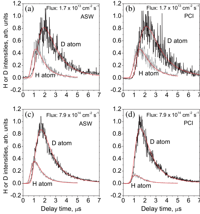
FIG. 1 (color online). Delay-time spectra of photodesorbed H (gray line) and D (black line) atoms from ices at 10 K: (a) ASW, (b) PCI for the atomic flux of 1.7 \times 10^{13} atoms \text{cm}^{-2} \text{s}^{-1} , (c) ASW, (d) PCI for the atomic flux of 7.9 \times 10^{14} atoms \text{cm}^{-2} \text{s}^{-1} . The red lines are fits to the data derived assuming Maxwell-Boltzmann distributions with translational temperatures in range 25–50 K for the spectra of the H and D atoms.
