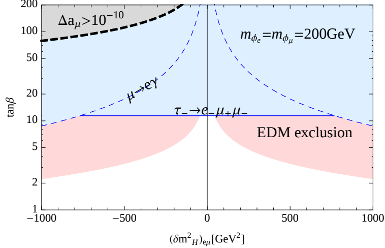
FIG. 4. (\delta m_H^2)_{e\mu} (GeV 2 ) and \tan \beta with m_{\phi_e} = m_{\phi_\mu} = 200 GeV.
