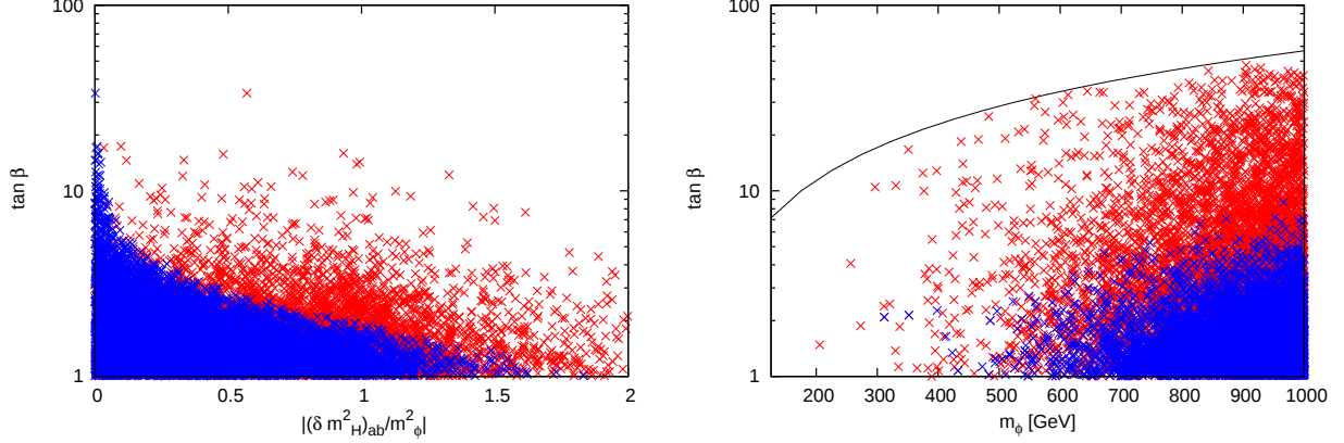
FIG. 5. |(\delta m_H^2)_{ab}/m_\phi^2| and \tan \beta (left), and m_\phi (GeV) and \tan \beta (right). m_{A_e} and m_{A_\mu} are fixed at m_\phi , and m_\phi is within 126 GeV and 1 TeV range. In the left figure, blue points figure out |(\delta m_H^2)_{\mu e}/m_\phi^2| and |(\delta m_H^2)_{ee}/m_\phi^2| , and red points are (\delta m_H^2)_{\mu\mu}/m_\phi^2 . In the right figures, |(\delta m_H^2)_{ab}/m_\phi^2| is larger than 0.01. The blue (red) points are the allowed ones for the experimental bounds with (without) the upper limit of the electron EDM. The black line is the upper bound in the case with |(\delta m_H^2)_{ab}| = 0 .
