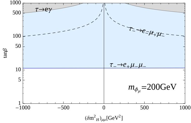
FIG. 3. (\delta m_H^2)_{\mu\mu} (GeV) and \tan\beta . The gray (light-blue) is excluded by \tau \rightarrow e\gamma at m_{\phi_\mu} = 200 GeV. The region above the dashed line is the upper bound from \tau^- \rightarrow e^- \mu^+ \mu^- and the blue region is the excluded one by \tau^- \rightarrow e^+ \mu^- \mu^- .
