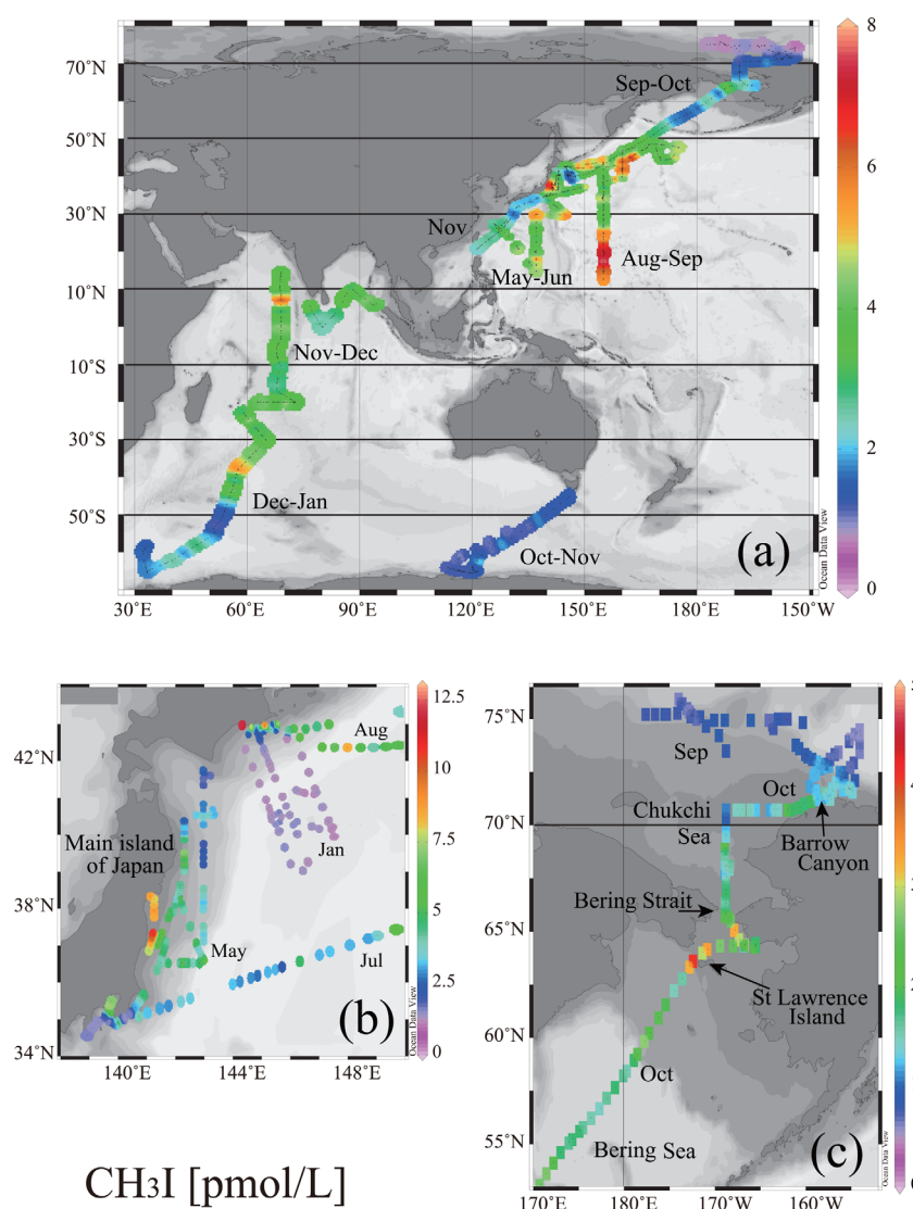
Figure 5. (a) Global-scale map of the horizontal distribution of \text{CH}_3\text{I} concentrations in surface mixed layer water and (b) enlarged maps of \text{CH}_3\text{I} concentrations in the western NW Pacific around Japan and (c) in the Bering Sea and Arctic Ocean.
