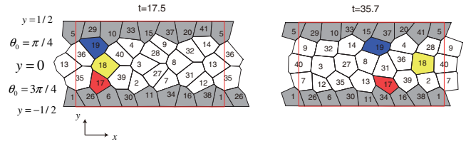
FIG. 3 (color online). Unidirectional movement of a cell sheet due to directional dependent contraction and spatial variation of \theta_0 along the y axis. Cells are colored so that the changes in configuration can be easily seen. The parameters are \tau_1 = 1.0 , \gamma_0 = 0.2 , \gamma_1 = 0.2 , K = 4.0 , K_p = 1.0 , A_0 = 0.048 , L_y = 1 , L_x = \sqrt{3} , K_B = 100.0 , \ell^* = 0.001 , b = 0.045 , \theta_0 = \pi/4 for (y_i + y_j)/2 > 0 and \theta_0 = 3\pi/4 for (y_i + y_j)/2 < 0 , and \eta_i = 100.0 for vertex i on the boundaries at y = \pm L_y/2 and \eta_i = 1.0 for the other vertices. The units of all parameters are arbitrary.
