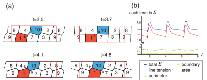
FIG. 2 (color online). Spontaneous and continuing shear movement of epithelial cells due to directionally dependent contractions; \theta_0 = \pi/4 . (a) Snapshots of cell configurations. (b) Time series of each term in E . The total value of E can increase due to the directional dependence of \gamma_{ij} [see Eq. (9)]. The parameter values are \gamma_0 = 0.5 , \gamma_1 = 0.5 , K = 4.0 , K_p = 1.0 , A_0 = 0.35 , L_y = 1 , L_x = 8\sqrt{3}/5 , b = 0 , \eta_i = 1.0 , \ell^* = 0.001 , and K_B = 100.0 . The units of all parameters are arbitrary.
