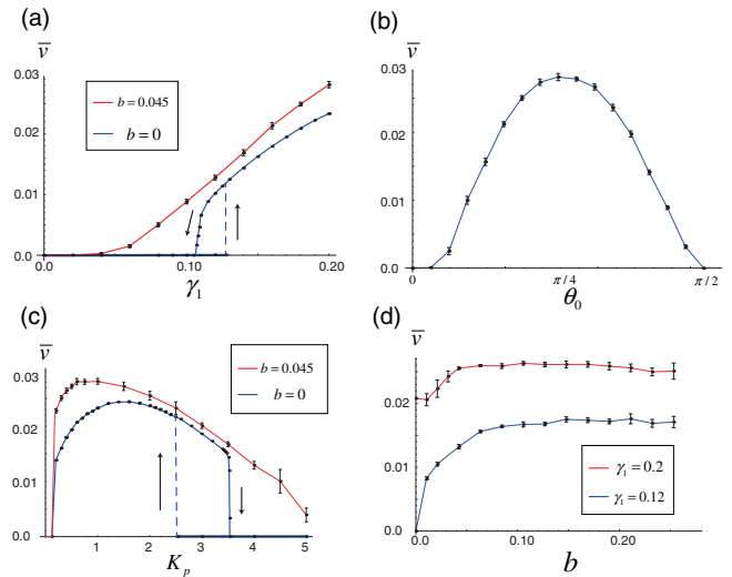
FIG. 4 (color online). Average speed of the collective movement of cells as a function of the various parameters: (a) \gamma_1 , (b) \theta_0 , (c) K_p , and (d) noise intensity b . Error bars indicate the standard deviation of \bar{v} (sample size = 10). The parameter values used here are the same as those used in Fig. 3 except where indicated in each graph.
