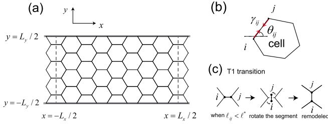
FIG. 1 (color online). Setup of the model. (a) The cell sheet is sandwiched between two parallel lines fixed at y = \pm L_y/2 . These represent the boundaries between other tissues and the cell sheet under consideration. Periodic boundary conditions are imposed at x = \pm L_x/2 . (b) A contraction force \gamma_{ij} acting on the cell boundary ij depends on the angle \theta_{ij} between the cell boundary and the positive x axis. (c) If the length of some cell boundary ij becomes shorter than a given small value \ell^* , the boundary is rotated 90^\circ and the connection is remodeled (T1 transition).
