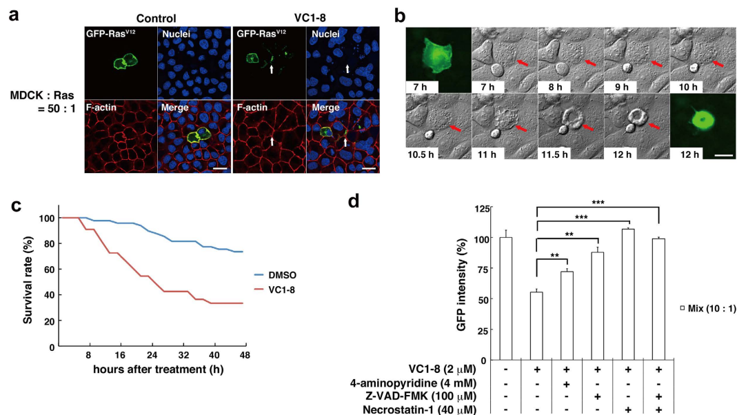
Figure 3. VC1-8 induces cell death of transformed cells that are surrounded by normal cells. (a) Immunofluorescence images of MDCK-pTR GFP-RasV12 cells that are surrounded by MDCK cells in the absence (left) or presence (right) of 2 \mu M VC1-8 for 16 h. Cells are stained with Hoechst 33342 (blue) and Alexa-Fluor-568-conjugated phalloidin (red). Arrows indicate a cell with fragmentation. Scale bars: 20 \mu m. (b) Images of a representative time-lapse analysis of MDCK-pTR GFP-RasV12 cells that are surrounded by MDCK cells (red) in the presence of 2 \mu M VC1-8. Scale bar: 20 \mu m. (c) A graph showing the survival rate of MDCK-pTR GFP-RasV12 cells surrounded by MDCK cells in the presence of DMSO (blue) or 2 \mu M VC1-8 (red). n = 49 cells (DMSO) and 33 cells (VC1-8). The effect of VC1-8 was statistically significant ( P < 0.0001 ). (d) Effect of apoptosis inhibitor (4-aminopyridine, Z-VAD-FMK) and/or necroptosis inhibitor (Necrostatin-1) on MDCK-pTR GFP-RasV12 cells mixed with MDCK cells. Data are mean \pm SD from three independent experiments. Values are expressed as a ratio relative to DMSO treatment. ** P < 0.01 , *** P < 0.001 .
