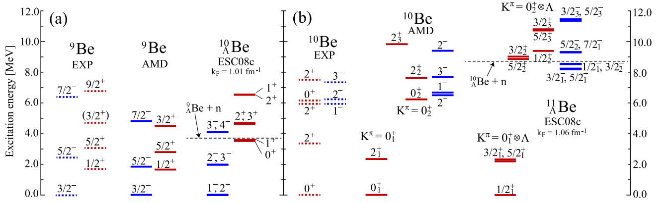
FIG. 1: (Color online) (a) Calculated excitation spectra of {}^9\text{Be} and {}^{10}_{\Lambda}\text{Be} . For the comparison, observed spectrum of {}^9\text{Be} [49] is also presented. Dashed line shows the experimental lowest threshold of {}^9_{\Lambda}\text{Be} + n in {}^{10}_{\Lambda}\text{Be} . (b) Same as (a) but for {}^{10}\text{Be} and {}^{11}_{\Lambda}\text{Be} . In {}^{11}_{\Lambda}\text{Be} , the energy of the lowest threshold {}^{10}_{\Lambda}\text{Be} + n is estimated from the observed data of {}^{10}_{\Lambda}\text{Be} [50] and the empirical value of B_{\Lambda} [51] due to the absence of the observation of {}^{11}_{\Lambda}\text{Be} .
