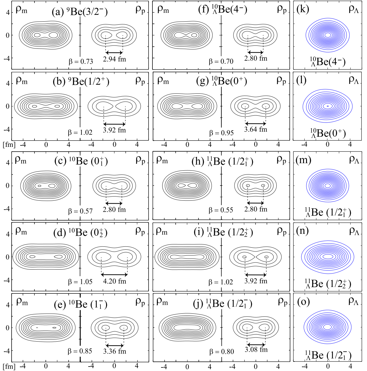
FIG. 2: (Color online) (a) - (e): Nuclear ( \rho_m ) and proton ( \rho_p ) density distributions of the 3/2^- and 1/2^+ states in {}^9\text{Be} , and the 0_1^+ , 0_2^+ and 1^- in {}^{10}\text{Be} . Inter-cluster distance between 2\alpha estimated by the peaks of the proton density is also displayed in each state. (f) - (j): Nuclear and proton density distributions of the hypernuclei corresponding to (a) - (e). (k) - (o): Density distributions of the \Lambda particle in each state in the hypernuclei.
