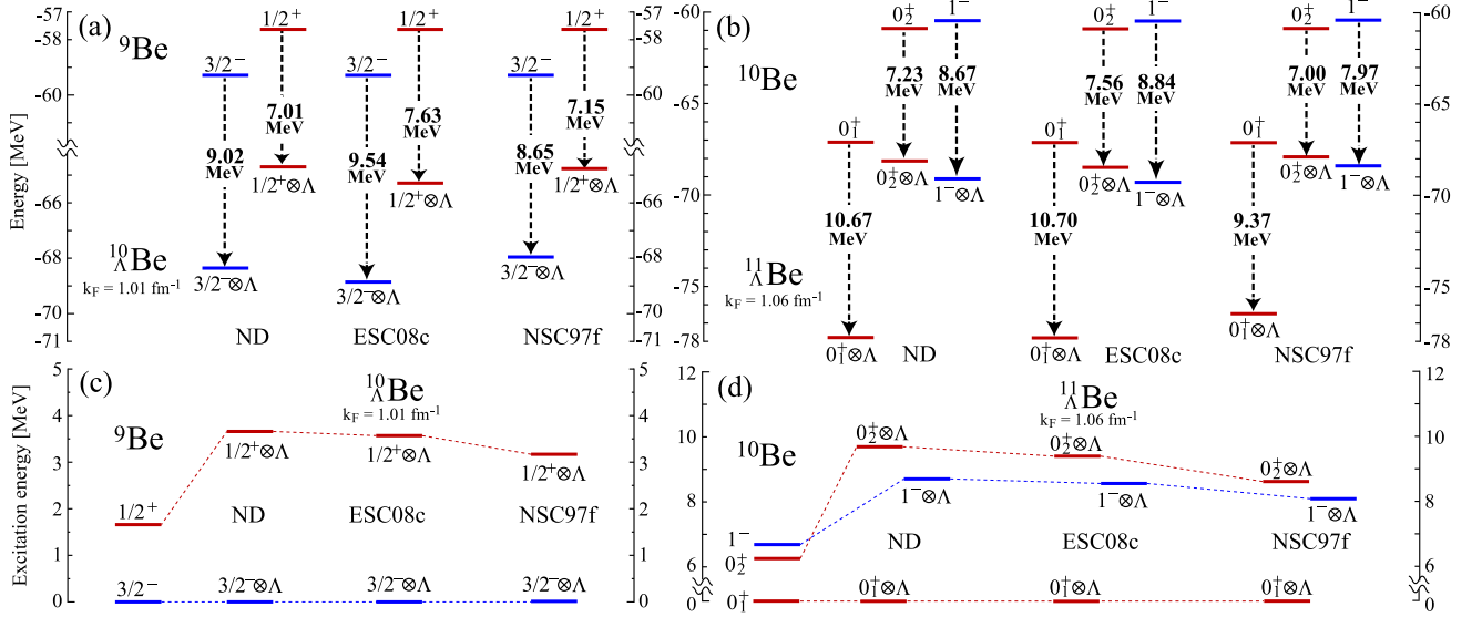
FIG. 4: (Color online) Comparison of B_\Lambda calculated with the ND, ESC08c and NSC97f interactions in (a) {}^{10}\Lambda\text{Be} and (b) {}^{11}\Lambda\text{Be} . (c) Comparison of the excitation energies of the {}^9\text{Be}(1/2^+) \otimes \Lambda states calculated with the ND, ESC08c and NSC97f interactions. (d) Same as (c), but for the {}^{10}\text{Be}(0_2^+) \otimes \Lambda and {}^{10}\text{Be}(1^-) \otimes \Lambda states in {}^{11}\Lambda\text{Be} . B_\Lambda in (a) and (b) and the excitation energies in (c) and (d) are calculated with the centroid energies of the doublets in each hypernucleus.
