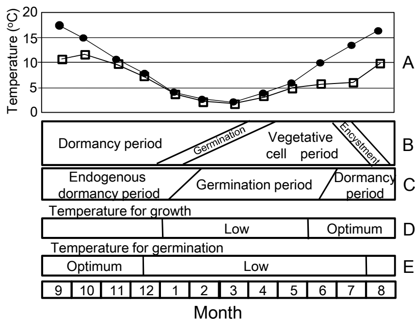
Fig. 34. Schematic diagrams of seasonal change in averaged water temperature (average of 0 – 30 m water column: ●, bottom: □) from 1982 to 2012 at Yakumo and Otoshibe stations (A), life cycle stage of A. tamarense (B), physiological phase of the cyst (C), temperature conditions for growth of the vegetative cells (D), and temperature conditions for the cyst germination (E).
