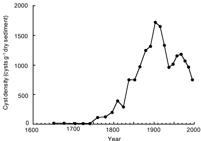
Fig. 40. Cyst density and estimated deposition time of A. tamarensis cysts at Stn. 5.
