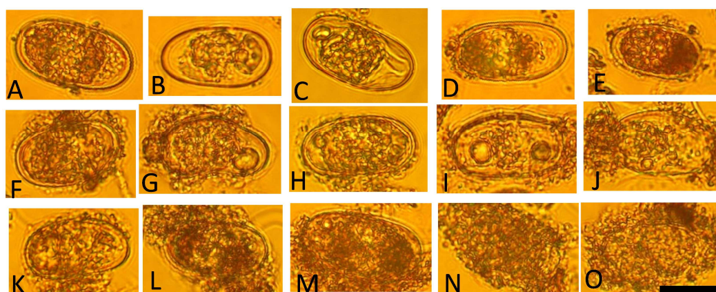
Fig. 48. The observation of A. tamarense -type cysts which collected from 0-1 cm bottom layer at 40 m-depth point off Date, Funka Bay in September, 2009. Special references were the thickness and the texture of cyst wall. A-D; textures of cyst wall were smooth with no substance (type 1 in Table 9), E-O; textures of cyst wall were smooth with many substances (type 2 in Table 9). Scale bar is 20 \mu m.
