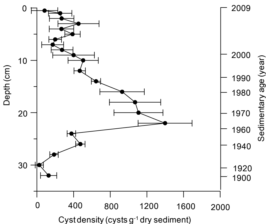
Fig. 43. Vertical distribution of A. tamarense -like cysts at Stn. A in Funka Bay. Plot indicates the average of triplicate counts (closed circle) and error bars indicate the standard deviations.
