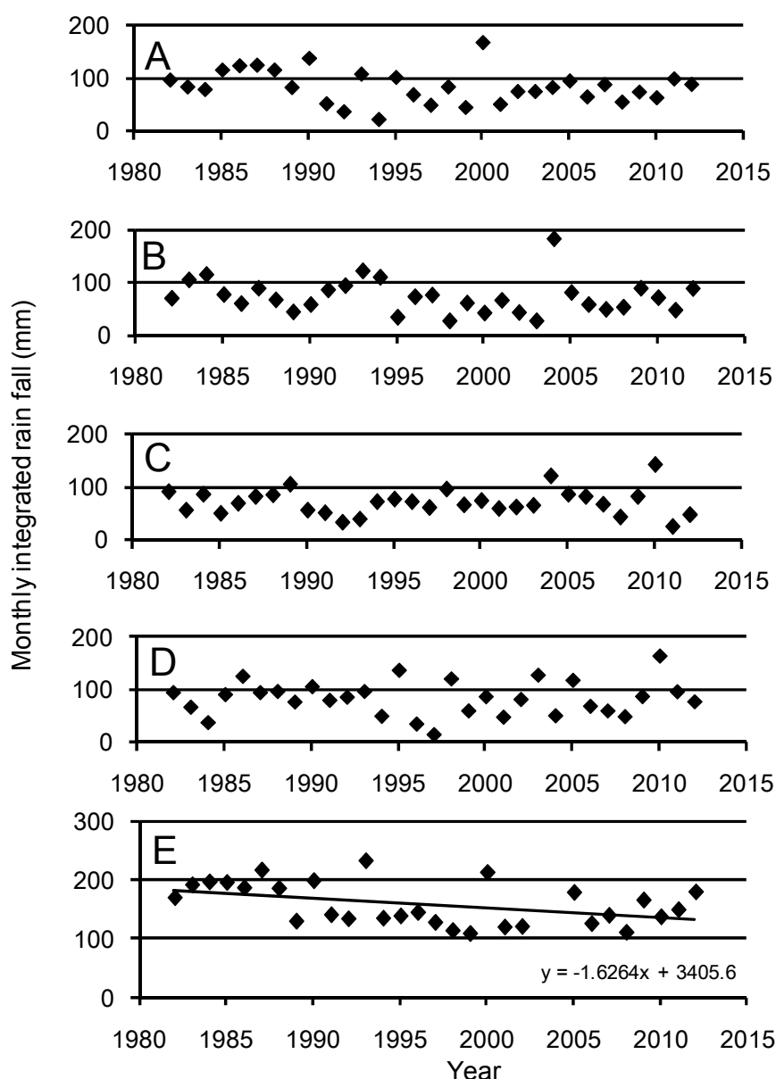
Fig. 51. Long-term fluctuations of monthly integrated rain fall (mm) recorded at AMeDAS Yakumo Station from 1982 to 2012. A: January, B: February, C: March, D: April, E: January and February, neglected maximum (2003) and minimum (2002) data. The negative linear regression was significant ( n=29 , r=0.422 , p<0.05 ).
