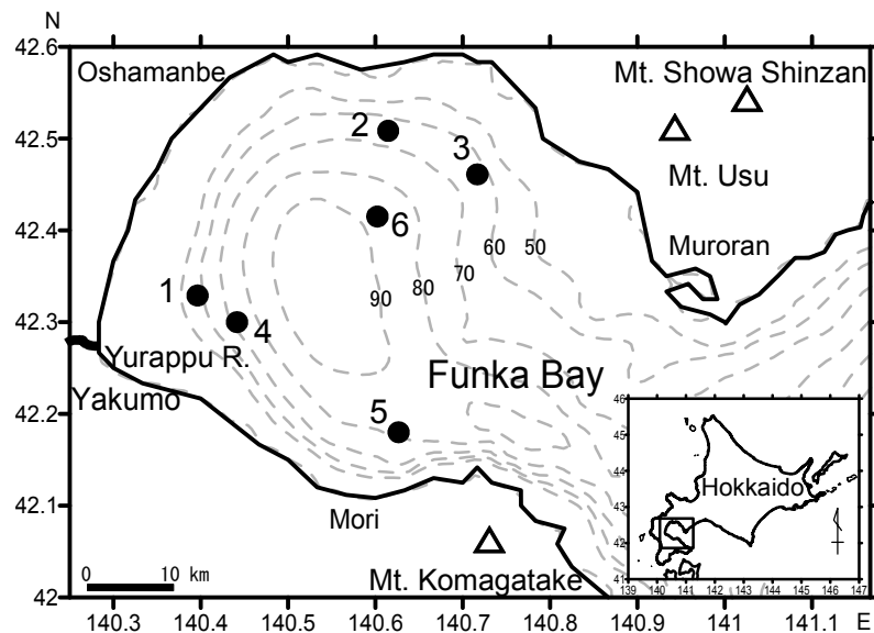
Fig. 35. Location of the sampling stations in Funka Bay (●). Dotted lines indicate bottom depth (m).
