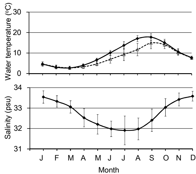
Fig. 6. Monthly averaged water temperature of water column (upper panel, \blacklozenge ), bottom water temperature (upper panel, \triangle ), and salinity of water column (lower panel) collected at seven different depths from 1981 to 2012 in coastal area of western Funka Bay (Otoshibe station: 1981-1992, Yakumo station: 1993-2012). Vertical bars indicate the standard deviations.
