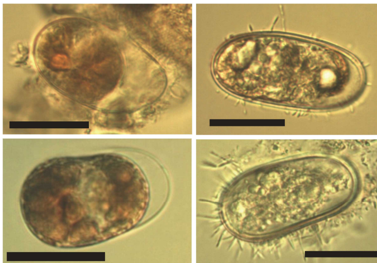
Fig. 47. A. tamarense cysts from surface sediment (0 to 0.5 cm depth, left top: cyst wall is thin with many substance, left bottom: cyst wall is thin with no substance) and deep sediment (30 to 32 cm depth, right top: cyst wall is thick with hair like extension, right bottom: cyst wall is thick with hair like extension and many substance). Scale bars are 20 \mu m.
