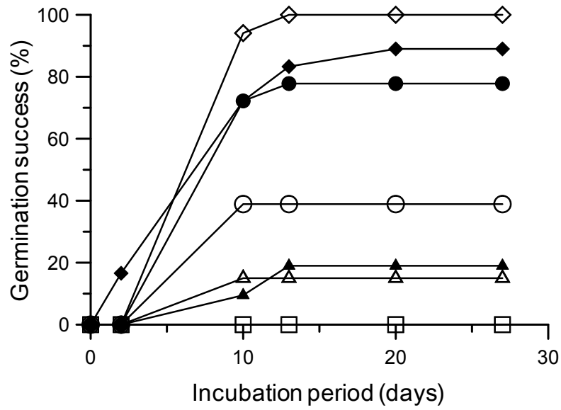
Fig. 44. Integrated germination success (%) of A. tamarensis cysts from seven depth layers (◆: 0-0.5 cm, ◇: 1-2 cm, ●: 5-6 cm, ○: 12-14 cm, △: 20-22 cm, ▲: 28-30 cm, □: 30-32 cm) of sediments incubated at 10°C under 100 \mu\text{mol photons m}^{-2} \text{s}^{-1} using cool fluorescent light with a 14-h light : 10-h dark photo-cycle.
