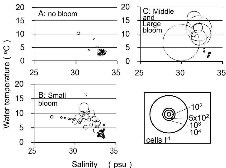
Fig. 9. T-S-P diagrams. Solid circle means cell density of A. tamarensis at the first detection. Dotted circle means cell density at maximum cell density of A. tamarensis bloom. A: the cases of no bloom years (maximum cell densities were \leq 100 ), B: the cases of small bloom years (maximum cell densities were 100 < \leq 1000 ), C: the cases of middle and large bloom years (maximum cell densities were > 1000 cells L^{-1} ).
