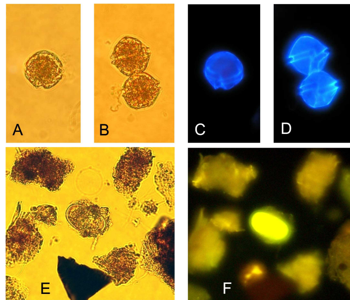
Fig. 1. Alexandrium tamarense , A, B; light micrograph of the vegetative cells under normal light (A; single cell, B; two cell chain, C, D; epifluorescence micrograph of the vegetative cells stained with calcofluor white observed under UV excitation (C; single cell, D; two cell chain), E; light micrograph of the cyst under normal light, F; epifluorescence micrograph of the cyst stained with primulin observed under blue excitation.
