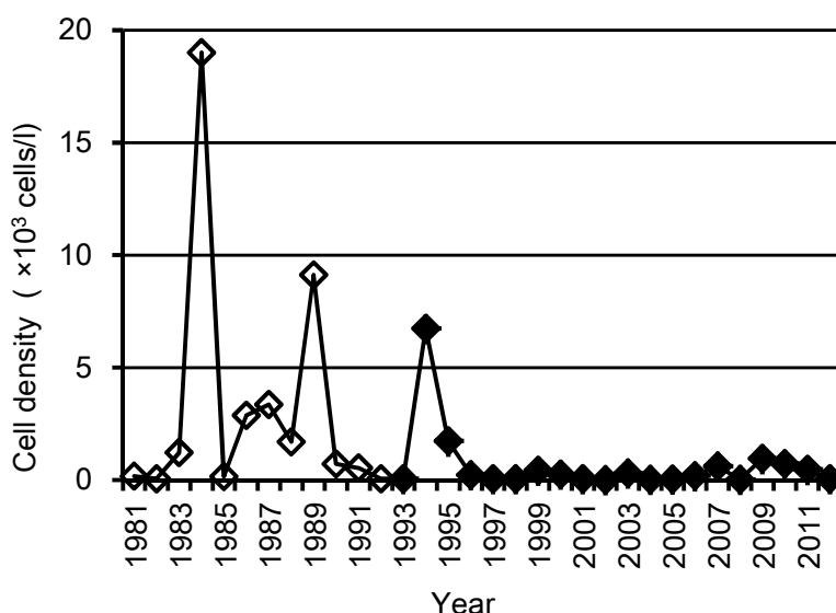
Fig. 4. The variation in maximum cell densities of A. tamarensis blooms from 1981 to 2012 at Otoshibe station (◇1981-1992) and Yakumo station (◆1993-2012) in coastal area of western Funka Bay.
