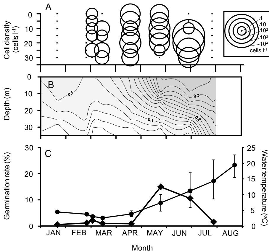
Fig. 30. Monitoring data (Seasonal change in cell densities of A. tamarensis at Yakumo station in 1994: A) , estimated growth rates (divisions day -1 ) using water temperature and light intensity from the results of the culture experiments (B) , germination rates of the cysts calculated using the bottom water temperature (◆, % month -1 ; C) and water temperature (●, average in the water column, vertical bars indicate maximum and minimum: C).
