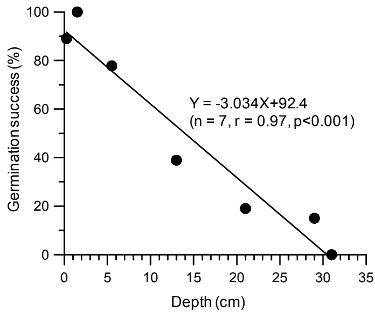
Fig. 45. Correlation between sediment depth (cm) and germination success (%) of A. tamarensis cysts.
