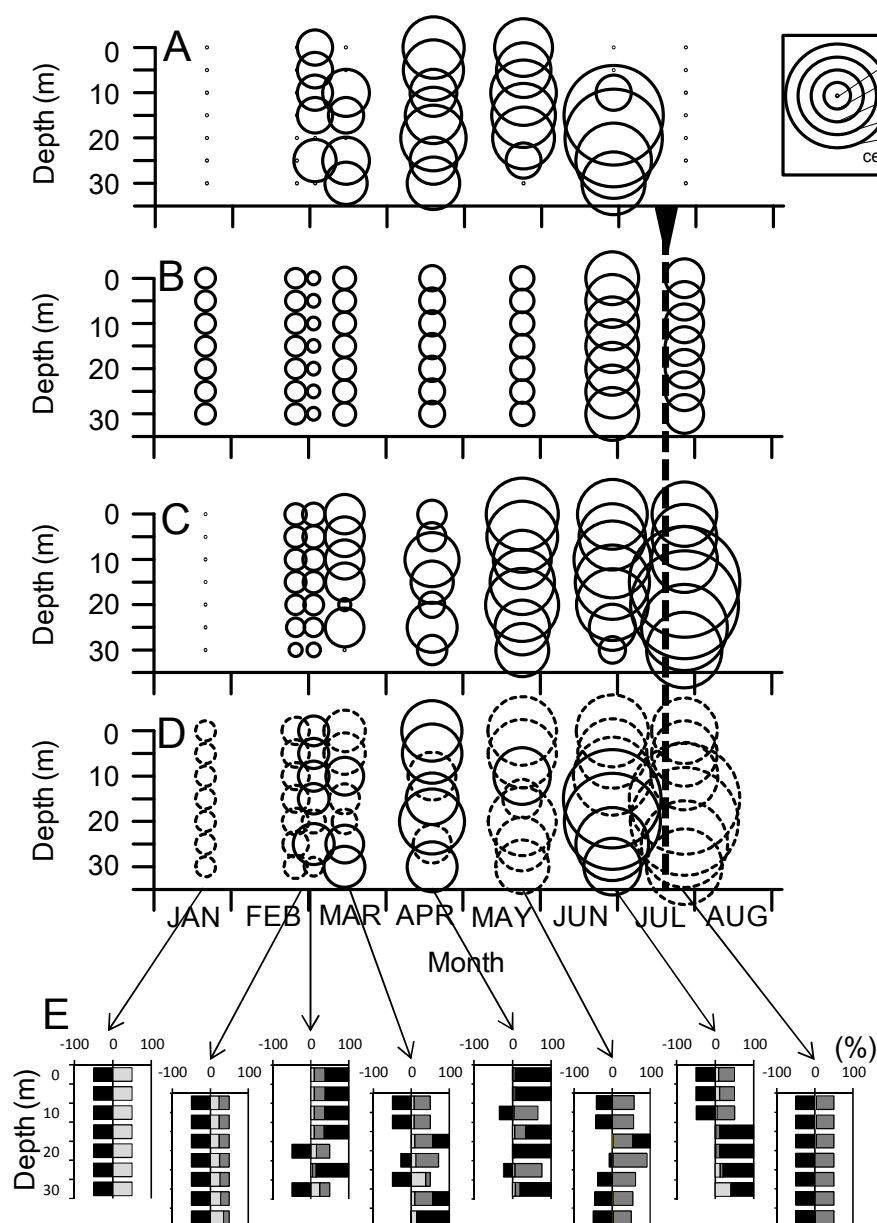
Fig. 33. The observed number of vegetative cells (A), estimated vegetative cell number inoculated from cyst germination (B), the estimated vegetative cell number by growth (C), and the estimated vegetative cell number fluctuated by the other factors (D), in 1994. Solid circles and dotted circles were increased cell numbers and decreased cell numbers, respectively. Composition of cyst germination (white), vegetative cell division (gray) and the others (black) in observed vegetative cells numbers (E). Vertical bold broken line indicate the timing when the average water temperature exceeded 14°C which is known as the upper limit of active growth of A. tamarensis in Funka Bay (Nishihama et al. 1980, Shimada 2000).
