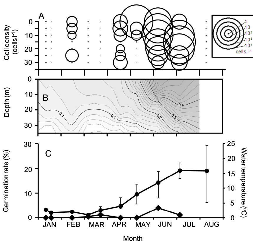
Fig. 28. Monitoring data (Seasonal change in cell densities of A. tamarensis at Otoshibe station in 1984: A), estimated growth rates (divisions day -1 ) using water temperature and light intensity from the results of the culture experiments (B), germination rates of the cysts calculated using the bottom water temperature (♦, % month -1 ; C) and water temperature (●, average in the water column, vertical bars indicate maximum and minimum: C).
