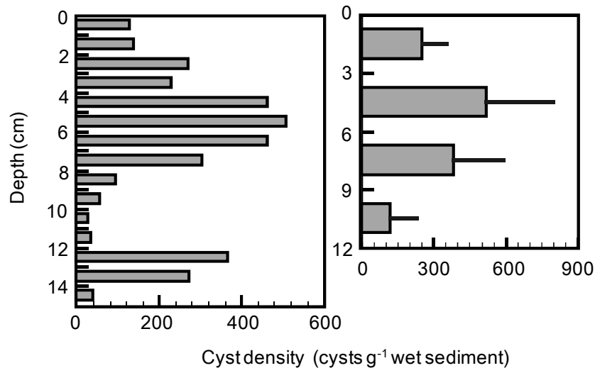
Fig. 22. Vertical profiles of A. tamarensis cyst density at Yakumo station. Left: the cyst density at every 1 cm depth layer from 0 to 15 cm sediment core collected in July, 1997. Right: the average cyst density at every 3 cm depth layer from 0 to 12 cm sediment core collected monthly from April, 1996 to March, 1997. Horizontal bars indicate the standard deviation (n = 3).
