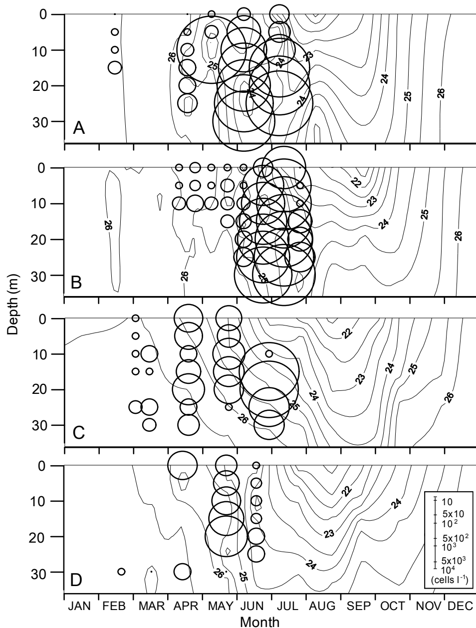
Fig. 10. Seasonal fluctuations of A. tamarense blooms with contour of sigma-t in large bloom years (maximum cell density > 5000 cells L^{-1} ): 1984 (A), 1989 (B), 1994 (C), and small bloom year ( 100 < \text{maximum cell density} \leq 1000 cells L^{-1} ): 2009 (D).
