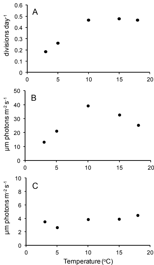
Fig. 17. Correlations between temperature and maximum growth rates ( \mu_m : A), half saturation constants ( K_s : B), threshold values of irradiance ( I_0 : C) of A. tamarensis isolated from Funka Bay obtained with the culture experiments under different light intensities at different temperatures.
