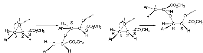
Scheme 1. Head-to-tail growth with inversion (left) and retention (right) of C(2) configuration in MCDMPO polymerization.
