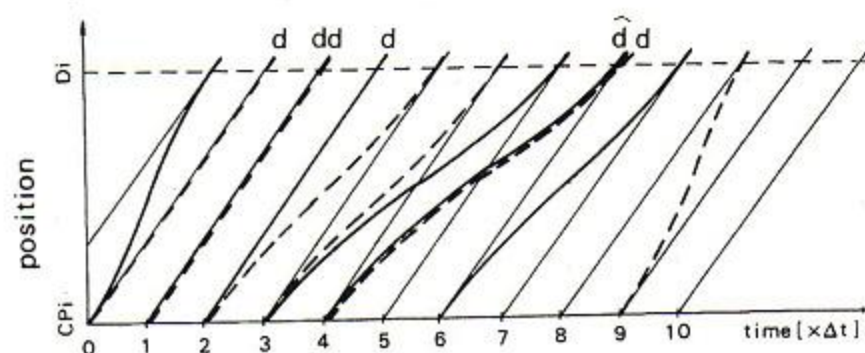
Fig. 8. Trajectories of the vehicles.
