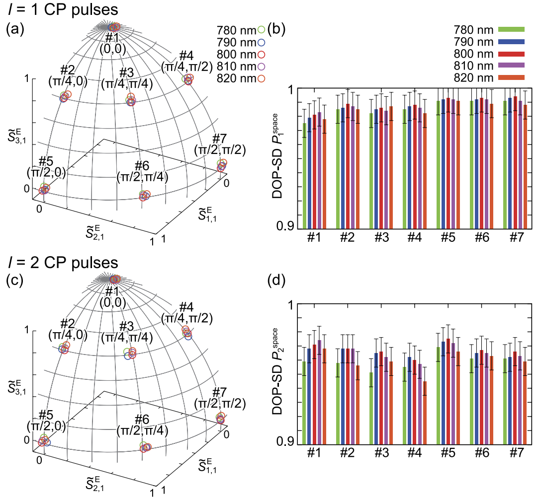
Figure 3. Spectrally-resolved characterization results for l=1 (a,b) and l=2 (c,d) CP pulses. The seven CP pulse states are realized in every azimuthal index l . (a,c) The values of normalized ESPs ( \tilde{S}_{1,l}^E , \tilde{S}_{2,l}^E , \tilde{S}_{3,l}^E ) for l=1 and l=2 CP pulse states plotted on the extended Poincaré sphere, respectively. (b,d) DOP-SD \mathcal{P}_l^{\text{space}} of l=1 and l=2 CP pulse states corresponding to (a,c), respectively.
