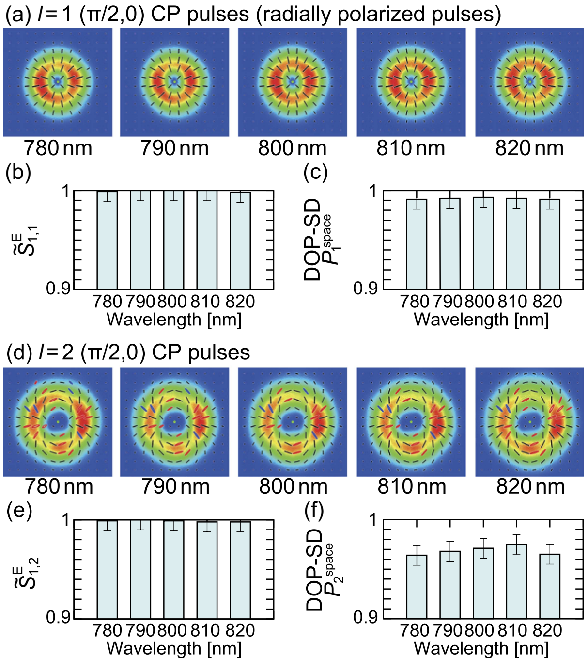
Figure 2. Characterization results of l = 1 (a–c) and l = 2 (d–f) ( \pi/2, 0 ) CP broadband pulses. (a,d) spectrally-resolved polarization distribution of generated l = 1 and l = 2 CP pulses, respectively. These polarization distributions are colored under the following rule: red, left-handed elliptical polarization; blue, right-handed elliptical polarization; black, linear polarization. The green points at the center of images represent the origins (x, y) = (0, 0) . (b,c) characterization results of \tilde{S}_{1,1}^E and \mathcal{P}_{1,1}^{space} for l = 1 ( \pi/2, 0 ) CP pulses (or radially polarized pulses), respectively. (e,f) characterization results of \tilde{S}_{1,2}^E and \mathcal{P}_{2,2}^{space} for l = 2 ( \pi/2, 0 ) CP pulses, respectively.
