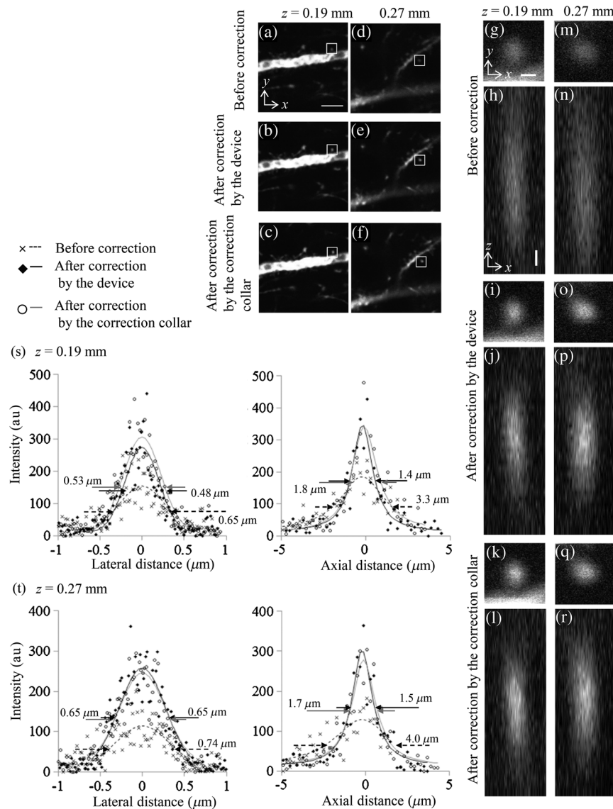
Fig. 6 Images of the biospecimen in two-photon excitation microscopy illuminated with 950-nm-wave-length laser light. Lateral images (a) before and (b) after correction by the device at z = 0.19 mm, when the correction collar of the objective lens was adjusted to obtain the best performance beneath the cover glass surface ( z = 0 mm). (c) Lateral image at z = 0.19 mm, when the correction collar of the objective lens was adjusted to obtain the best performance at z = 0.19 mm. Lateral images (d) before and (e) after correction by the device at z = 0.27 mm, when the correction collar of the objective lens was adjusted to obtain the best performance at z = 0 mm. (f) Lateral image at z = 0.27 mm, when the correction collar of the objective lens was adjusted to obtain the best performance at z = 0.27 mm. The images in (g-r) were obtained in the area indicated by a rectangle in (a-f). (g) Lateral and (h) axial images before and after correction by (i, j) the device and (k, l) the correction collar at z = 0.19 mm. Lateral and axial images (m, n) before and after correction by (o, p) the device and (q, r) the correction collar at z = 0.27 mm. (s, t) Intensity profiles across the center of the intensity distribution along the x - and the z -axes at each depth z . The scale bars denote 5\ \mu\text{m} in (a) and 0.5\ \mu\text{m} in (g) and (h).
