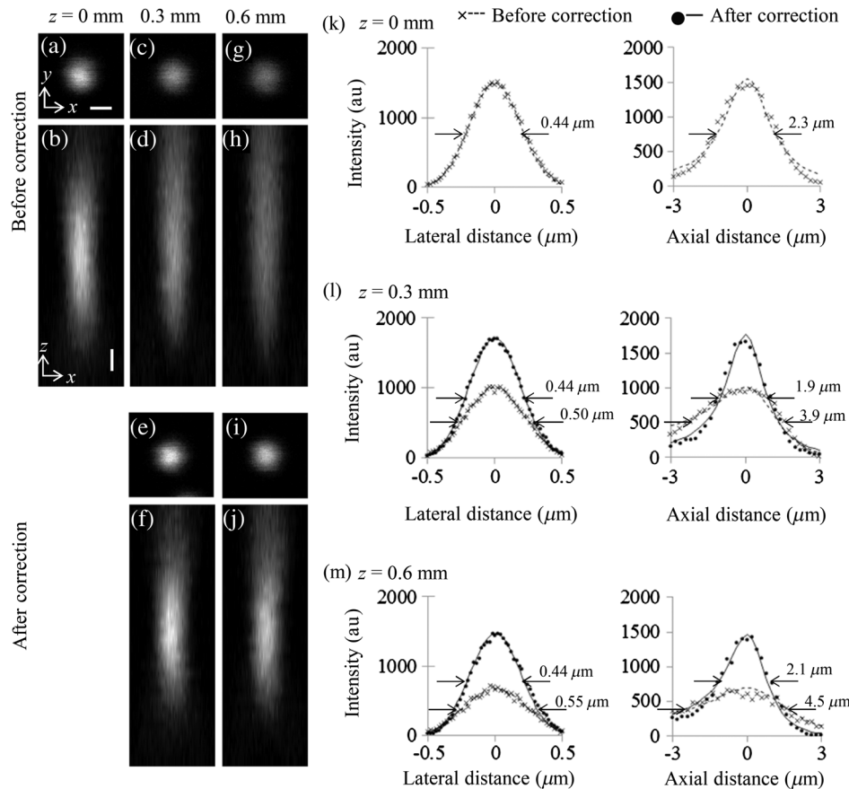
Fig. 5 Images of fluorescent beads in two-photon excitation microscopy illuminated with 950-nm-wave-length laser light. The correction collar of the objective lens was adjusted to obtain the best performance beneath the cover glass surface ( z = 0 mm). (a) Lateral and (b) axial images at z = 0 mm. Lateral and axial images (c, d) before and (e, f) after correction at z = 0.3 mm. Lateral and axial images (g, h) before and (i, j) after correction at z = 0.6 mm. (k-m) Intensity profiles across the center of the intensity distribution along the x - and the z -axes at each depth z . The data points in (k-m) are the mean values of several beads. The scale bars represent 0.5 \mu\text{m} .
