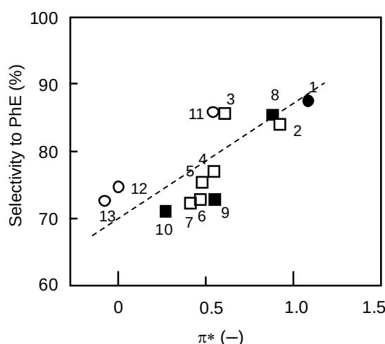
Fig. 5. The selectivity to PhE over Rh/Al 2 O 3 vs. the \pi^* value of the solvent. Numbers given correspond to the different solvents in Fig. 1.
