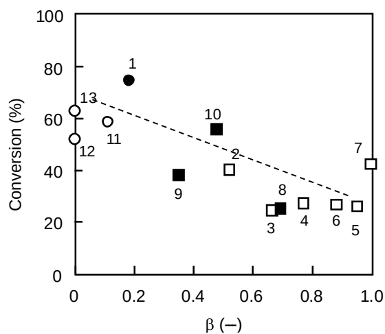
Fig. 3. The conversion over Rh/Al 2 O 3 vs. the \beta value of the solvents. Numbers given correspond to the different solvents in Fig. 1.
