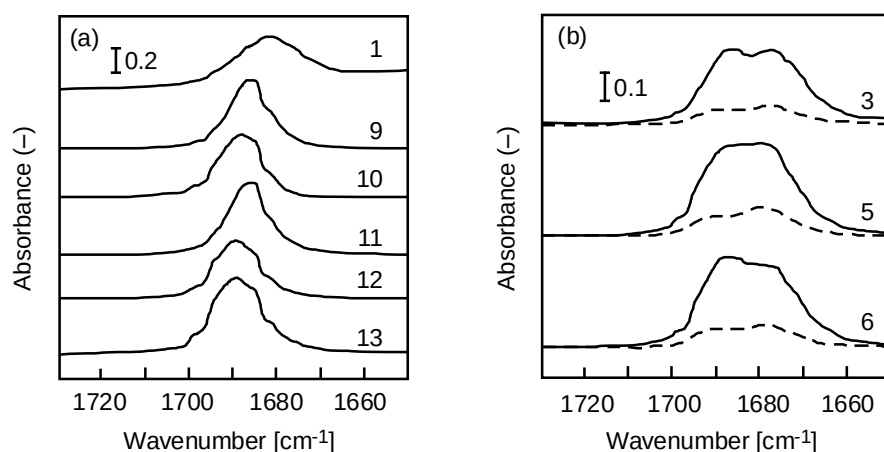
Fig. 4. ATR-FTIR spectra of AP in different solvents measured under ambient conditions. For (a) AP/solvent = 2/5 (volume); (b) AP/solvent = 2/5 (solid lines), 1/15 (broken lines). Numbers given correspond to those solvents in Fig. 1.
