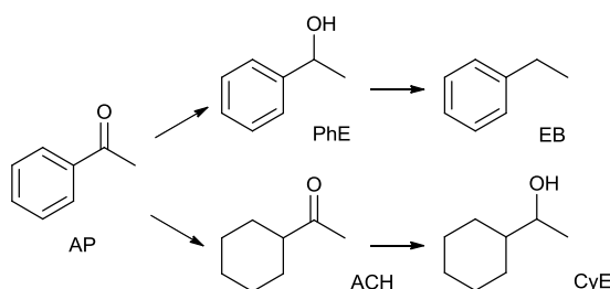
Scheme 1. Hydrogenation of acetophenone (AP). PhE: phenylethanol, ACH: acetylcyclohexane, EB: ethylbenzene, CyE: cyclohexylethanol
