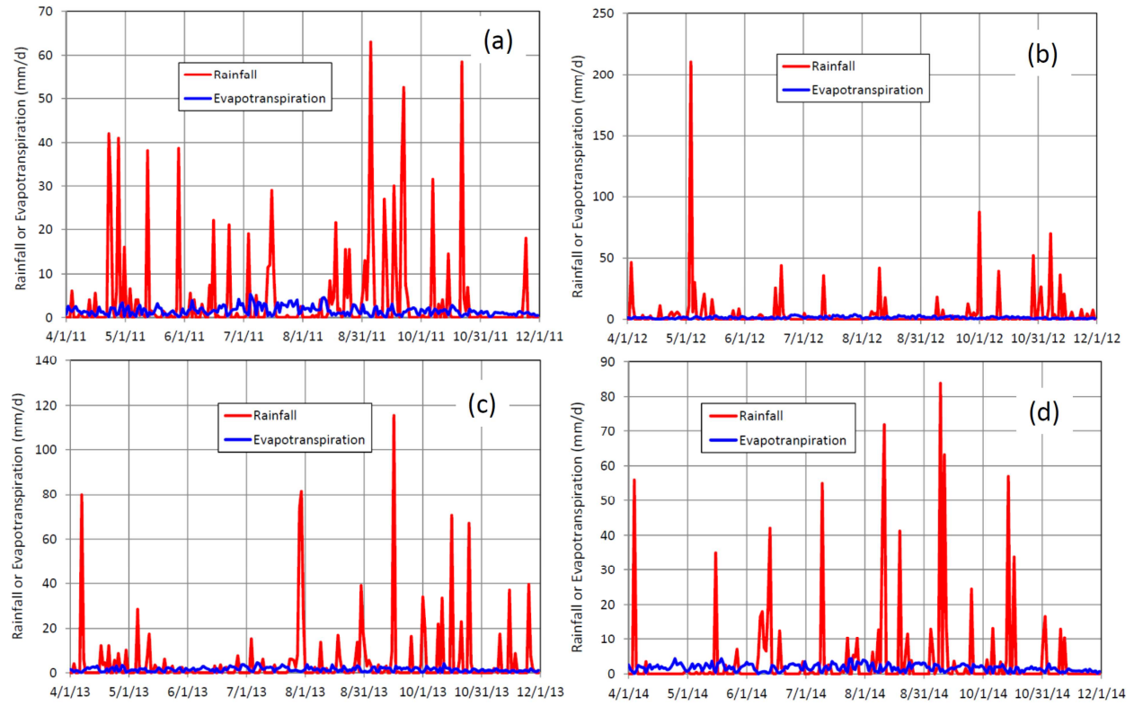
Fig. 3.2 Calculated evapotranspiration and observed rainfall in (a) 2011, (b) 2012, (c) 2013 and (d) 2014
