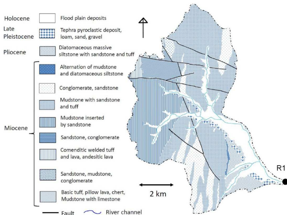
Fig. 2.2 Geology of the catchment upstream of site R1
