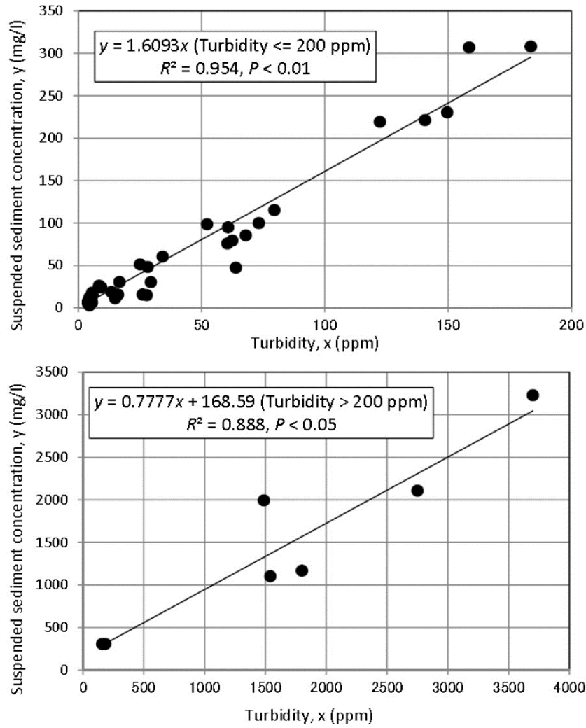
Fig. 2.3 Relationships between water turbidity (ppm) and suspended sediment concentration (SSC: mg/L), separated by turbidity of 200 ppm.
