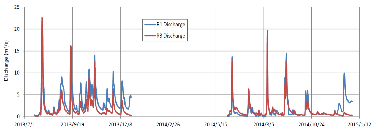
Fig. 5.1 Daily observed discharge at sites R1 and R3
