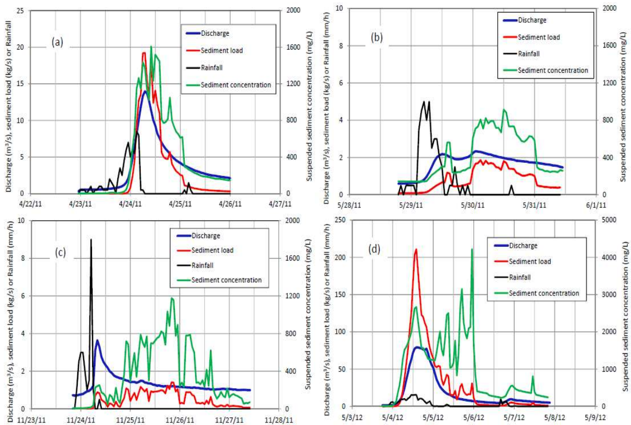
Fig. 2.5 Hourly time series of discharge, SSC and sediment load at site R1, and rainfall at site P for river runoff events with extra sediment supply. (a) no. 1, (b) no. 4, (c) no. 12 and (d) no. 13 in Table 2.
