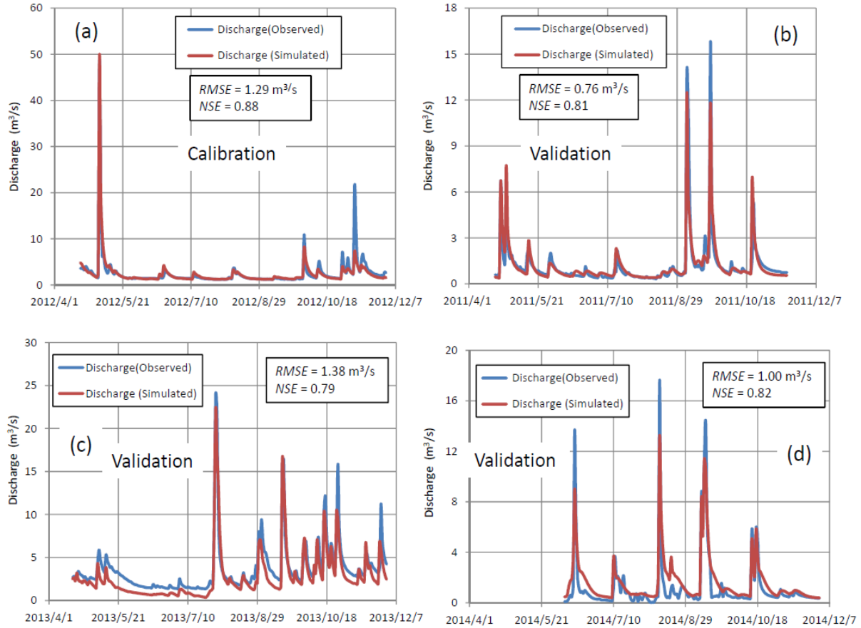
Fig. 4.3 Discharge simulation at site R1 (a) calibration in 2012, (b) validation in 2011, (c) validation in 2013, (d) validation in 2014.
