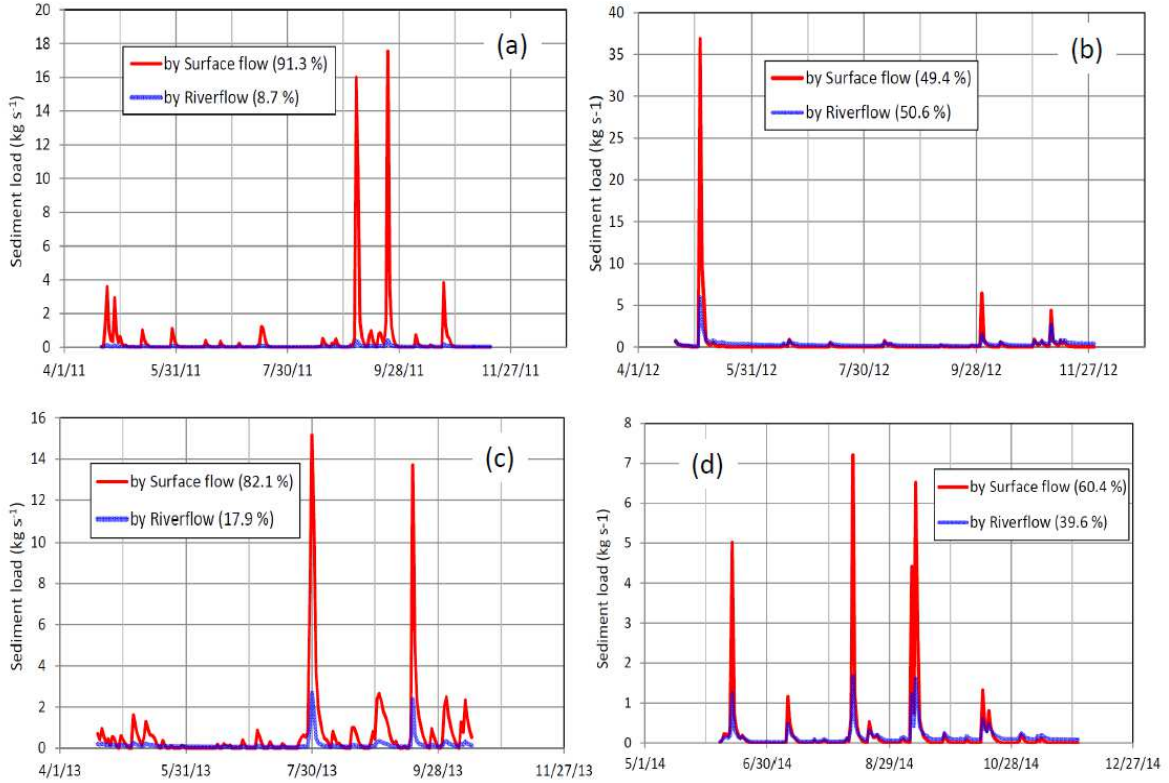
Fig. 3.6 Contribution of sediment transport by surface flow and river by the tank model for (a) 2011, (b) 2012, (c) 2013 and (d) 2014.
