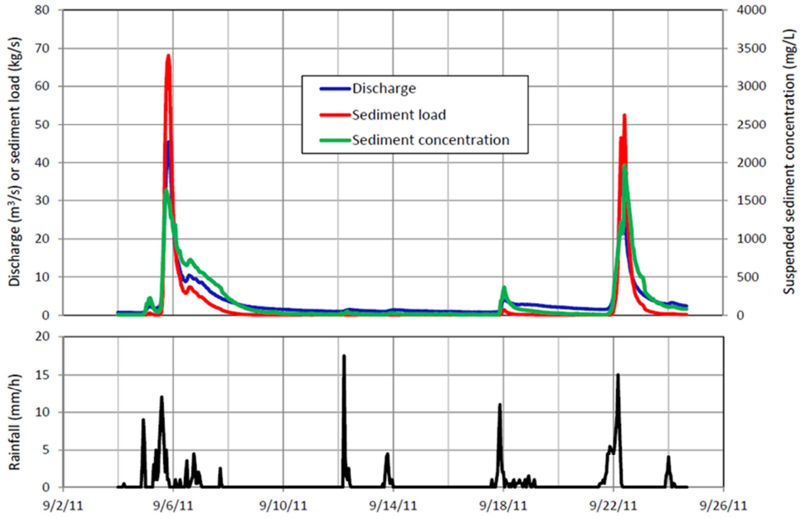
Fig. 2.6 Hourly time series of discharge, SSC and sediment load at site R1, and rainfall at site P for river runoff events without extra sediment supply.
