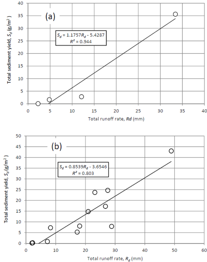
Fig. 5.5 Relations between total runoff rate R_d (mm) and total sediment yield S_d ( \text{g}/\text{m}^2 ) for rainfall runoff events with extra sediment supply (a) at site R1 (b) at site R3 in July 2013-2014.
