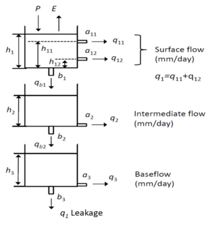
Fig. 3.1 Tank layout for the tank model
