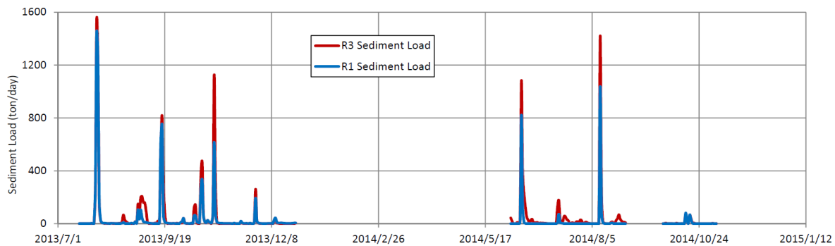
Fig. 5.2 Sediment load observed at site R1 and site R3
