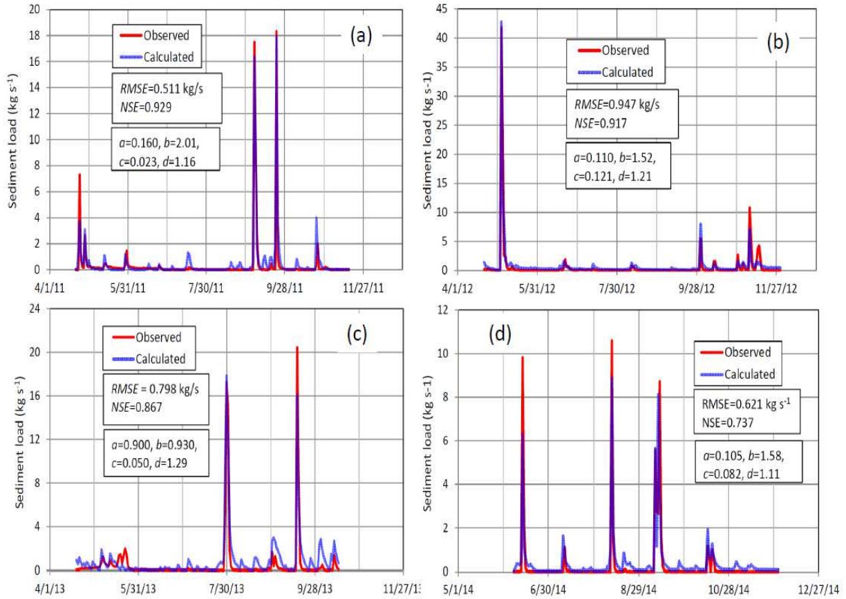
Fig. 3.5 Simulated results of sediment load by the coupling with power function (a) 2011, (b) 2012, (c) 2013 and (d) 2014.
