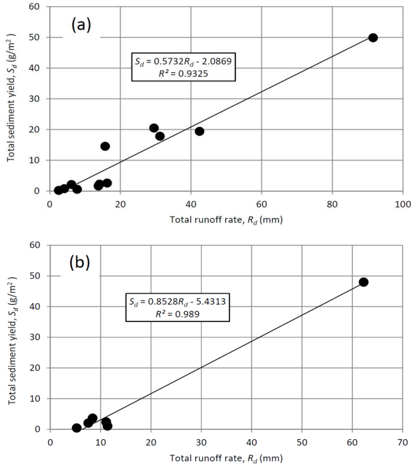
Fig. 5.6 Relations between total runoff rate R_d (mm) and total sediment yield S_d (g m -2 ) for rainfall runoff events without extra sediment supply (a) at site R1 (b) at site R3 in July 2013-2014.
