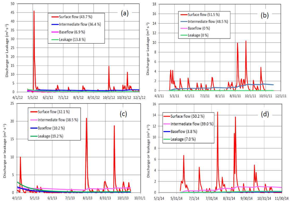
Fig. 3.4 Time series and occupation rate of flow components separated by the tank model for (a) 2012 and (b) 2011, (c) 2013, (d) 2014.
