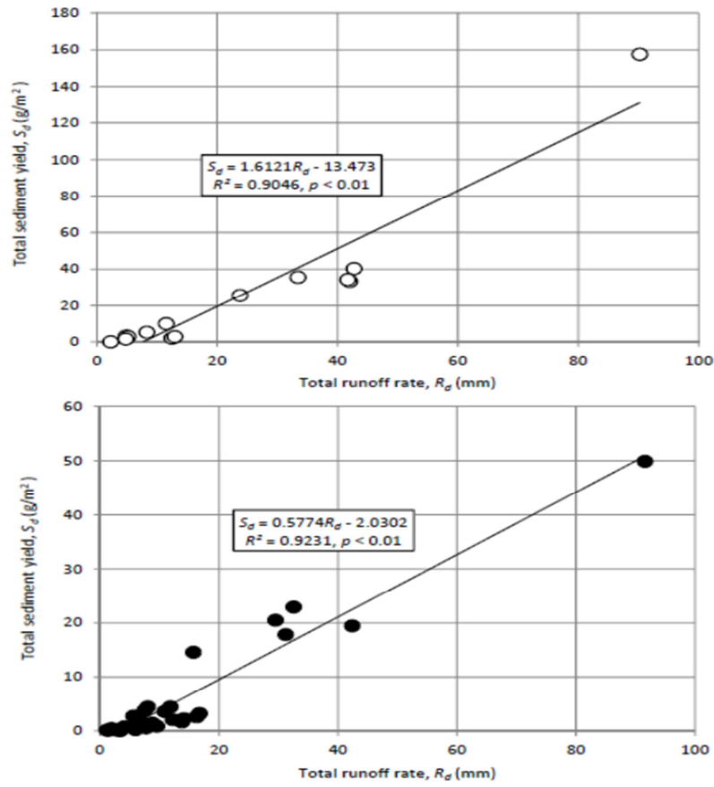
Fig. 2.7 Relations between total runoff rate R_d (mm) and total sediment yield S_d ( \text{g m}^{-2} ) for rainfall runoff events with (white circles) and without (black circles) extra sediment supply at site R1.
