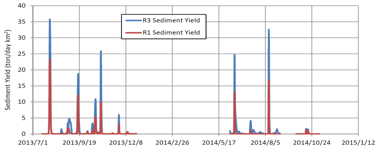
Fig. 5.3 Sediment yield at site R1 and site R3
