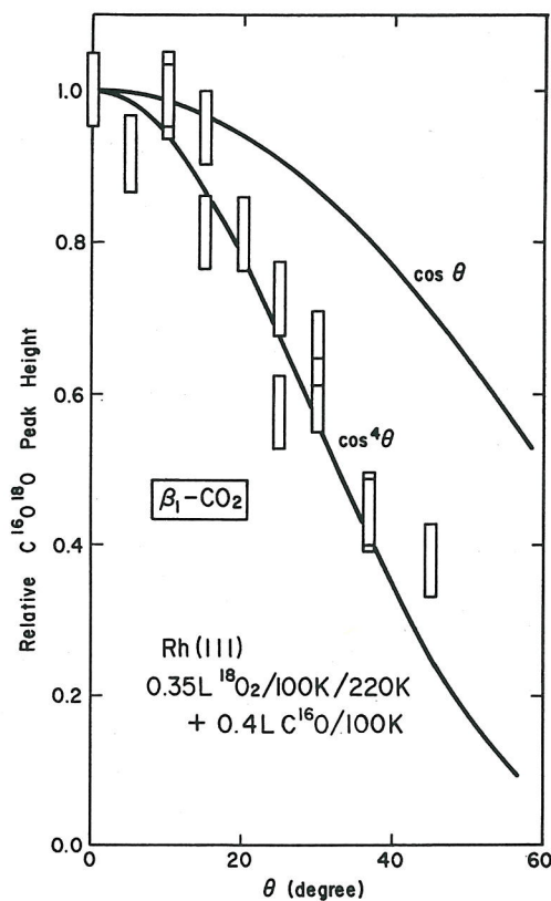
FIG. 12. Angular distribution of the β 1 -CO 2 formation.
