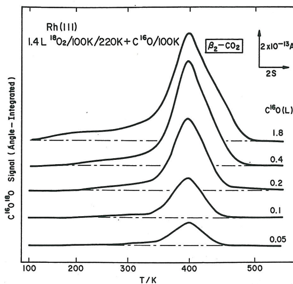
FIG. 7. \beta_2\text{-CO}_2 formation spectra on oxygen-saturated surfaces. The heating rate was 24 K/s.
