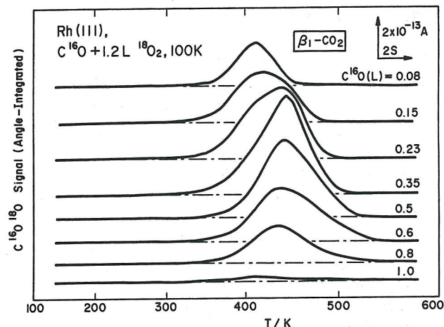
FIG. 2. Variation of \text{CO}_2 spectra with various CO preexposures. The surface was first exposed to CO and then to 1.2 L ^{18}\text{O}_2 at 100 K. The heating rate was 20 K/s.
