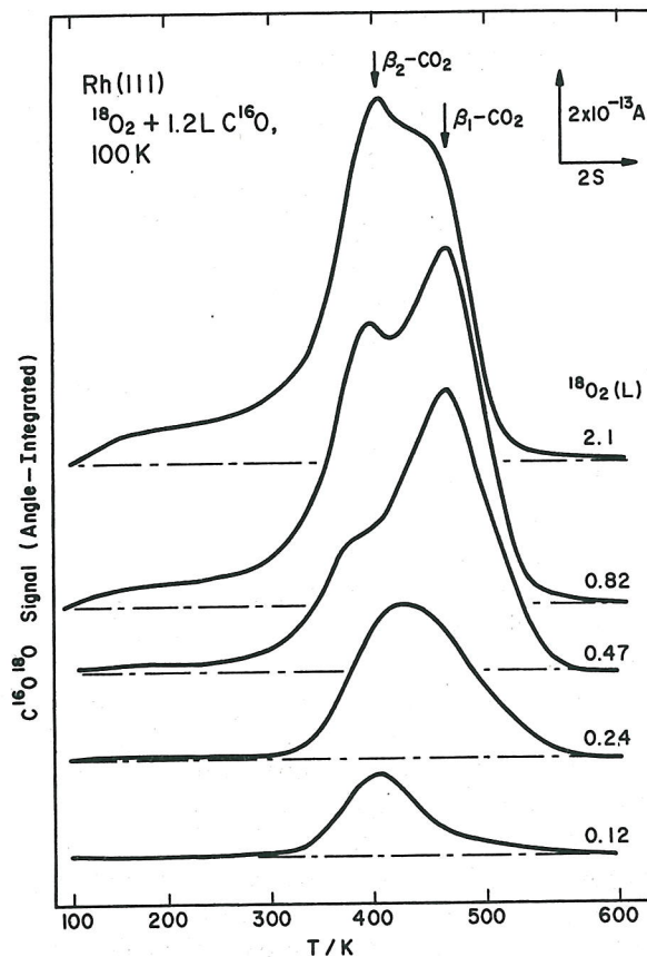
FIG. 3. \text{CO}_2 formation spectra with various amounts of ^{18}\text{O}_2 exposures followed by 1.2 L exposure of \text{C}^{16}\text{O} at 100 K. The heating rate was 35 K/s.
