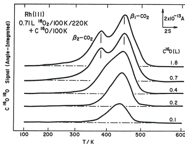
FIG. 6. \beta_1\text{-CO}_2 and \beta_2\text{-CO}_2 formation spectra at moderate \text{O}_2 exposures. The heating rate was 23 K/s.
