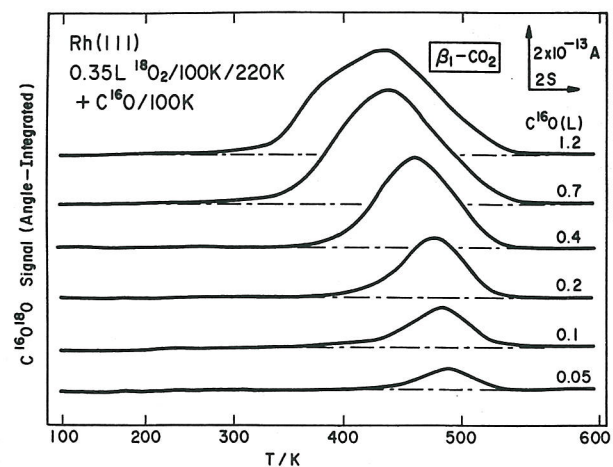
FIG. 5. \beta_1\text{-CO}_2 formation spectra at small \text{O}_2 exposures. The surface was exposed to 0.35 L ^{18}\text{O}_2 at 100 K and heated to 220 K. It was further exposed to various amounts of CO at 100 K. The heating rate was 22 K/s.
