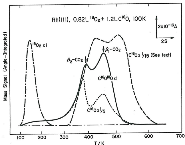
FIG. 1. Typical thermal desorption spectra of ^{18}\text{O}_2 , \text{C}^{16}\text{O} , and \text{C}^{16}\text{O}^{18}\text{O} when the surface was exposed to 0.82 L ^{18}\text{O}_2 and 1.2 L \text{C}^{16}\text{O} at 100 K. The dashed curve of CO shows the desorption from a CO-saturated surface without \text{O}_2 exposure. The heating rate was 33 K/s.
