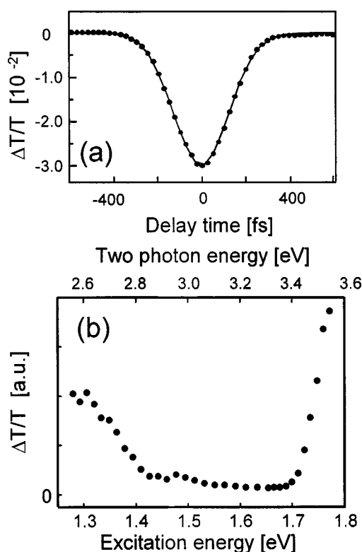
FIG. 3. (a) Decrease in TPA-induced transmission at 1.5 eV excitation. The solid line indicates a Gaussian fit. (b) TPA spectrum obtained from changes in transmission at various excitation energies ( E_{ex} ). The upper axis corresponds to 2 \times E_{ex} .
