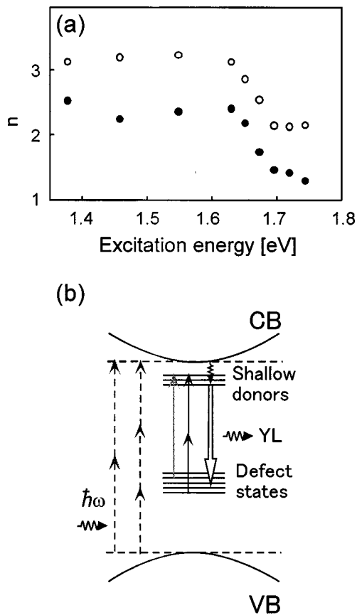
FIG. 2. (a) Excitation energy dependence of multiphoton PL. Closed and open circles correspond to YL and UV luminescence, respectively. (b) Schematic of the carrier transition processes observed in the YL band. Solid and gray arrows indicate excitation energy < E_g/2 and > E_g/2 , respectively.
