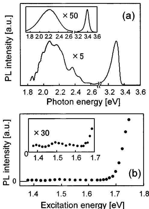
FIG. 1. (a) Multiphoton PL spectrum excited with 1.5 eV photons. Inset: PL excited by a He–Cd laser. The YL ranges from 1.8 to 2.6 eV. (b) Multiphoton PLE spectrum detected at 2.4 eV, corresponding to the higher energy side of the YL. Inset: Expanded view below E_g/2 .
