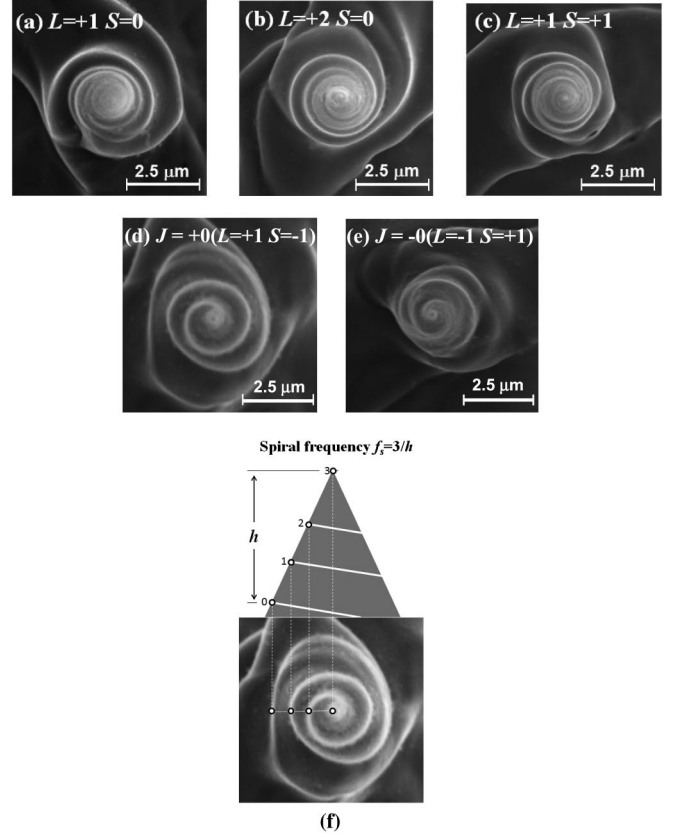
FIG. 2. Chiral nanoneedles fabricated by (a) linearly polarized first-order and (b) second-order optical vortices. (c) Chiral nanoneedle fabricated by circularly polarized first-order optical vortex with J = 2 . Chiral nanoneedles fabricated by circularly polarized optical vortices with a total angular momentum J = 0 : (d) L = 1 , S = -1 and (e) L = -1 , S = 1 . (f) Definition of the spiral frequency of the nanoneedles. The spiral frequency is defined as the number of spiral turns divided by h (distance between the tip and the bottom of the spiral structure in the chiral nanoneedle).
