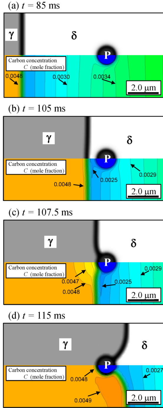
Fig. 3—Time changes of the phase-field and carbon concentration profiles around one particle. Particle radius, r , is 0.6\ \mu\text{m} and the length of y -direction, l , is 6.0\ \mu\text{m} . Initial carbon concentration of \delta phase, C_{\delta,0} , is 0.0045 (mole fraction). After step (d) the interface returned to planar shape as in step (a).
