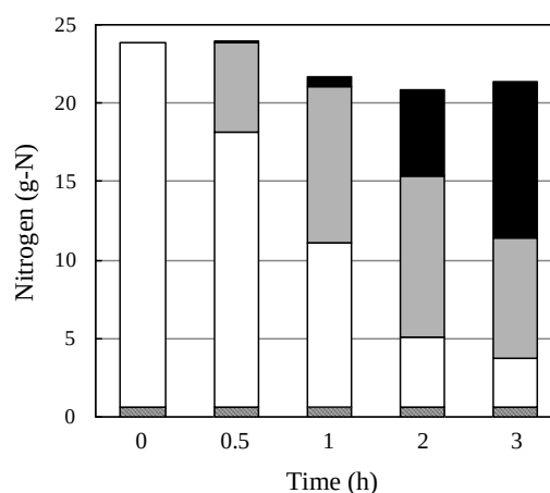
Fig. 5 Time courses of the amounts of nitrogen derived from urea (white), low molecular methylene urea (gray), methylene urea (black) and creatinine+NH 4 Cl (stripe) during methylene urea synthesis from treated synthetic urine.
