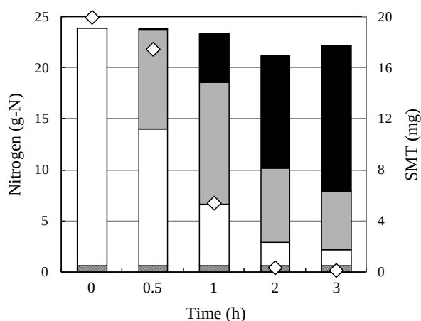
Fig. 3 Time courses of the amounts of nitrogen derived from urea (white), low molecular methylene urea (gray), methylene urea (black) and creatinine+NH 4 Cl (stripe) during methylene urea synthesis from synthetic urine. Diamond shows the amount of SMT contained in synthetic urine.
