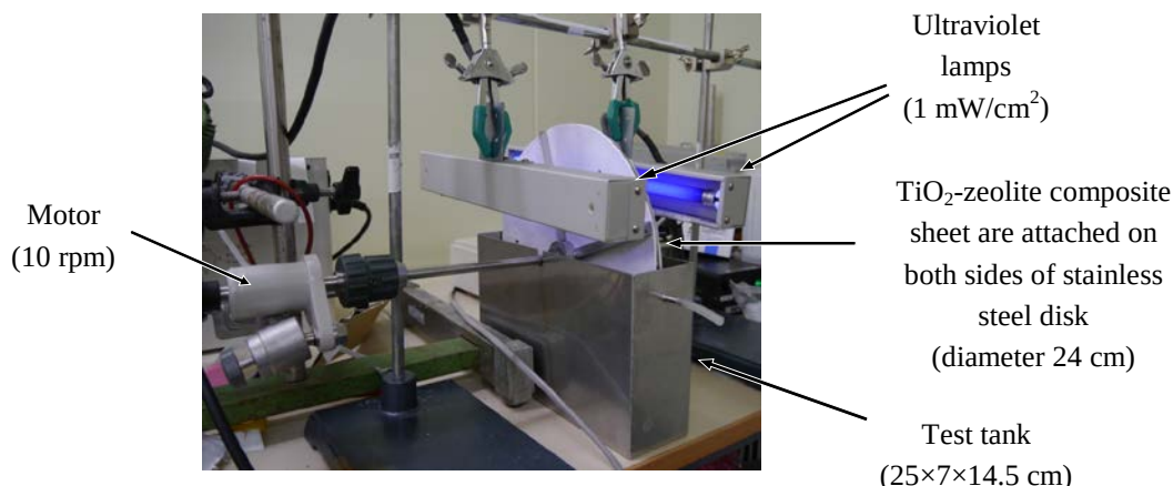
Fig. 1 Rotating advanced oxidation contactor
