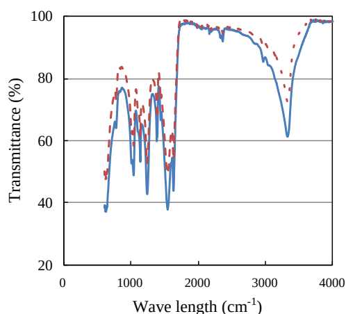
Fig. 2 IR spectra of precipitate obtained from synthetic urine (solid line) and urea solution (dash line).
