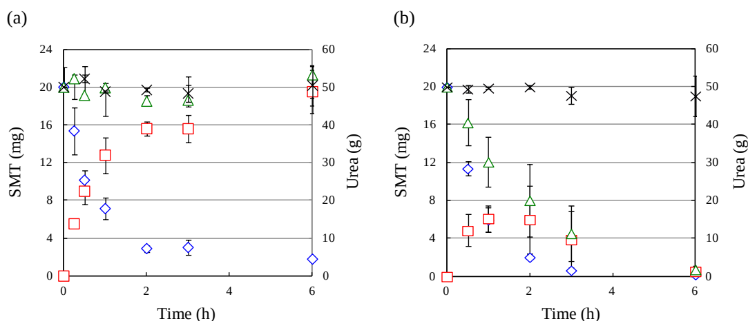
Fig. 4 Time courses of the amount of urea and SMT when treated by RAOC without (a) or with (b) UV irradiation: urea (crosses) and SMT (diamonds) in synthetic urine, SMT in TiO 2 -zeolite composite sheet (squares) and total system (triangles).
