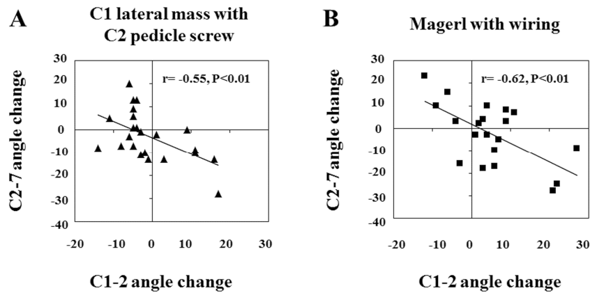
Fig 3 Correlation between the C1–C2 angle change and C2–C7 angle change. A: C1 lateral mass
