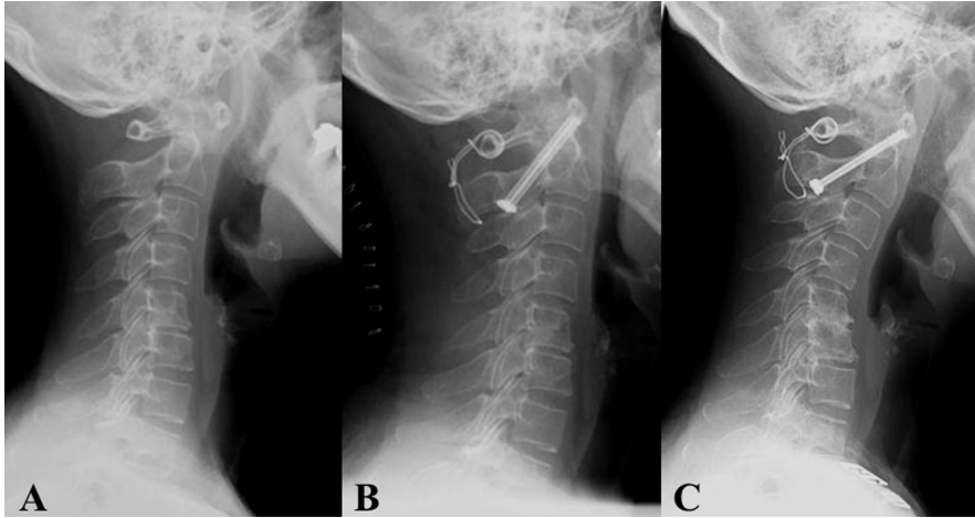
Fig 4 A 42-year-old rheumatoid arthritis woman with a preoperative C1–C2 angle of 27° ( A ). The C1–C2 angle after surgery was increased to 36° after the Magerl procedure combined with Gallie wiring technique ( B ). Increased kyphotic change in the C2–C7 angle was observed at 7 years follow-up ( C ).
