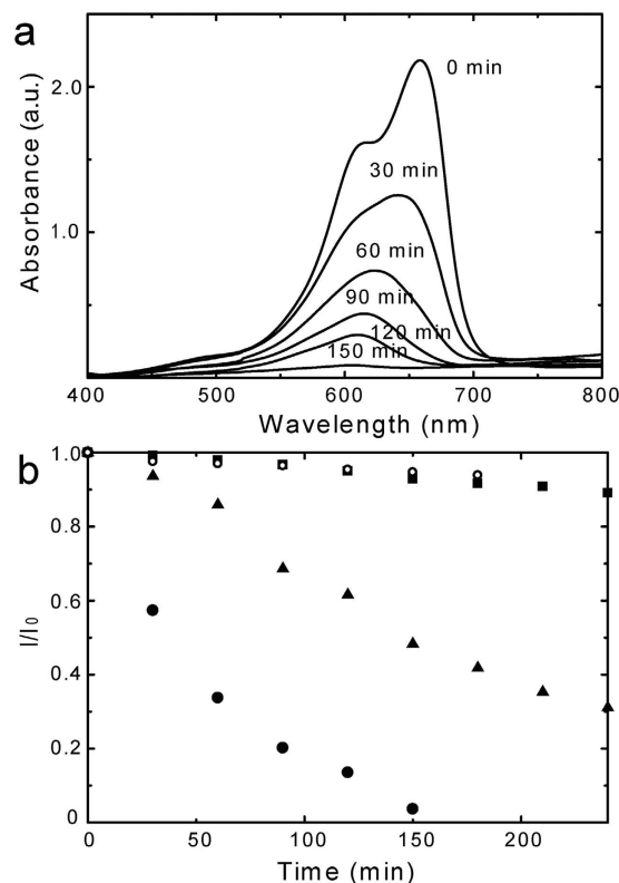
Figure 6. Photocatalytic activity of N-doped \text{TiO}_2 . (a) UV-visible spectroscopic changes of methylene blue solution over \text{TiO}_2 -(1), (b) chronological change of adoption intensity upon various photocatalysts under visible-light (>410 nm) irradiation: no catalyst (circle), \text{TiO}_2 -(1) (black dot), \text{TiO}_2 -(2) (black square) and \text{TiO}_2 -sg (black triangle).
