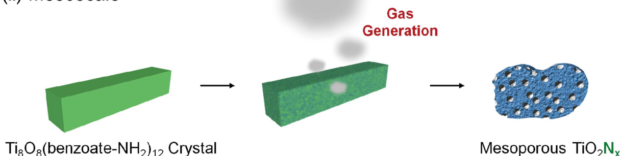
Figure 5. Schematic illustration of the reaction mechanism. Reaction scheme at (i) molecular scale and (ii) mesoscale: Coordination cluster of 1 is converted to mesoporous N-doped \text{TiO}_2 .
