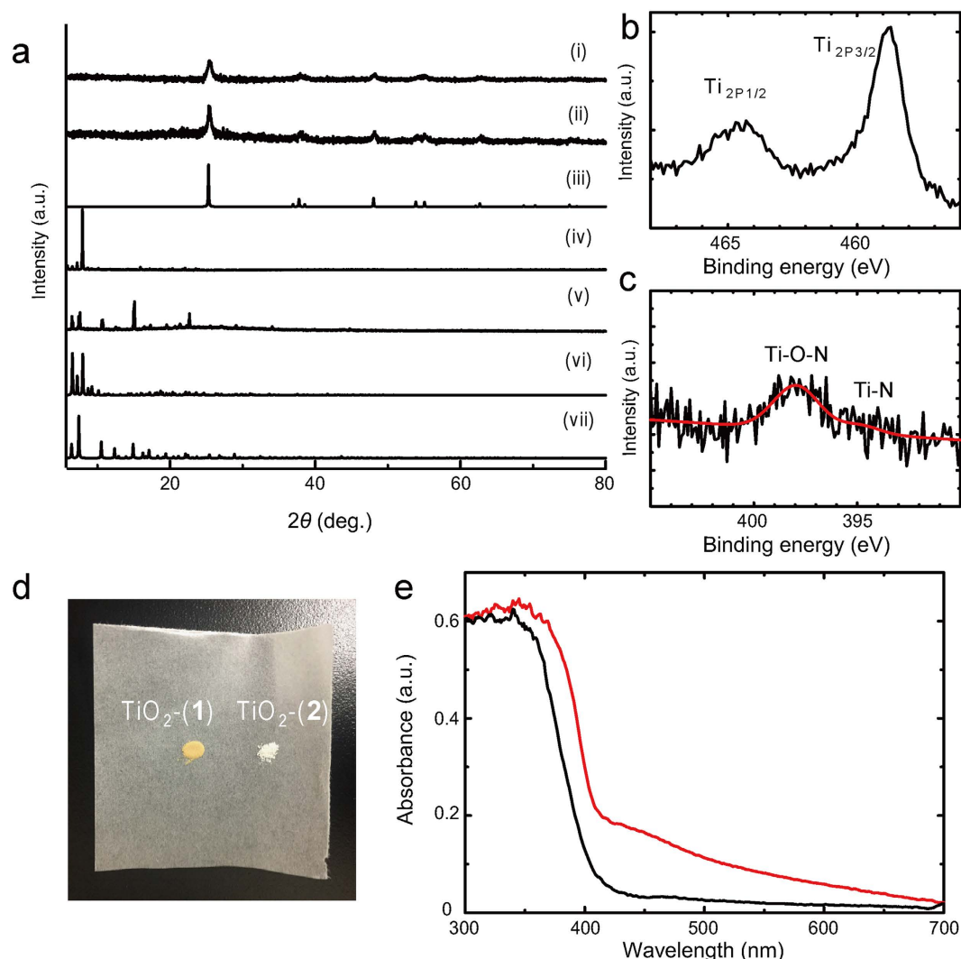
Figure 3. Spectroscopic characterization of TiO 2 -(1) and TiO 2 -(2). (a) PXRD of (i) TiO 2 -(1), (ii) TiO 2 -(2), (iii) Simulated TiO 2 , (iv) 1, (v) 2, (vi) simulated 1 and (vii) simulated 2. (b–c) XPS spectra of TiO 2 -(1) for Ti 2p and N 1s with fitting curves (red). The whole spectra is shown in supplementary information. (d) Photograph of TiO 2 -(1) and TiO 2 -(2), (e) UV-vis absorption spectra of TiO 2 -(1) (red) and TiO 2 -(2) (black).
