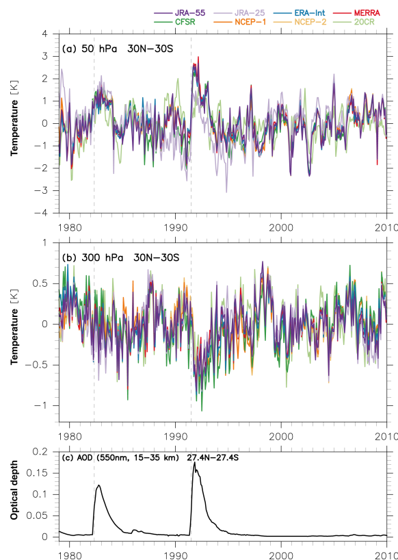
Figure 3. Time series of temperature residual R(t) (including volcanic signals and random variations) averaged for 30° N–30° S for the 1979–2009 regression analysis from eight reanalysis data sets at (a) 50 hPa and (b) 300 hPa. (c) Time series of aerosol optical depth at 550 nm averaged for 27.4° N–27.4° S and integrated for the region 15–35 km. Vertical dotted lines indicate the starting date of the two volcanic eruptions.
