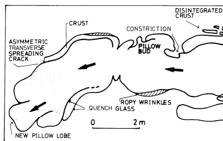
Fig. 7 Horizontal cross section of a pulsating pillow lobe. Loc. Sakae-hama (No. 25 in Fig. 2). The pillow lobe is enveloped by crusts with quench glass on both inner and outer margins. Some of the crusts have been disintegrated. It is noted that constrictions develop in front of an asymmetric transverse spreading crack, and that a pillow bud and a new pillow lobe have grown through the crust. Ropy wrinkles develop perpendicularly to the elongation of the pillow lobe.
