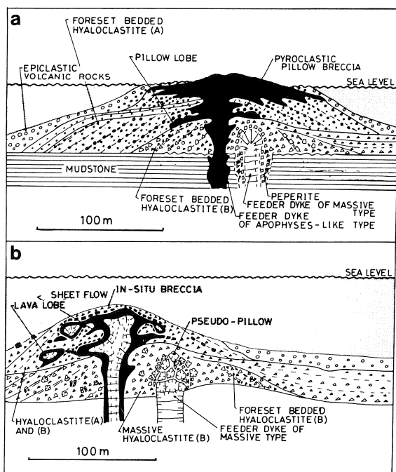
Fig. 37 Figures illustrate models of submarine volcanoes, compiled from the date of this study. a: A volcano of mafic to intermediate rocks which consist mainly of pillow lobes and hyaloclastites (A) and (B). Peperite is formed by intrusion of feeder dykes into unconsolidated mud. b: A volcano of intermediate to felsic rocks which consist of lava lobes associated with sheet flows, and hyaloclastite (B) containing pseudo-pillows.
