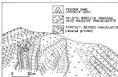
Fig. 27 Vertical exposure of a complex of feeder dykes and hyaloclastites (B). Loc. Gokibiru (No. 2 in Fig. 2). Note that the feeder dykes of massive type grade outward into massive hyaloclastite through in-situ breccia. The massive hyaloclastite grades further into foreset-bedded hyaloclastite. Another stratified hyaloclastite has truncated the complex. N: north, S: south.
