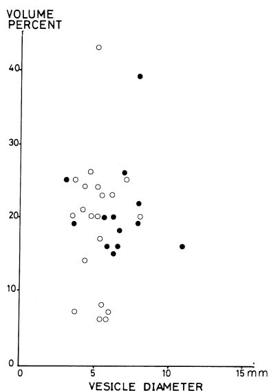
Fig. 9 Volume percent versus diameter of vesicles in pillow lobes and pillow fragments from the Suttu Formation (Loc. Yamanaka, No. 20 in Fig. 2). Open circles: pillow lobes, solid circles: pillow fragments in hyaloclastite (A). Volume percent was measured by counting ca. 100 points by the use of a transparent plate with 5 mm grids. Diameter represents the average values of largest 10 vesicles. Spherical and ellipsoidal vesicles in the upper outer (5 cm from the surface of pillows) were measured, but pipe-vesicles were omitted.
