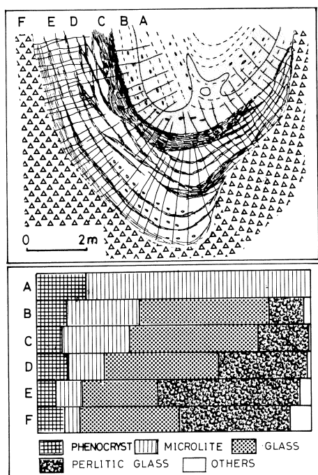
Fig. 13 Schematic sketch of a horizontal section of a rhyolite feeder dyke and modal compositions. Loc. Kawashira (No. 10 in Fig. 2). A: lithic core, B to E: flow layer zone and glassy rim, F: hyaloclastite. Approximately 500 points were counted on a thin section from each zone.
