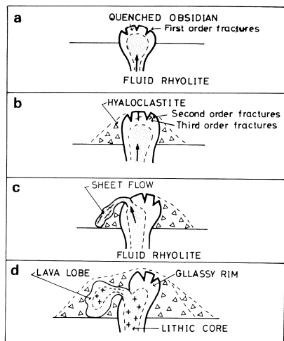
Fig. 36 Mode of the formation of lava lobe and associated hyaloclastite. a : The feeder dyke reaches the sea floor ; its surface is quenched and contraction fractures are formed perpendicularly to it. b : Second - and third - order contraction fractures develop and the quenched surface layer undergoes in-situ brecciation. c : The first-order contraction fracture taps the fluid interior of the feeder dyke, and a sheet flow extrudes upon the surface of the rubble pile, d : The forward propagation of the sheet flow produces a lava lobe. Simultaneously its surface is quenched and disaggregated.
