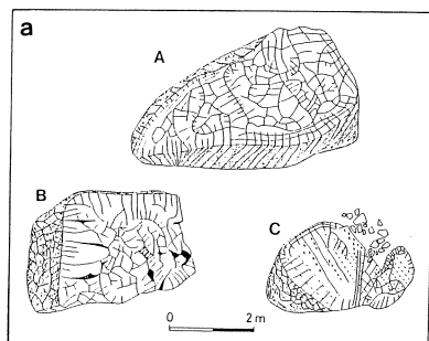
Fig. 19a Pseudo-pillows of hornblende andesite. A and B from Bikuni (No. 7 in Fig. 2) and C from Hizuka (No. 9 in Fig. 2).
