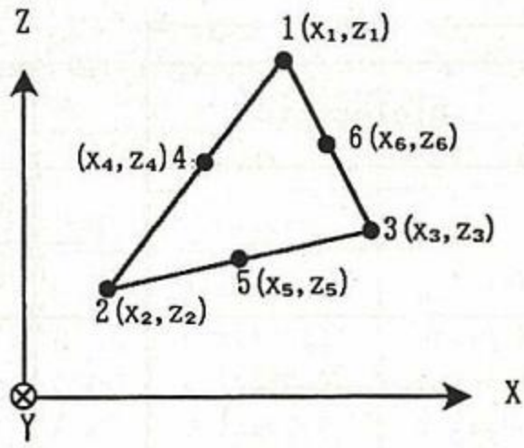
Fig. 2. Second-order triangular element.
