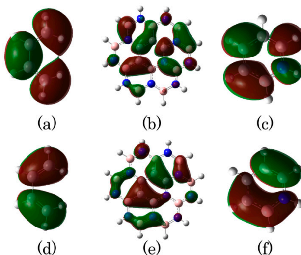
Figure 6. LUMO (a–c) and HOMO (d–f) of butadiene, C 4 B 10 N 10 H 12 , and C 4 BNH 6 .
