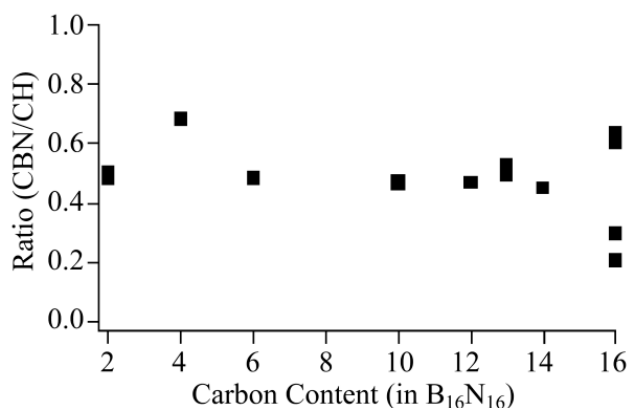
Figure 5. Ratio between bandgap of carbon doped h-BN and HOMO-LUMO gap of corresponding hydrocarbon molecules. Note that the “Carbon Content” axis shows half of that in Figure 4.
