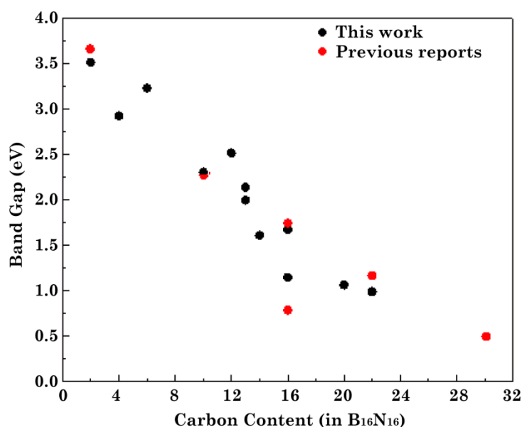
Figure 4. Band gap values as a function of carbon content in B 16 N 16 . The results of previous works [12–24] are added.
