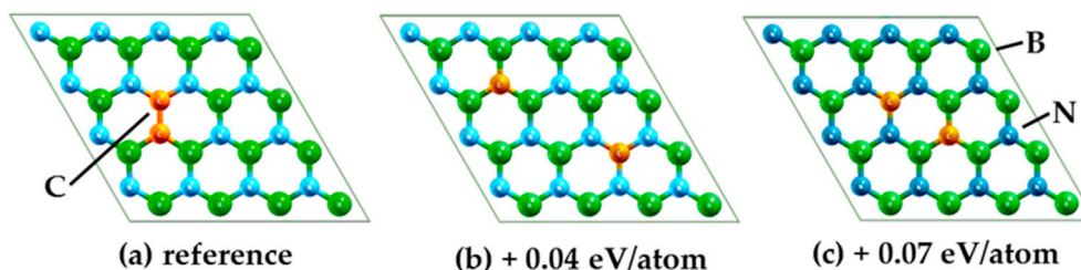
Figure 1. Relative energies of the h\text{-B}_{16}\text{N}_{16} doped with two carbon atoms. (a) lowest energy configuration; (b) two atoms separation; (c) four atoms separation.
