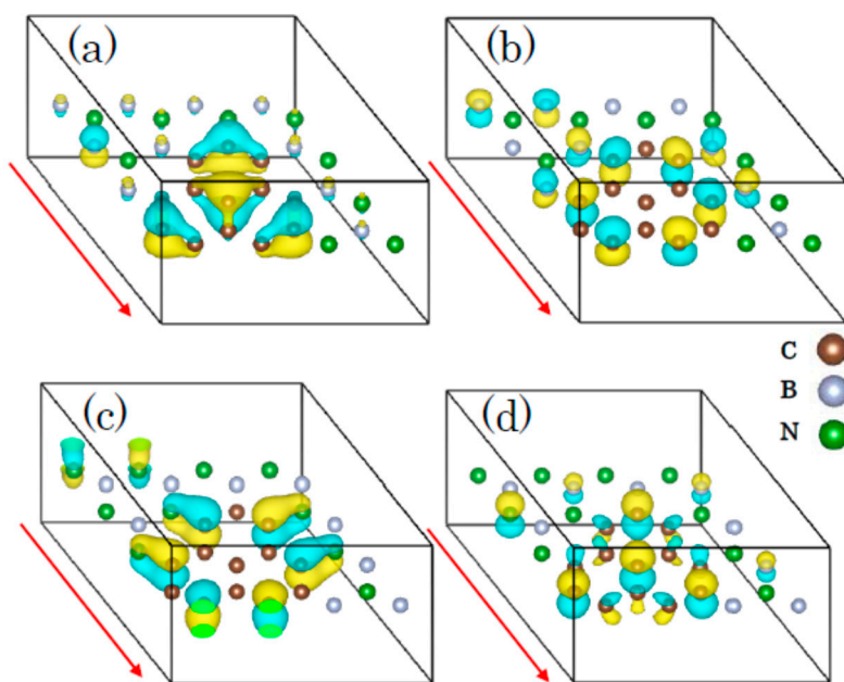
Figure 8. (a) HOMO and (b) LUMO of “N-rich phenalenyl”, and (c) HOMO and (d) LUMO of “B-rich phenalenyl”.
