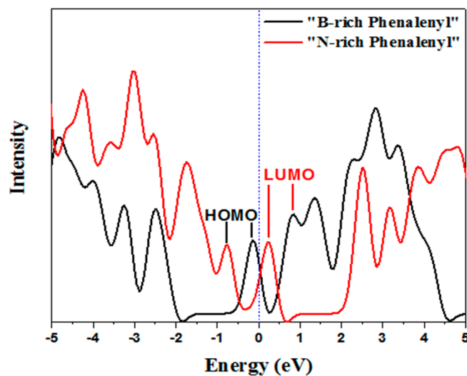
Figure 9. The DOS of the “B-rich Phenalenyl” (black curve) and “N-rich phenalenyl” (red curve).
