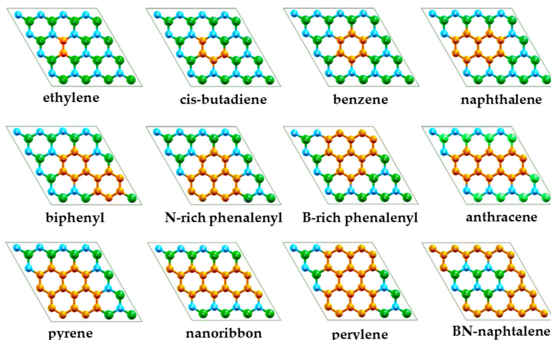
Figure 2. Structure of the carbon-doped h\text{-BN} s analyzed in this work. They are named after corresponding organic molecules.
