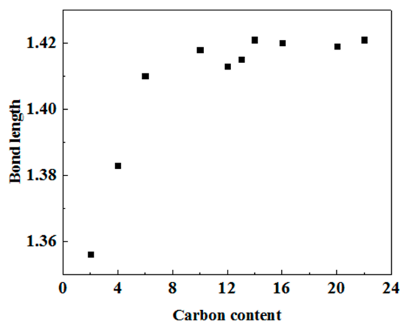
Figure 3. Average C-C bond length of carbon content.
