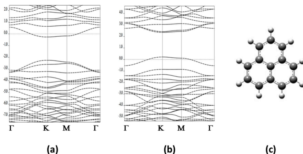
Figure 7. The band structures of “phenalenyl” doped h-BN. (a) “N-rich phenalenyl”, seven boron atoms and six nitrogen atoms were replaced by carbon atoms. (b) “B-rich phenalenyl”, six boron atoms and seven nitrogen atoms were replaced by carbon atoms. Energy zero are Fermi energies; (c) shows the structure of “phenalenyl” ( C_{13}H_9 ).
