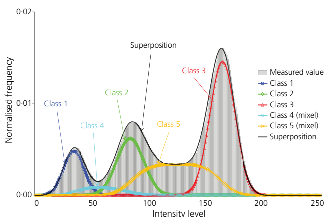
Figure 5. Example of histogram obtained from a three-phase image with lines showing the probability distributions of five classes and their superposition
