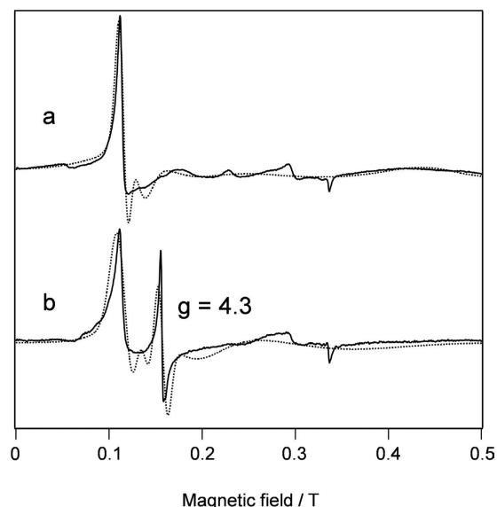
Figure 5. EPR spectra of Irr in oxidation reaction. The oxidation reaction was initiated by addition of 1.0 equivalent heme to 500 \mu L of the Irr solution (1 mM Irr, 2 mM DTT). (a) immediately after the addition of heme, and (b) after 6 hours incubation at room temperature. The observed and simulated spectra are shown in the solid and dotted line, respectively. The details of the simulation is described in Supplementary Information.
