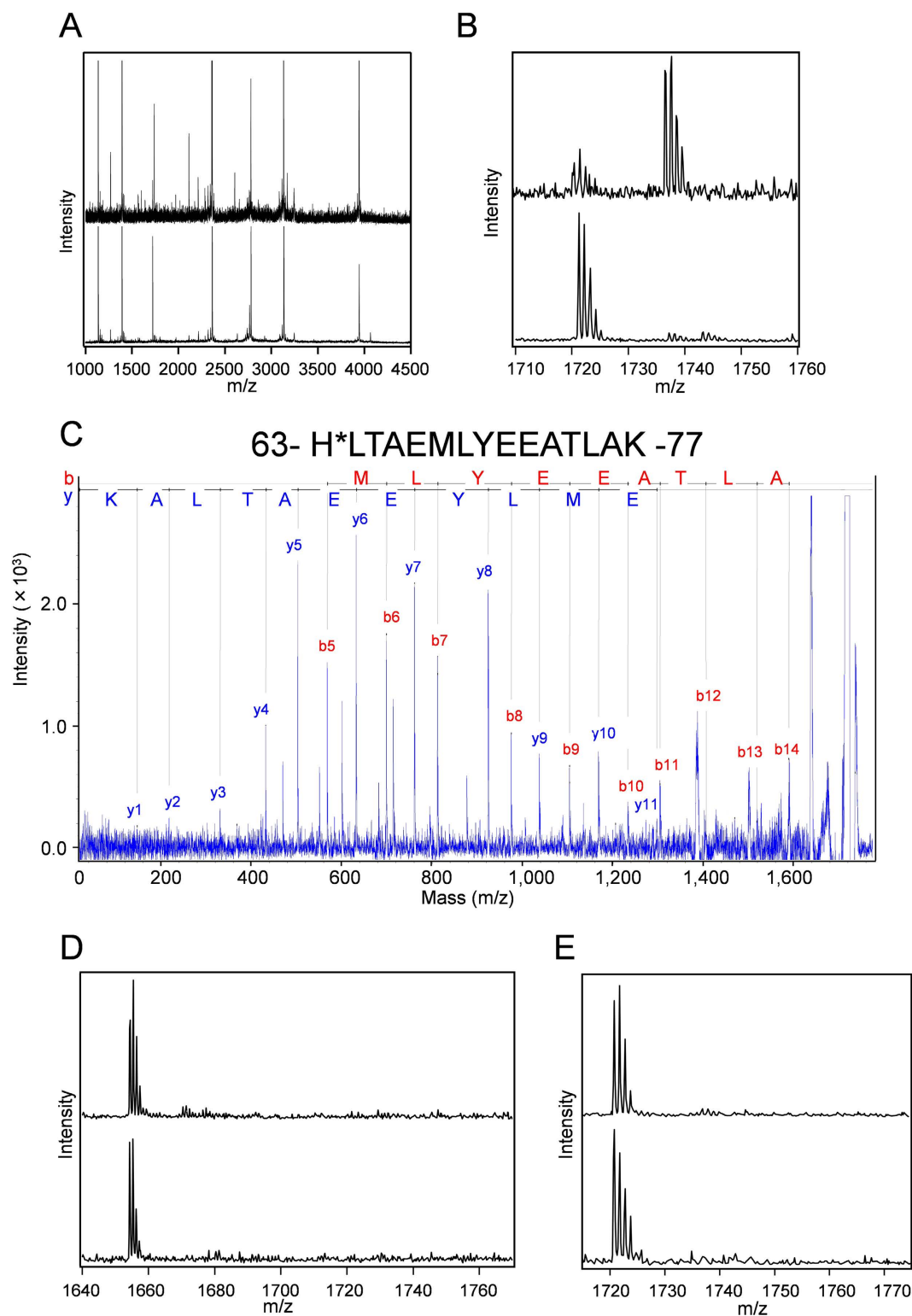
Figure 6. MALDI-TOF and MALDI-TOF/TOF spectra of the digested Irr. MALDI-TOF mass spectra of the tryptic-digested peptide fragments of Irr (40 \mu M) ( A ) 1000–4500 m/z, ( B ) 1710–1760 m/z before oxidation (lower spectrum) or after oxidation (upper spectrum). ( C ) Carboxyl-terminal (y-series) and amino-terminal (b-series) fragmentation products are shown. In the Irr 63–77 sequence, the asterisk shows the oxidation of a residue of Irr ( ^{63}\text{His} ). MALDI-TOF mass spectra of the tryptic-digested peptide fragments of the His cluster mutants (40 \mu M) ( D ) Irr (H117-119A), ( E ) Irr (H63A) before oxidation (lower spectrum) or after oxidation (upper spectrum).
