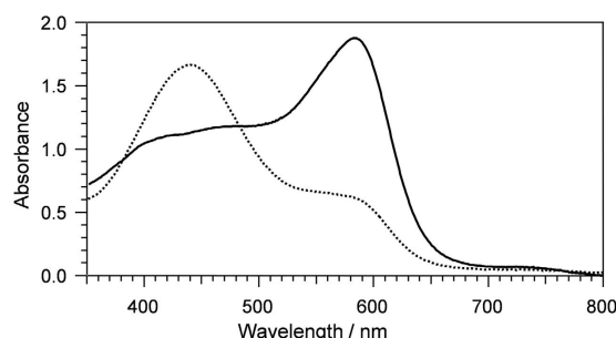
Figure 2. Spectroscopic assay for \text{H}_2\text{O}_2 generation by Irr. Absorption spectral changes for the \text{H}_2\text{O}_2 generation assay in the presence (solid line) and absence of Irr (dotted line). The reaction solution contains 125\ \mu\text{M} xylene orange and 25\ \text{mM} \text{FeCl}_2 . After 15 min incubation at room temperature, the absorption spectra were measured and the amount of generated \text{H}_2\text{O}_2 was quantified by the absorbance at 595 nm.
