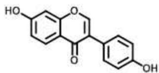
Daidzein
