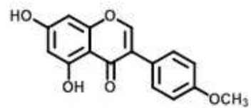
Biochanin A
