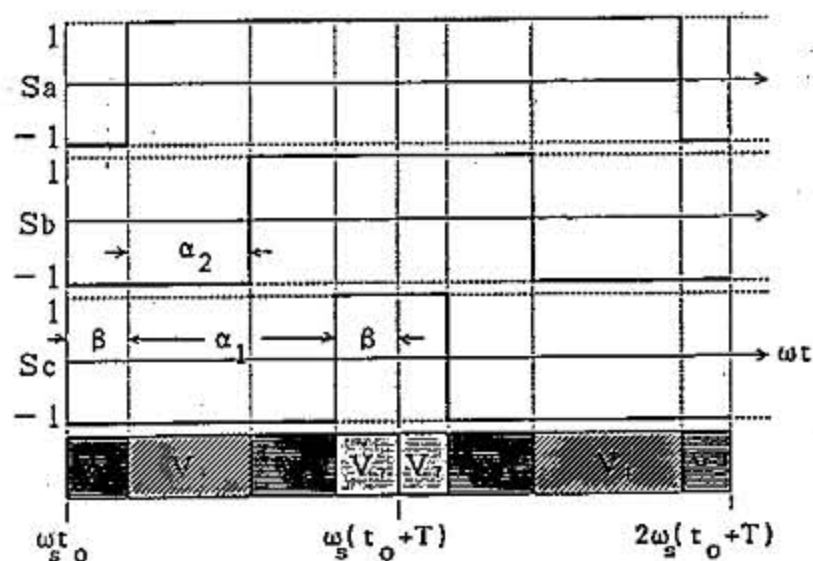
Fig. 12. Switching functions for each phase and voltage vectors used with DPWM-C for two sampling intervals.
