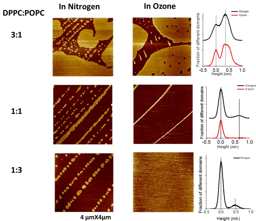
Figure 5.17 AFM images ( 4 \times 4 \mu\text{m}^2 ) of DPPC-POPC mixed monolayers on the mica surface transferred at 30mN/m (left column) before and (middle column) after exposure to low-level ozone for more than 100 min on the water surface, and the height-distribution histogram (right column) of each domain of these mixed monolayers. (Dipping directions of the monolayer transfer are shown by arrow in the images)
