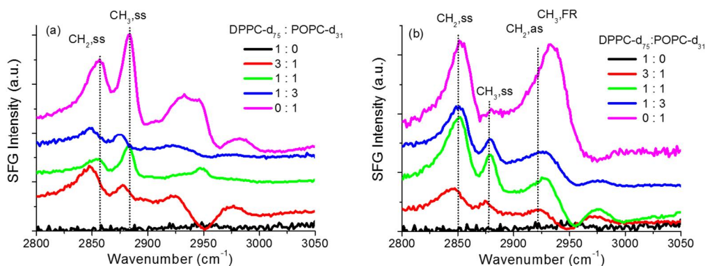
Figure 5.15 The ssp -polarized SFG spectra of DPPC-d 75 /POPC-d 31 mixed monolayers for different molar ratios observed in the C-H stretching region for unsaturated chain of POPC-d 31 component (a) before and (b) after exposure to ozone ( 20 \pm 10 ppb).
