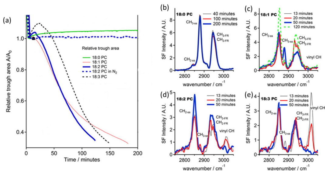
Figure 1.8 (a) Relative trough area of saturated PC (18:0), and unsaturated PCs (18:1, 18:2, 18:3) as a function of time at constant surface pressure. (b)-(e) The SFG spectra of these PCs. 93
