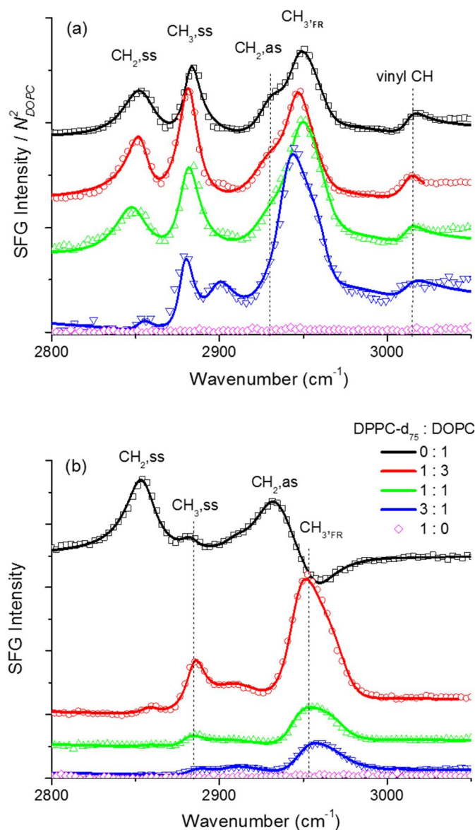
Figure 4.8 SFG spectra of DPPC-d 75 /DOPC mixed monolayers. The ssp-polarized SFG spectra of DPPC-d 75 /DOPC mixed monolayers for different molar ratios observed in the C-H stretching region for DOPC component (a) before and (b) after exposed to ozone (20 ± 10 ppb). Open symbols are SFG data, and solid traces are fitting results. In order to compare the SFG intensities of DOPC in Figure. 8a, it is normalized by the square of their relative molecular
