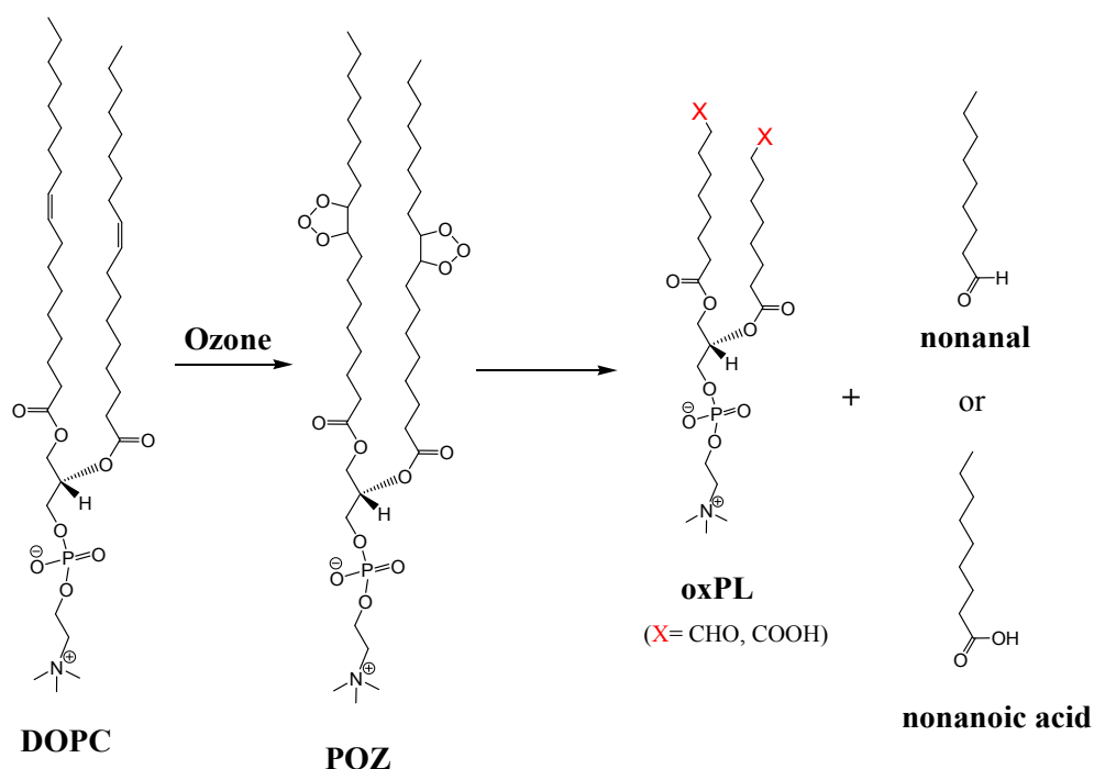
Scheme 4.1. Possible reaction mechanism of ozone oxidation on the unsaturated DOPC on the water surface.
