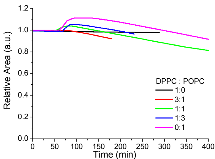
Figure 5.5 Stability of surface area for the DPPC/POPC mixed monolayers at 30 mN/m as a function of time. The monolayers are exposed to nitrogen in the first 60 min and then switched to an ozone environment ( 20 \pm 10 ppb). All the surface areas are normalized to the initial area.
