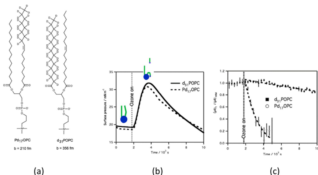
Figure 1.4 The molecule structure of Pd 17 OPC and d 31 POPC (a). The change of surface pressure (b) and fitted \rho\delta (c) as a function of time. \rho is the neutron scattering length density, \delta is the film thickness, and they are related to the reflectivity of an interface for neutrons. 53
