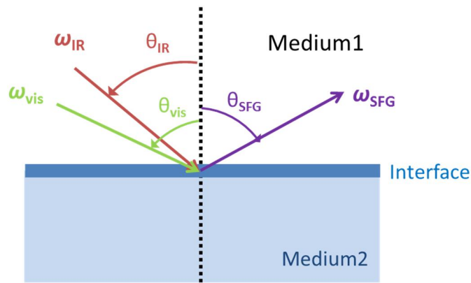
Figure 2.3 SFG with co-propagating geometry.
