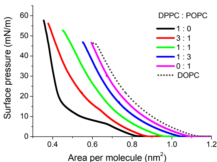
Figure 5.3 \pi -A isotherms of DPPC-POPC mixed monolayers. Pure water was used as subphase. DPPC-POPC molar ratios of 0:1, 1:3, 1:1, 3:1, and 1:0 were used. The \pi -A
