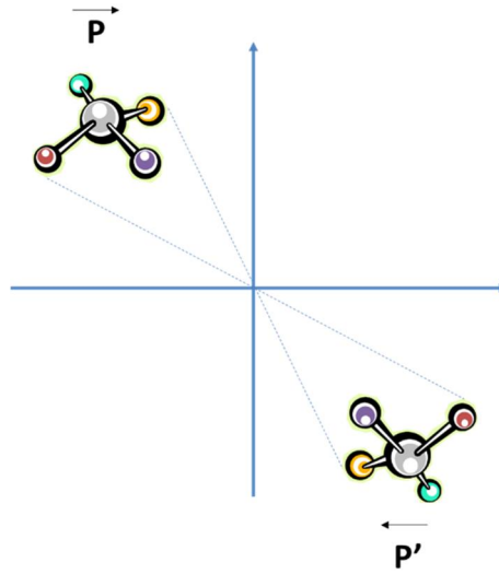
Figure 2.1 Scheme of the bulk phase with inversion symmetry
