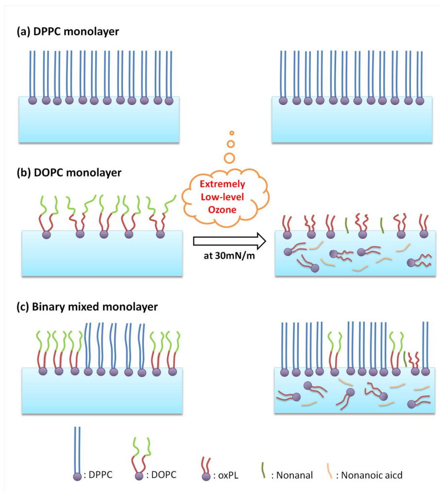
Scheme 4.2 The schematic models for DPPC-DOPC pure and mixed monolayer in nitrogen and low-level ozone. (a) DPPC monolayer, (b) DOPC monolayer and (c) DPPC-DOPC mixed monolayer on a water surface before (left) and after (right) exposure to an extremely low-level ozone. All the models schematically exhibit molecular structures per unit area at a constant surface potential of 30 mN/m. See text for details.
