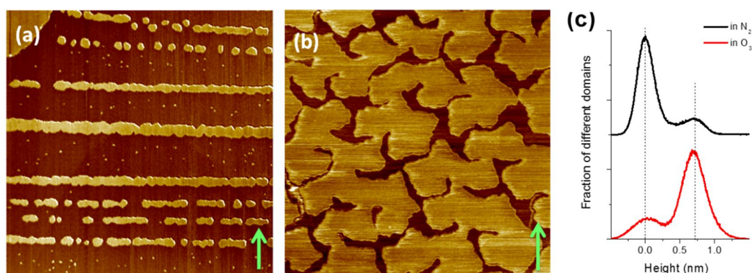
Figure 4.4 AFM images of DPPC-d 75 /DOPC (1:1) mixed monolayer and height-distribution histogram. AFM images ( 4 \times 4 \mu\text{m}^2 ) of the DPPC-d 75 /DOPC (1:1) mixed monolayer transferred from the water surface at 30 mN/m (a) before and (b) after exposure to low-level ozone. (c) The height-distribution histogram for the two AFM images. The arrows in the AFM images show the direction of the monolayer transfer.
