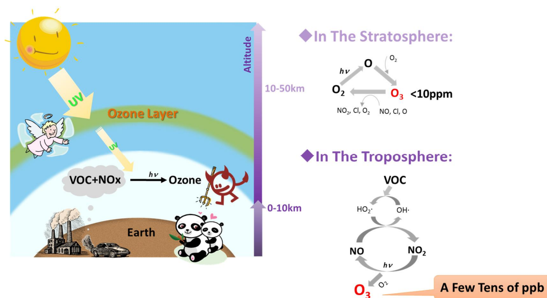
Figure 1.3 The processes of ozone formation in the atmosphere.
