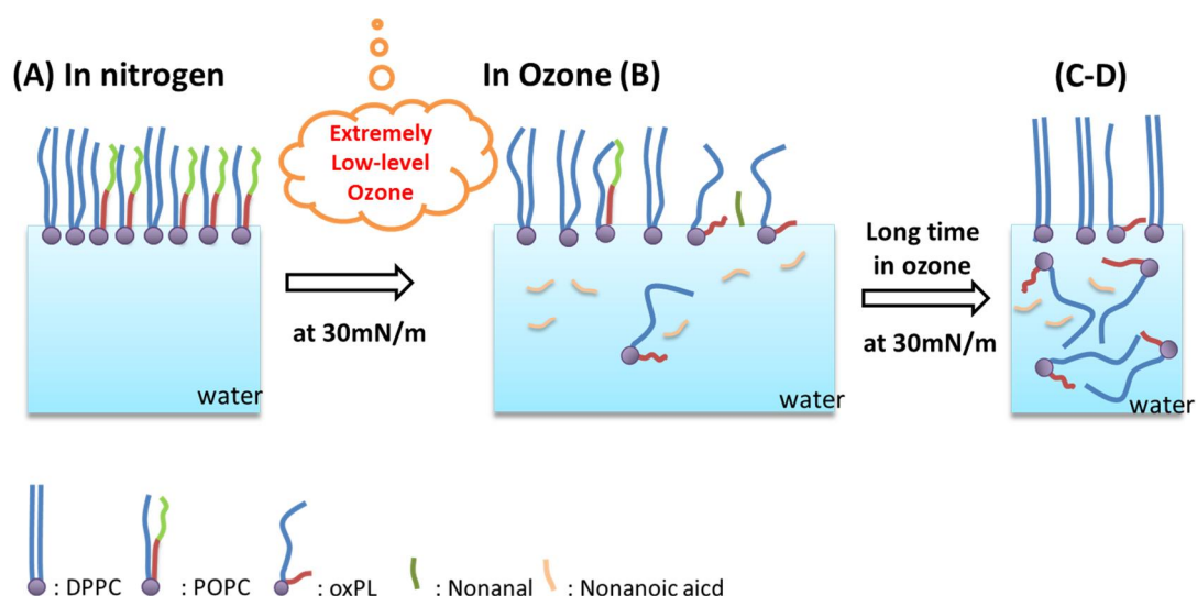
Scheme 5.3 Schematic representations of DPPC-POPC mixed monolayer after exposure to ozone for different time scale. (A) before ozone exposure (B) exposure for 100min (C-D) exposure more than 400 min and 10hours.
