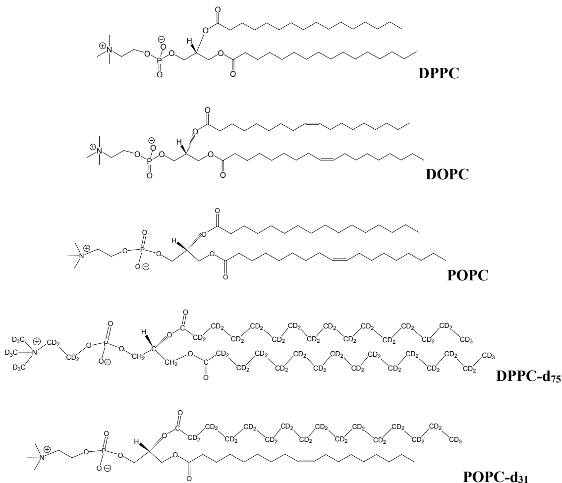
Figure 3.1 Molecular structures of DPPC, DOPC, POPC, DPPC- d_{75} , and POPC- d_{31} .
