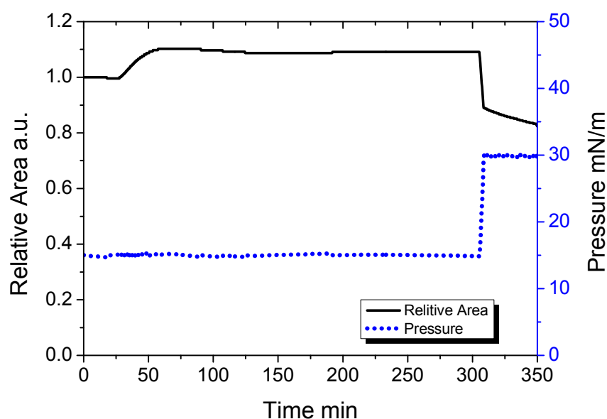
Figure 5.6 Stability of surface area of the POPC monolayer at 15 mN/m exposed to nitrogen (0-40 min), and then introducing ozone into the chamber (40-350 min, 20 \pm 10 ppb), and the surface pressure is increased to 30 mN/m at 300 min. All the surface areas are normalized to the initial area. The surface pressure is also shown in the figure.
