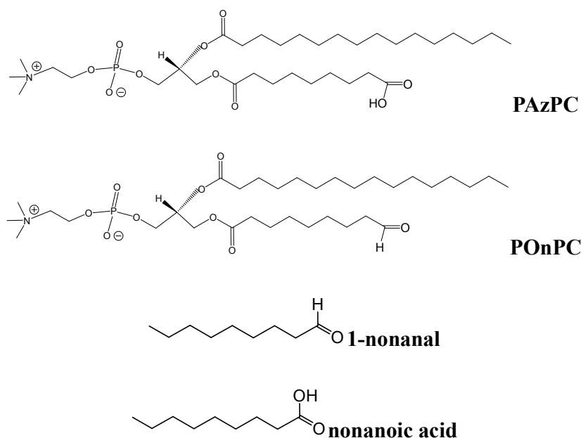
Figure 3.2 Molecular structures of oxidized phospholipids PAzPC and POnPC, and their counterpart residues 1-nonanal and nonanoic acid.
