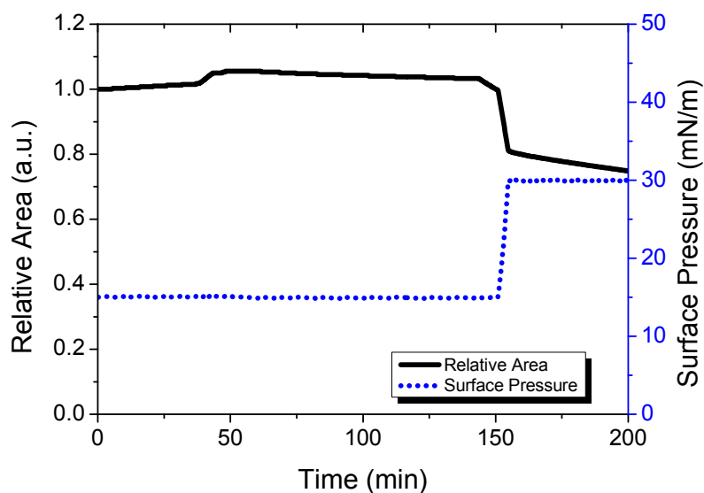
Figure 5.7 Stability of surface area of the DPPC-POPC 1:1 monolayer at 15 mN/m exposed to nitrogen (0-40min), and then introducing ozone into the chamber (40-150min, 20 \pm 10 ppb). After 150 min, the surface pressure is increased to 30 mN/m. All the surface areas are normalized to the initial area. The surface pressure is also shown in the figure.
