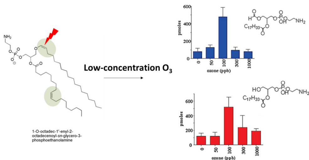
Figure 1.5 The molecule structure of 18:0p/18:1-PE and oxidation products generated by ozone exposure (0,50,100,300, and 1000ppb). (a)1-Formyl-2-octadecenyl-PE (b)1-hydroxy-2-octadecenyl-PE
