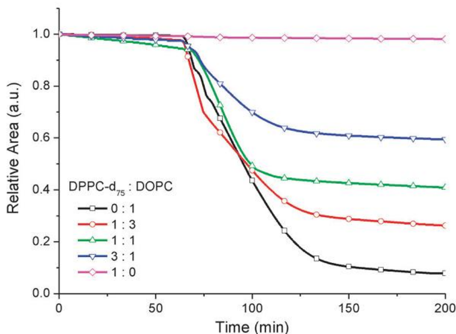
Figure 4.3 Stability of surface area for the DPPC-d 75 /DOPC mixed monolayers at 30 mN/m as a function of time. The monolayers are exposed to nitrogen in the first 60 min and then switched to an ozone environment ( 20 \pm 10 ppb). All the surface areas are normalized to the initial area. See text for details.
