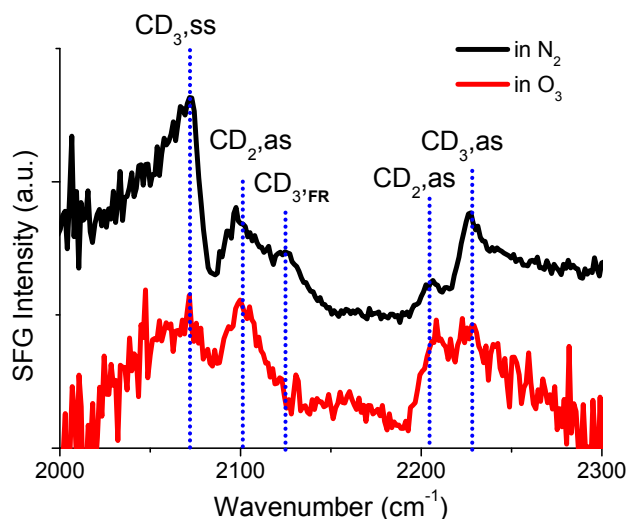
Figure 5.10 Ex-situ SFG spectra of pure POPC-d 31 monolayer in C-D stretching region in nitrogen and ozone. The spectra are offset for clarity.
