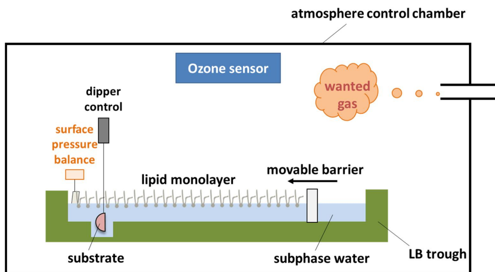
Figure 3.3. Scheme of a LB trough in the sealed chamber with surface pressure, dipper, and atmosphere control.
