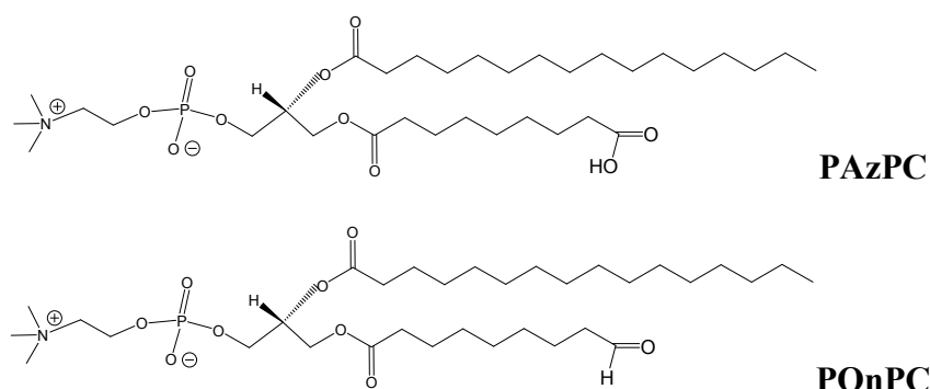
Figure 5.2 Molecular structures of oxidized phospholipids PAzPC and POnPC, and their counterpart residues 1-nonanal and nonanoic acid.
