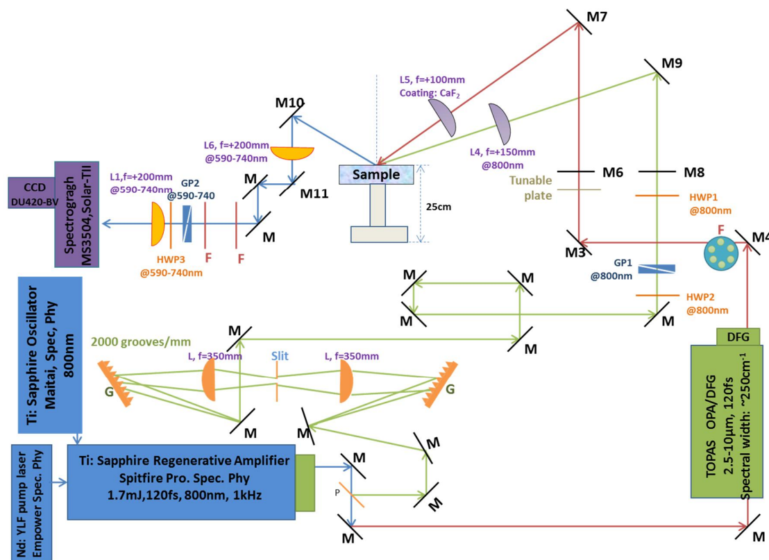
Figure 3.5. Scheme of the broad-band SFG setup. A laser system (in color of blue and green), pulse shaper (orange), sample stage (grey), and detection devices (purple). In the pulse shaper, the gratings and the slit are placed in the focal plane of the lens. The visible beam pass is in green, IR beam pass is in red, and SFG beam pass is in blue. Abbreviations: M mirror, L lens, HWP half wave plate, GP Glan prism, F filter, and HWP half wave plate.
