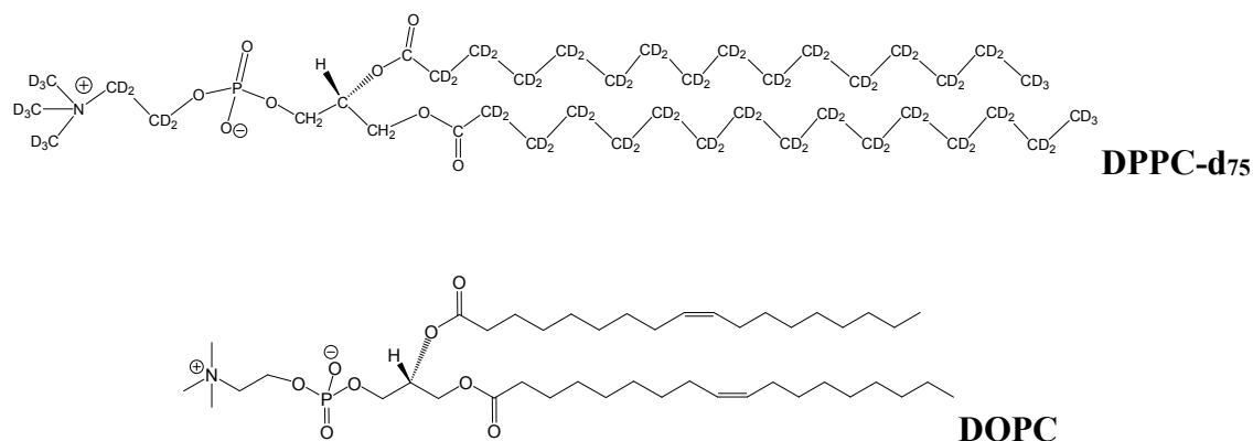
Figure 4.1 Molecular structures of DPPC-d 75 , and DOPC.
