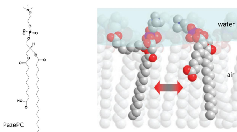
Figure 1.6 The molecule structure of oxidized phospholipid PazePC (left) and the scheme shows the reorientation of the oxidized portion at air-water interface (right). 67, 76
