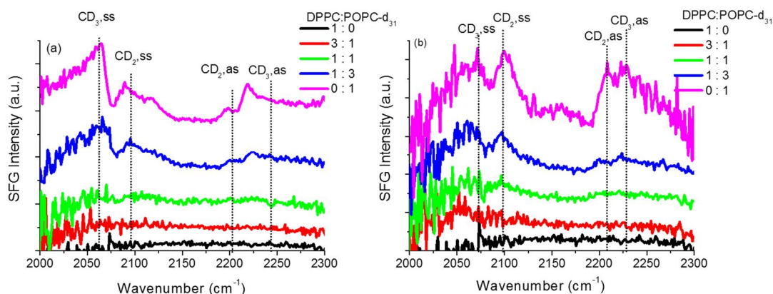
Figure 5.16 The ssp -polarized SFG spectra of DPPC/POPC- d_{31} mixed monolayers for different molar ratios observed in the C-D stretching region for saturated chain of POPC- d_{31} component (a) before and (b) after exposure to ozone ( 20 \pm 10 ppb).
