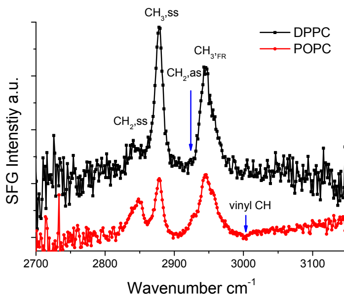
Figure 5.8 The ssp -polarized in-situ SFG spectra of DPPC (black trace) and fresh POPC (red trace) in lab air at 30 mN/m. The spectra are offset for clarity.
