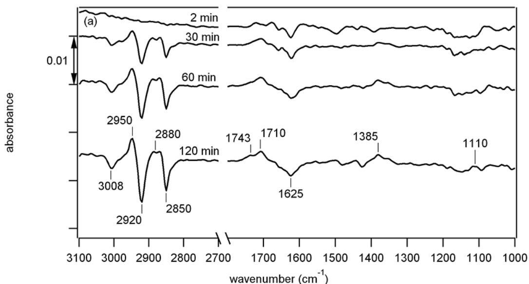
Figure 1.7 DRIFTS spectrum of POPC/ Instant Ocean (IO, a synthetic sea salt) during reaction with 1.2 \times 10^{13} ozone cm -3 . Absorbance is normalized by the single beam spectrum of unreacted POPC/IO. 77
