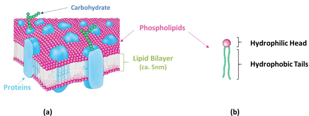
Figure 1.1 Typical views of a cell membrane (a) and phospholipid molecule (b). 6
