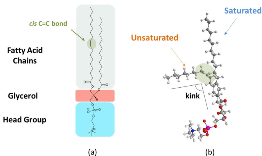
Figure 1.2 Molecular structure of unsaturated phospholipid POPC.
