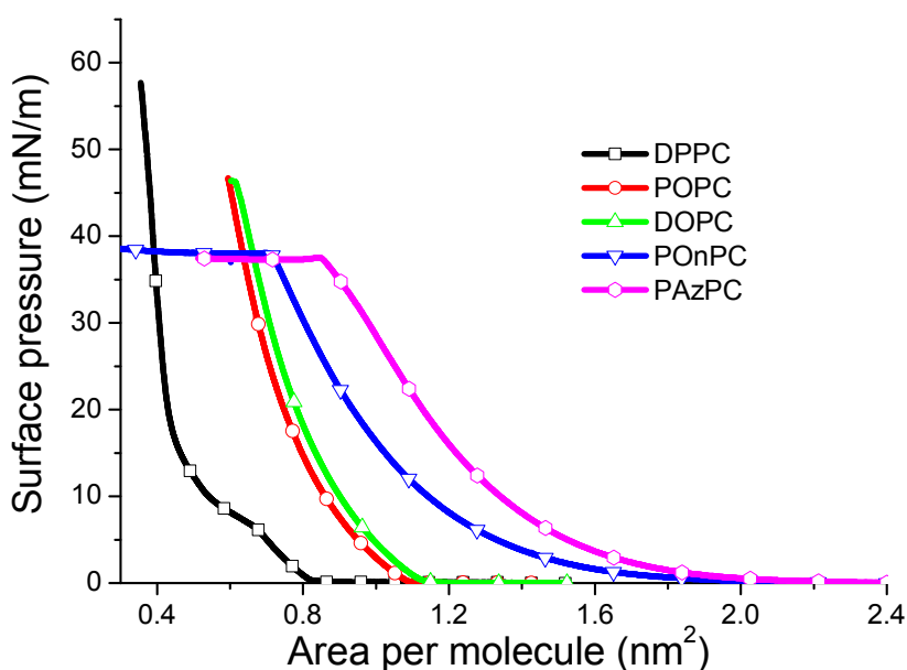
Figure 5.12 \pi -A isotherms of DPPC, POPC, DOPC, and oxPLs including POnPC and PAzPC. The \pi -A isotherms were obtained on a pure water surface (22°C) under nitrogen atmosphere and in dark.
