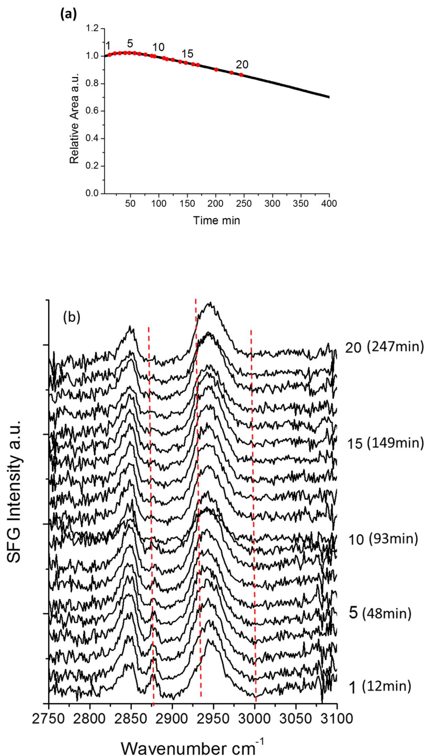
Figure 5.9 (a) The time dependence curve of the POPC monolayer in air at 30 mN/m; (b) In-situ SFG spectra of pure POPC- \text{d}_{31} in C-H stretch region as a function of the exposure time in lab air. The red dot in (a) is the mark for the time when probed SFG spectra.
