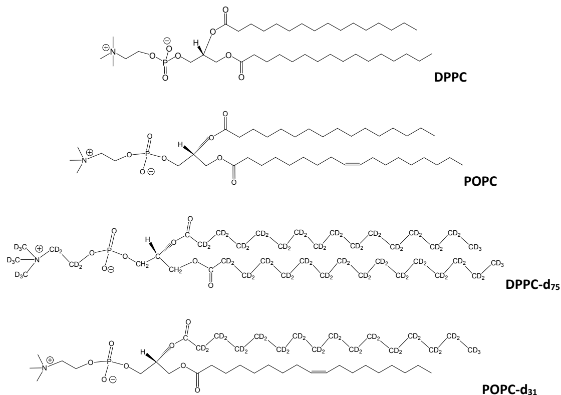
Figure 5.1 Molecular structures of DPPC, POPC, DPPC-d 75 , and POPC-d 31 .
