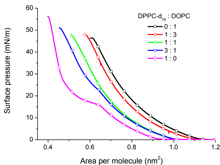
Figure 4.2 \pi -A isotherms of DPPC-d 75 /DOPC mixed monolayers. The \pi -A isotherms is
