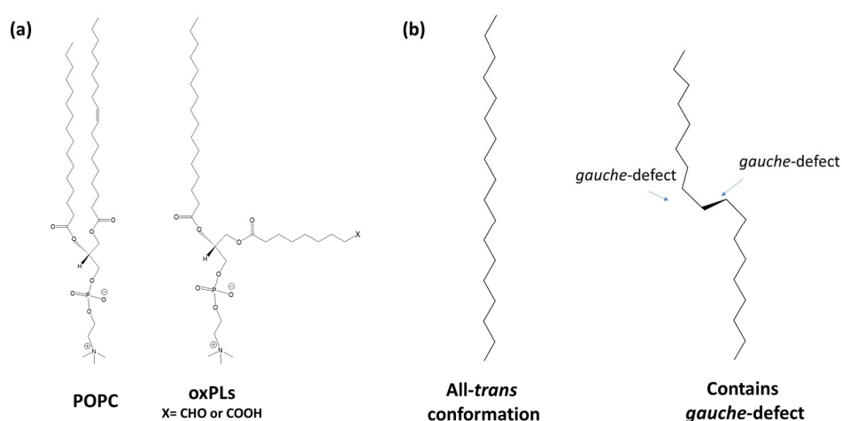
Scheme 5.2 The scheme of reason for the increase of POPC monolayer area after exposed to ozone. (a) reorientation of the oxidation modified alkyl chain. (b) alkyl chains with all-trans conformation and contains two gauche -defects. 14, 32
