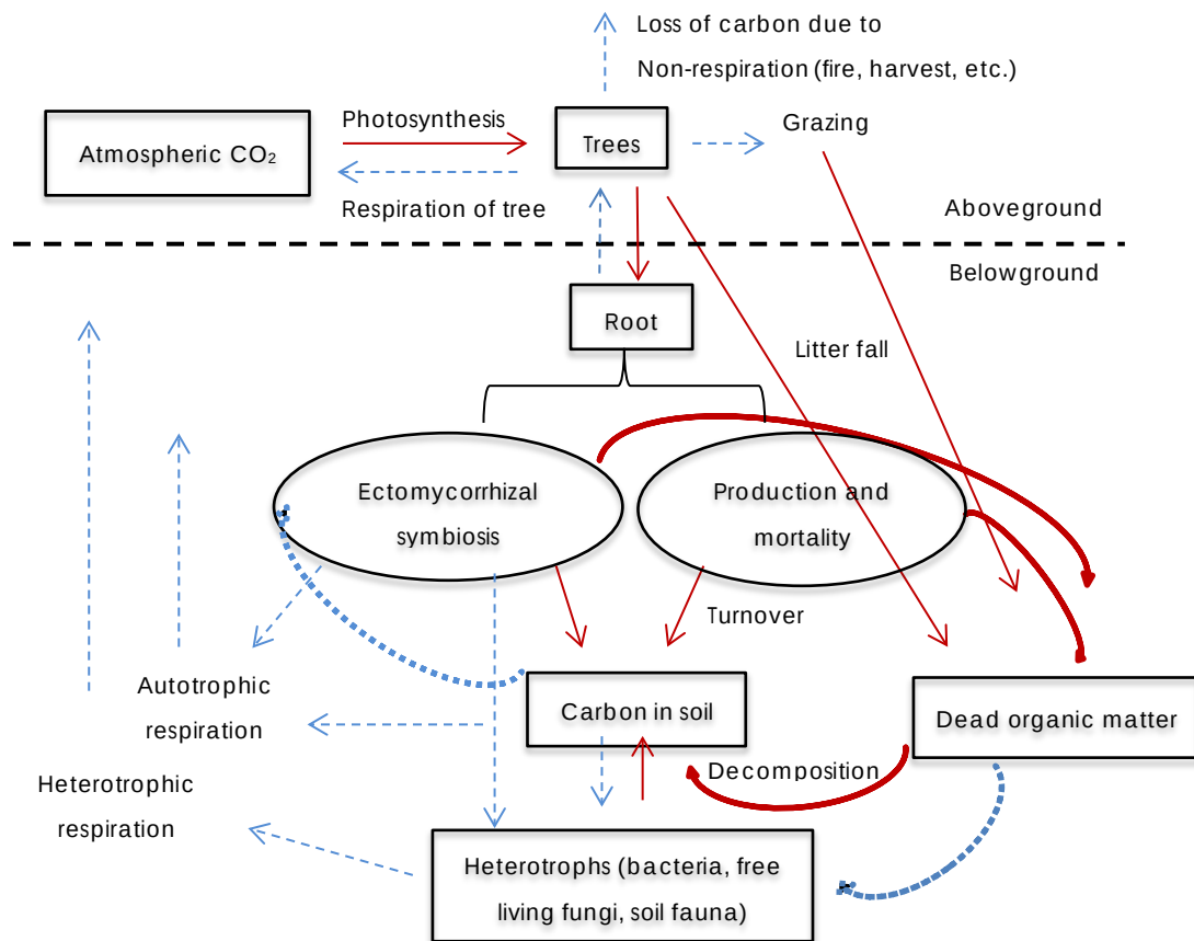
Figure 1.1 Schematic overview of the important role of ectomycorrhizal symbiosis and root dynamics in forests carbon cycling. Carbon pools are represented with boxes and circles, carbon fluxes by arrows (Solid line denotes the increase and dash line denotes the reduction) and processes are marked with text only (illustrated partly based on the idea of Fransson 2012).
