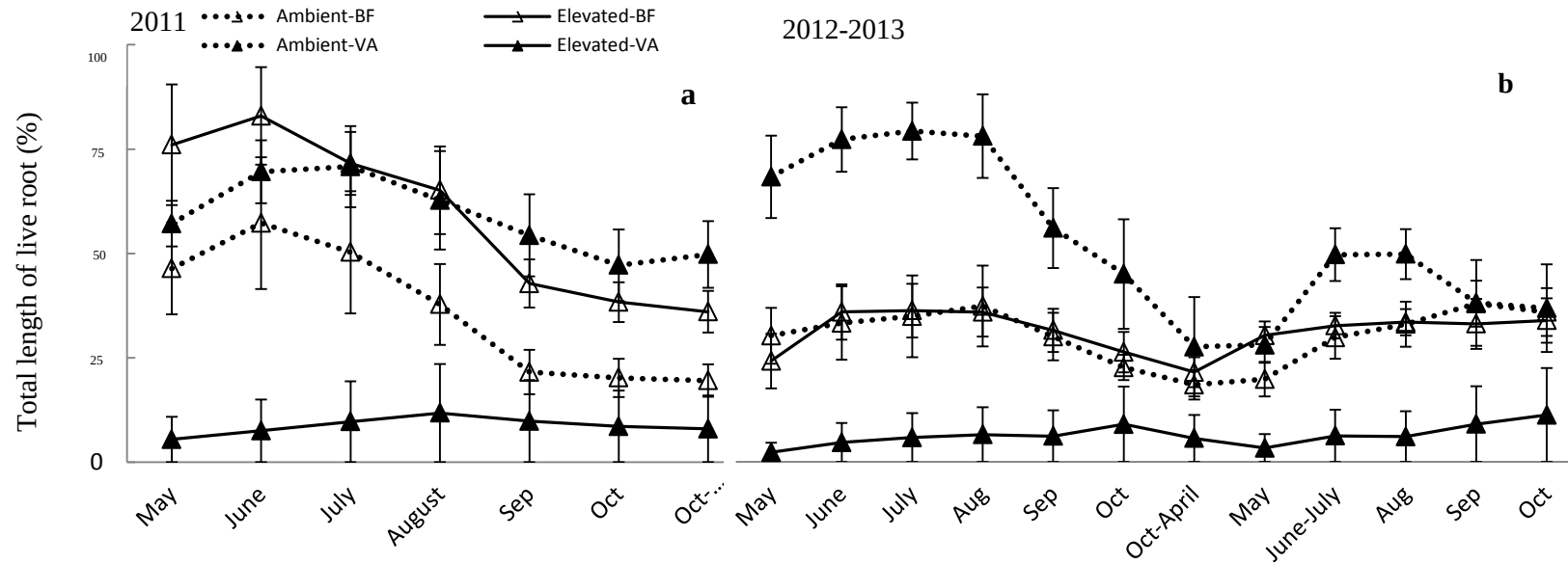
Figure 2.3 Relative length of live fine root (standing crop) of white birch seedlings growing under elevated ( 500 \text{ } \mu\text{mol mol}^{-1} ) and control ( 370 \text{ } \mu\text{mol mol}^{-1} ) [\text{CO}_2] on volcanic ash (VA) and brown forest (BF) soil.
