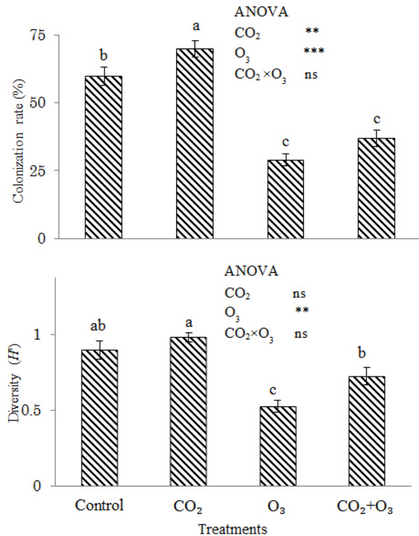
Figure 3.2 Ectomycorrhiza (ECM) colonization rate and diversity of hybrid larch F 1 under different treatments at the end of the experimental period. The ECM diversity ( H' ) was calculated as Shannon's diversity index, and each value is the average of four chamber replications. A vertical bar indicates the standard error. Different character symbols denote the degree of significance between the four treatments ( P < 0.05 ). ANOVA: ** P < 0.01 , *** P < 0.001 , "ns" means not significant.
