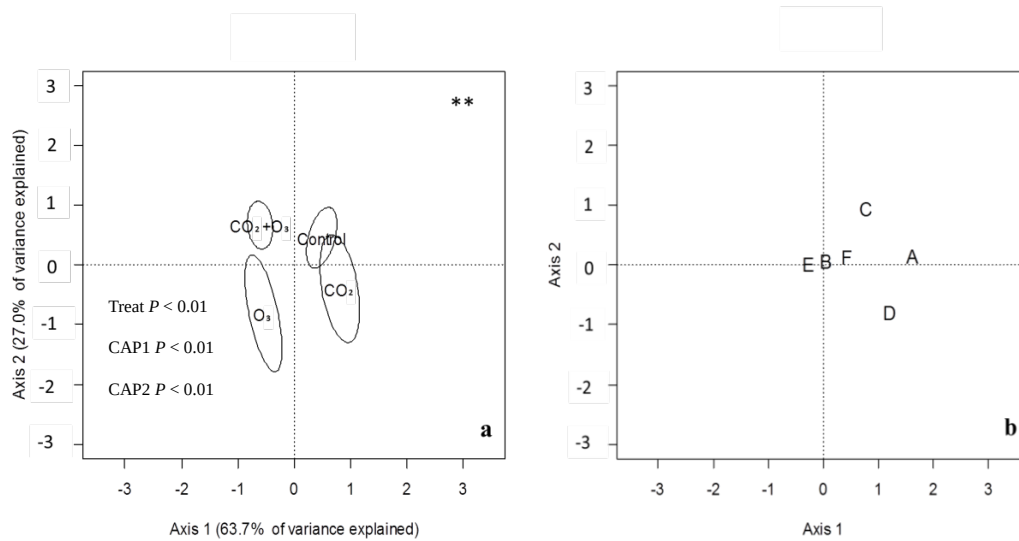
Figure 3.3 Abundance of colonized ECM species in response to four fumigation treatments at the end of the experimental period. The colonization rate, together with diversity of different ECM species, was estimated using a distance-based redundancy analysis (db-RDA) among the four gas treatments. The db-RDA depends on the matrix created using ECM species and the four treatments, and it calculates the eigenvalues and their contribution to the squared Bray distance. The results of the ANOVA use permutation tests for capscale under a reduced model (CAP1, CAP2, and CAP3 are shown). Independent variables are identified as factors (Treat.) CAP1 and CAP2 refer to axis 1 and axis 2 information, respectively, and they represent the proportion explained by the difference between each treatment. From the R results, we determined that the directions of both axis 1 ( P = 0.005 ) and axis 2 ( P = 0.005 ) were significantly different. This result indicates that the abundance of colonized ECM species from elevated O_3 and mixed conditions was largely different from that of control and elevated CO_2 conditions (axis 1 direction). Between elevated O_3 and mixed conditions, the abundance of ECM species was also markedly changed (explained by axis 2). An asterisk refers to significant codes: **P < 0.01 .
