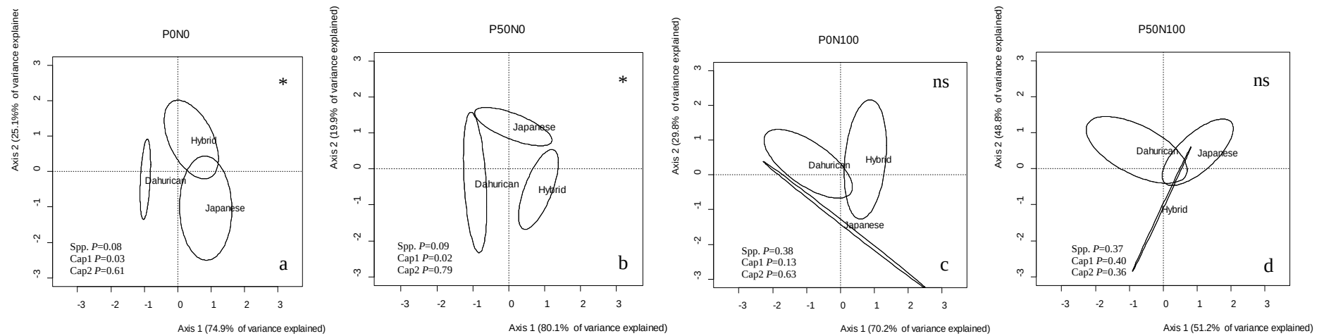
Figure 4.4 Community structure of ECM species with the three Larix species as factors among the different nutrient regimes. Results of distance-based redundancy analysis, with symbols indicating the results of ANOVA: *, P \leq 0.05 ; ns, not significant.
