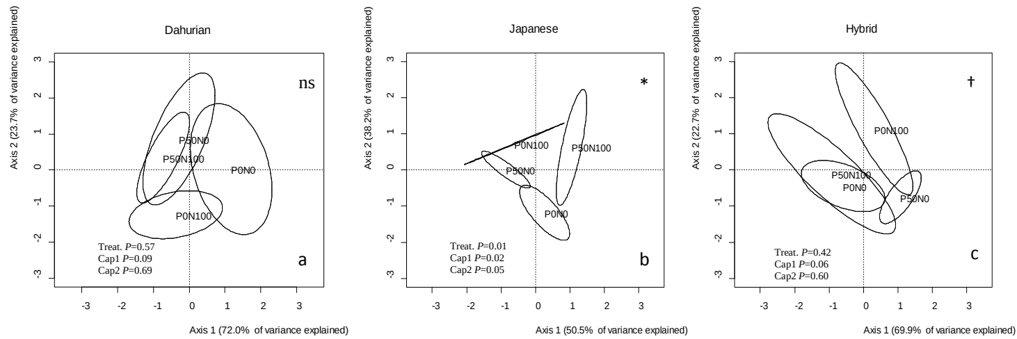
Figure 4.3 Community structure of ECM species with nutrient treatments as factors among the three Larix species. Results of distance-based redundancy analysis, with symbols indicating the results of ANOVA: †, P \leq 0.10 ; *, P \leq 0.05 ; ns, not significant.
