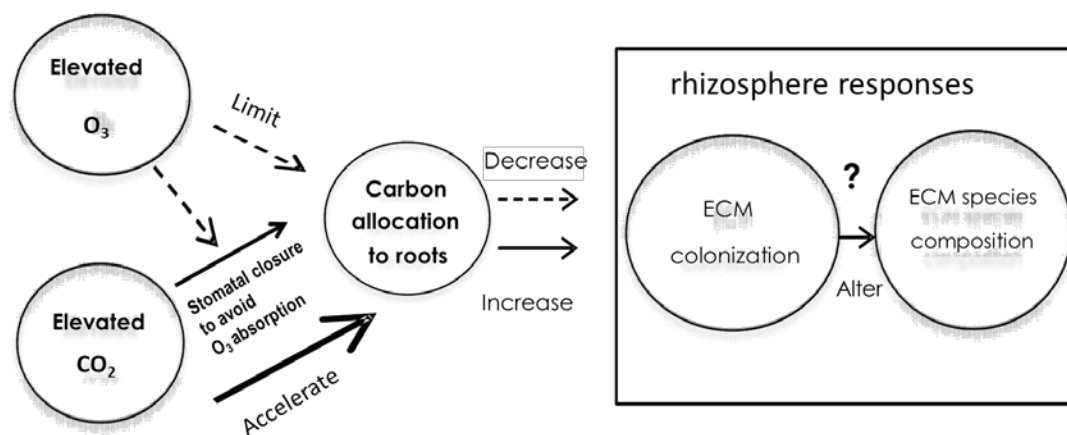
Figure 1.2 Relation between carbon allocation to belowground of a host tree, and the ectomycorrhizal symbiosis under elevated \text{CO}_2 and \text{O}_3 . Arrows shows the carbon driver of different factors (Solid line denotes enhancing factor and dashed line denotes the limiting factors) (Wang XN original)
