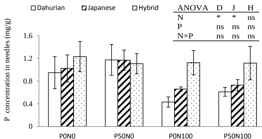
Figure 4.5 Concentration of P in needles of three larch species under the different nutrient treatments. Each value is the mean of six replications, and the error bar shows SE. ANOVA: *, P < 0.05 ; ns, not significant. D, J and H are the abbreviations for three larch species.
