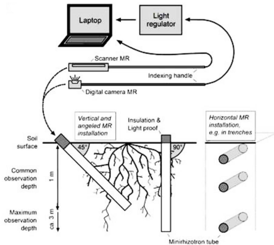
Figure 2.1 Schematic of Minirhizotron (MR) techniques, (Image capture instrument with Digital Camera or Scanner MR) and different options to install the MR tubes (angled or vertical from the soil surface or horizontally from trenches) (Maeght et al. 2013).
