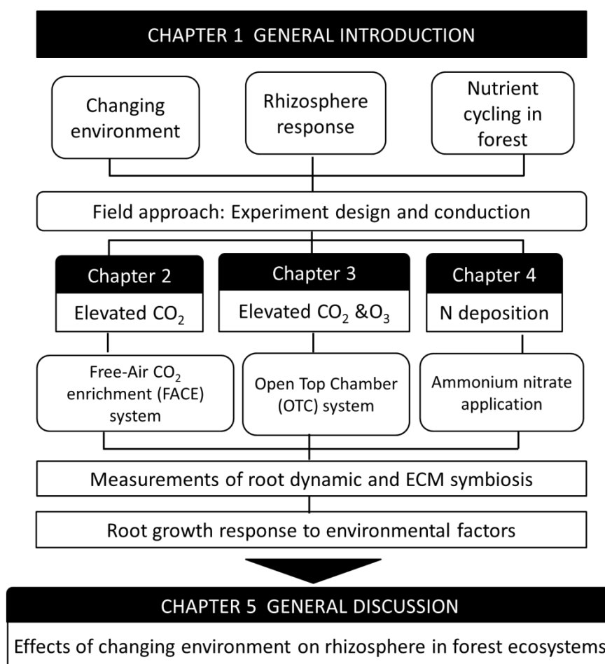
Figure 1.3 Structure of this study
