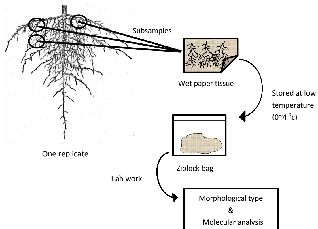
Figure 3.1 The sampling process for an individual seedling replicate. Three subsamples were randomly selected.
