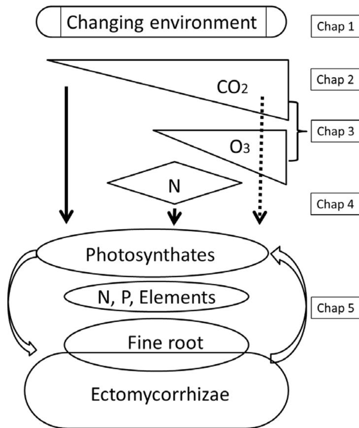
Figure 1.4 Impact scale and interaction effect of different environmental factors.
