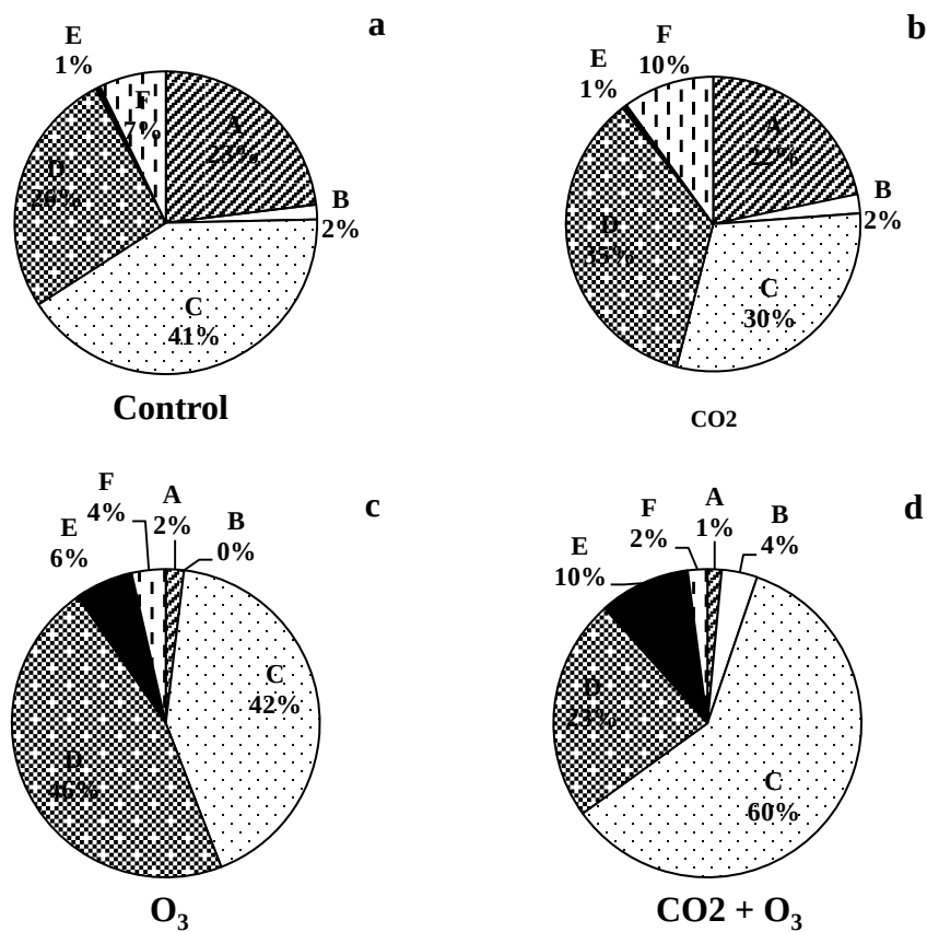
Figure 3.4 Changes in the abundance of the ECM community of the four treatments. Each value is the proportion of each type of ECM identified with the hybrid larch F 1 under the four types of fumigation (a, b, c, d). a: Tomentella sp. B: Peziza sp. C: Suillus laricinus D: S. grevillei E: Cadophora finlandia F: Laccaria cf. laccata
