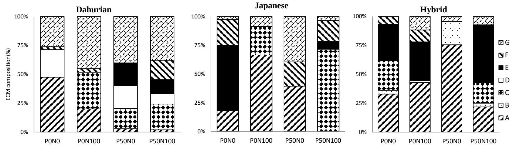
Figure 4.1 Composition of ECM fungal species of three larch seedlings with four different nutrient regimes. The different streak symbols correspond to the proportions of ECM fungal types colonizing host seedlings; values are calculated from the colonization rate of ECM fungi in different nutrient conditions.
