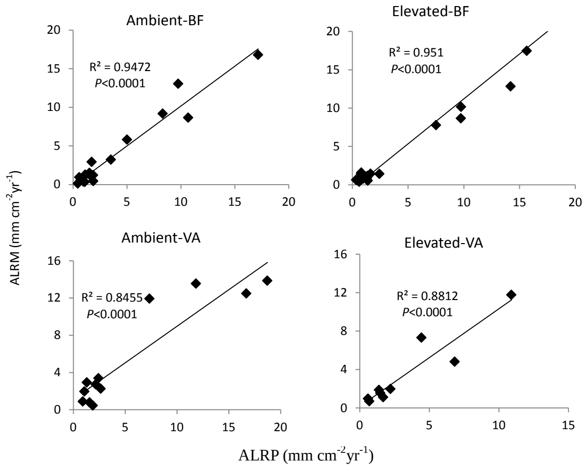
Figure 2.6 Relationship between annual length-based root production (ALRP) and annual length-based root mortality (ALRM) in each tube and treatment. Pearson correlation test showed P < 0.0001 .
