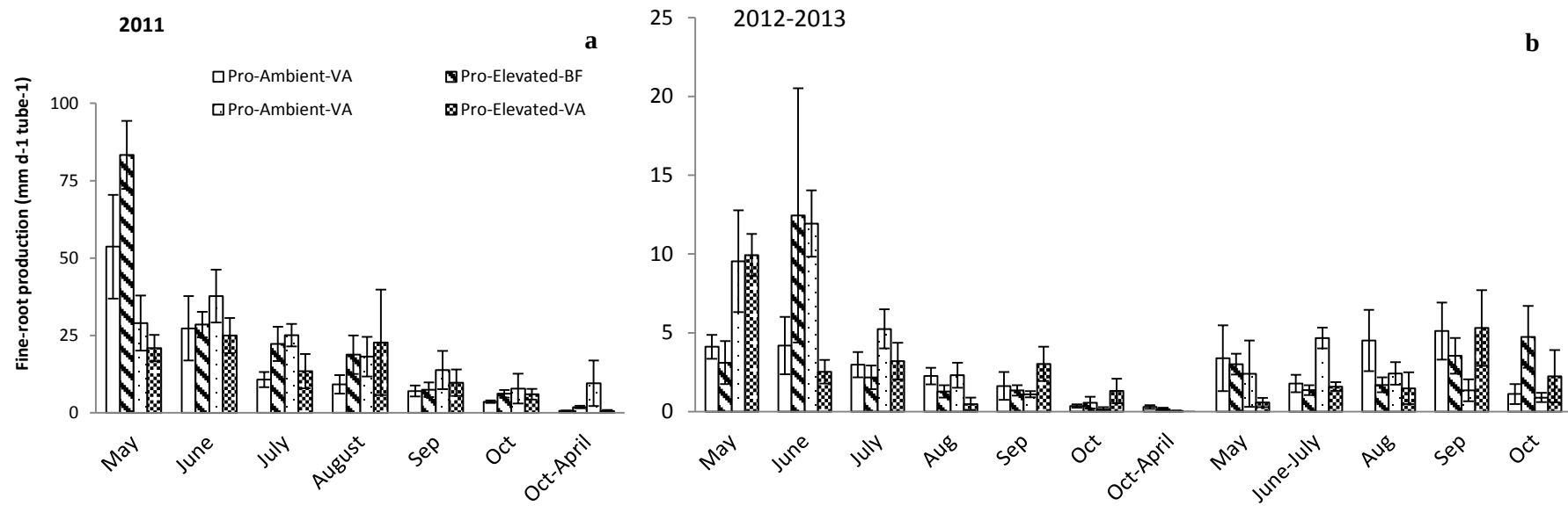
Figure 2.4 Fine root length production rate of birch seedlings growing under elevated and ambient [CO 2 ] on volcanic ash (VA) and brown forest (BF) soil.
