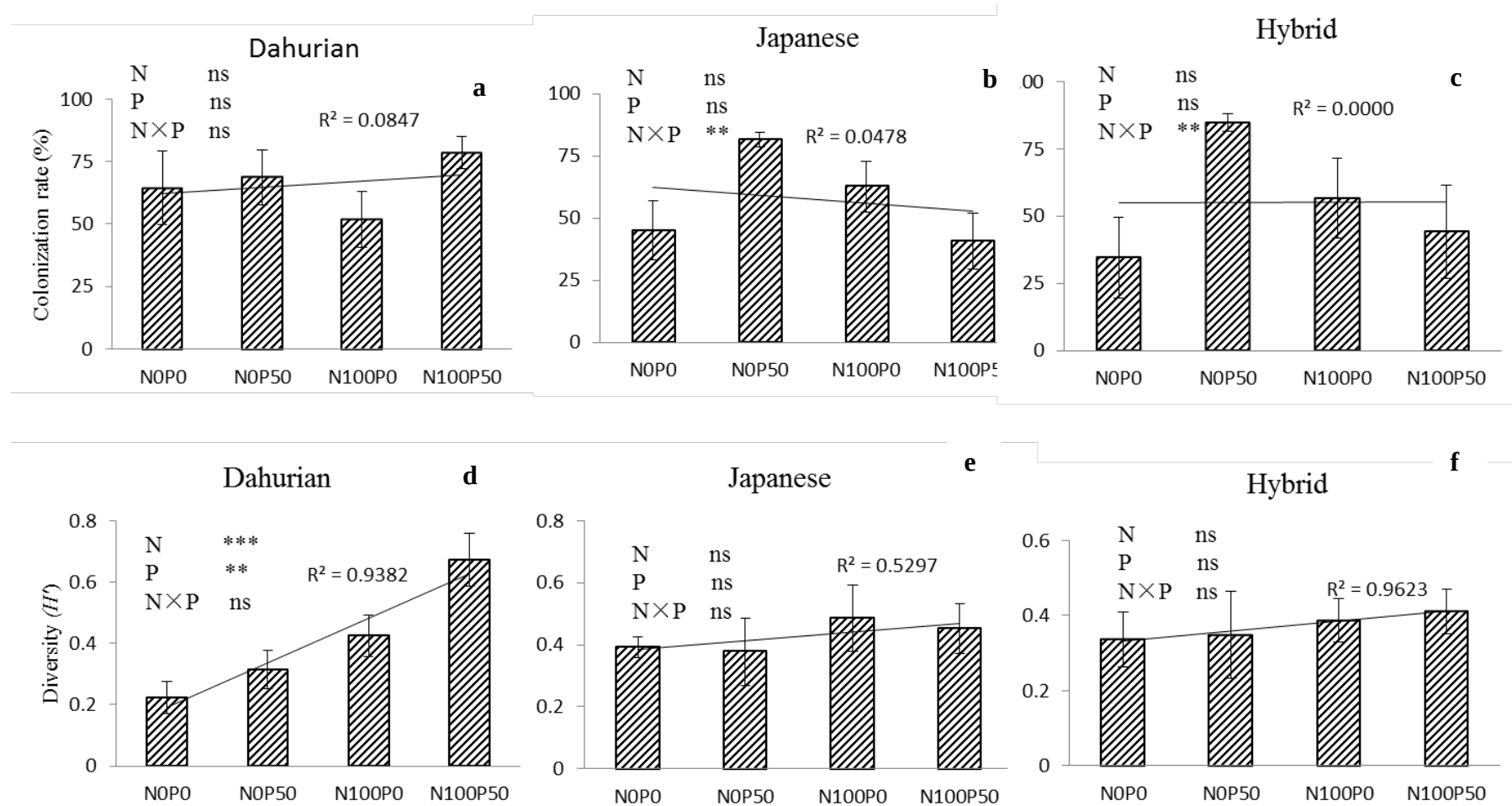
Figure 4.2 ECM colonization rate and species diversity of three larch seedlings under different N and P treatment. Each value is the average of six replications, and the error bar denotes the SE. ANOVA: *** P < 0.001 , ** P < 0.01 , ns: not significant.
