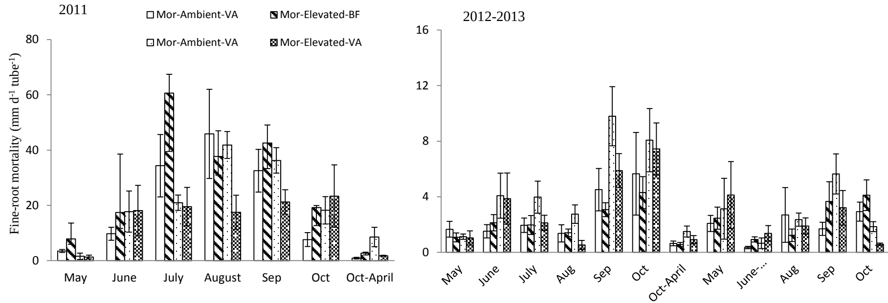
Figure 2.5 Fine root length mortality of birch seedlings growing in elevated and ambient [CO 2 ] on infertile volcanic ash (VA) and fertile brown forest (BF) soil.
