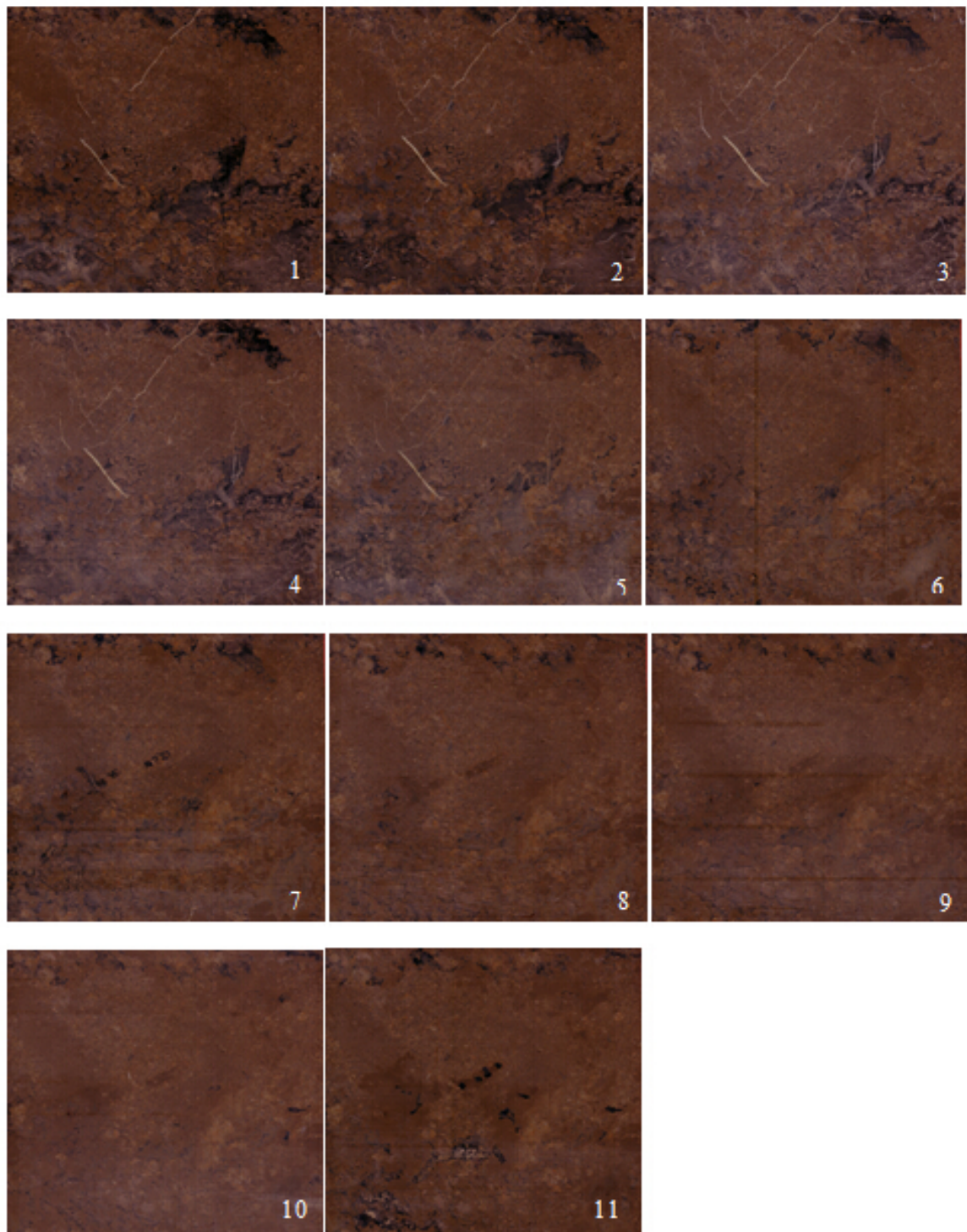
Figure.2.2 Root images captured in one tube from the first session to the last one during one year observation. The accurate size of each image is 21.59 \times 19.56 \text{ cm}^2 , the number in each image denotes the sessions, 1-11 indicates the first to last session.
