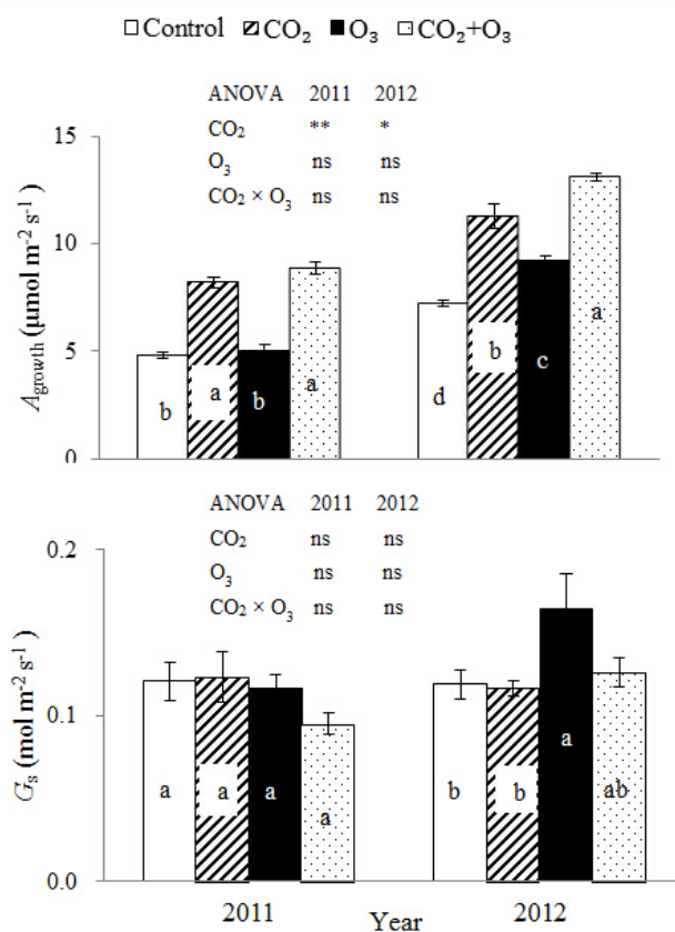
Figure 3.5 Net photosynthetic rate of growth under [CO 2 ] concentrations ( A_{\text{growth}} ) and stomatal conductance ( G_s ). Each value is the mean of four chamber replications, and the vertical bar indicates the standard error. Different character symbol denote significant differences between the four treatments ( P < 0.05 ). ANOVA: * P < 0.05 , ** P < 0.01 , “ns” means not significant.
