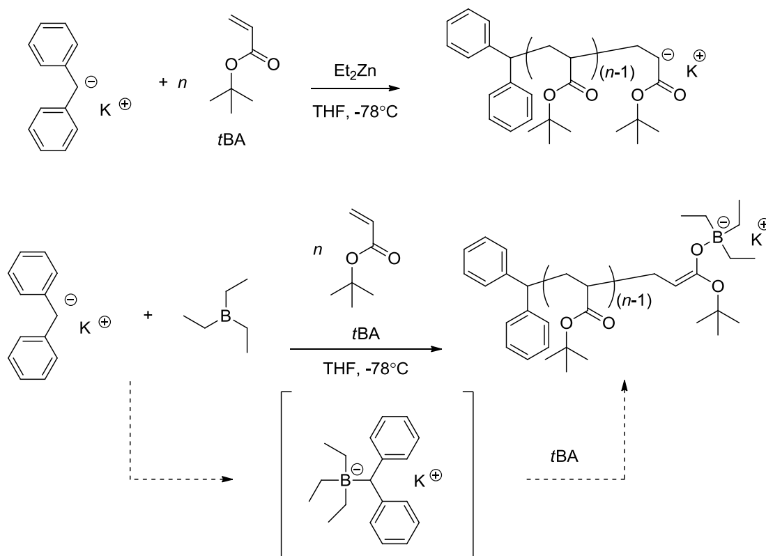
Scheme 1-8. Anionic Polymerization of t BA Initiated by Diphenylmethylanion in the presence of dialkylzinc or triethylborane
