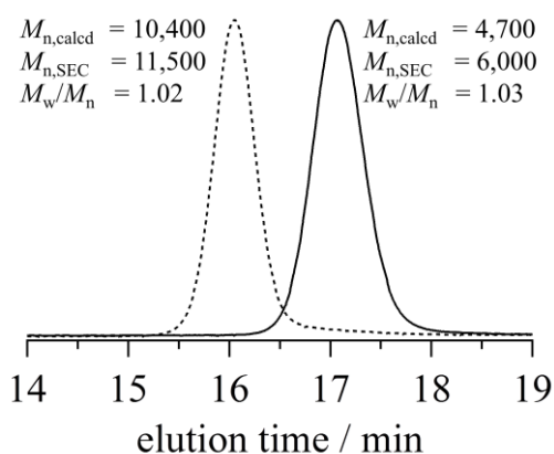
Figure 2-4. SEC traces of the products obtained from the first polymerization (solid line) and the second polymerization (dotted line) in the postpolymerization (eluent, THF; flow rate, 1.0 mL min -1 ).
