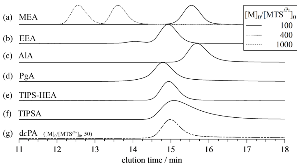
Figure 3-4. SEC traces of the functional acrylate polymers obtained from GTP of (a) MEA, (b) EEA, (c) AIA, (d) PgA, (e) TIPS-HEA, (f) TIPSA, and (G) dcPA (eluent, THF; flow rate, 1.0 mL min -1 ).
