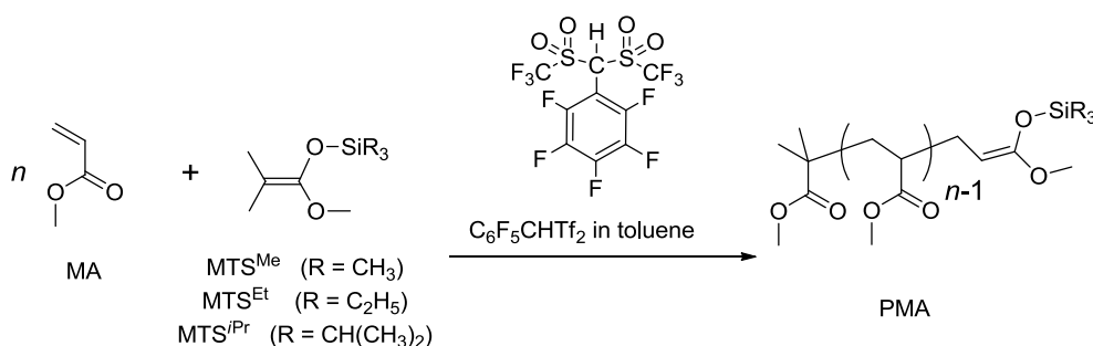
Scheme 2-1. C_6F_5CHTf_2 -Promoted group transfer polymerization (GTP) of methyl acrylate (MA) using MTS^{Me} , MTS^{Et} , and MTS^{iPr}
