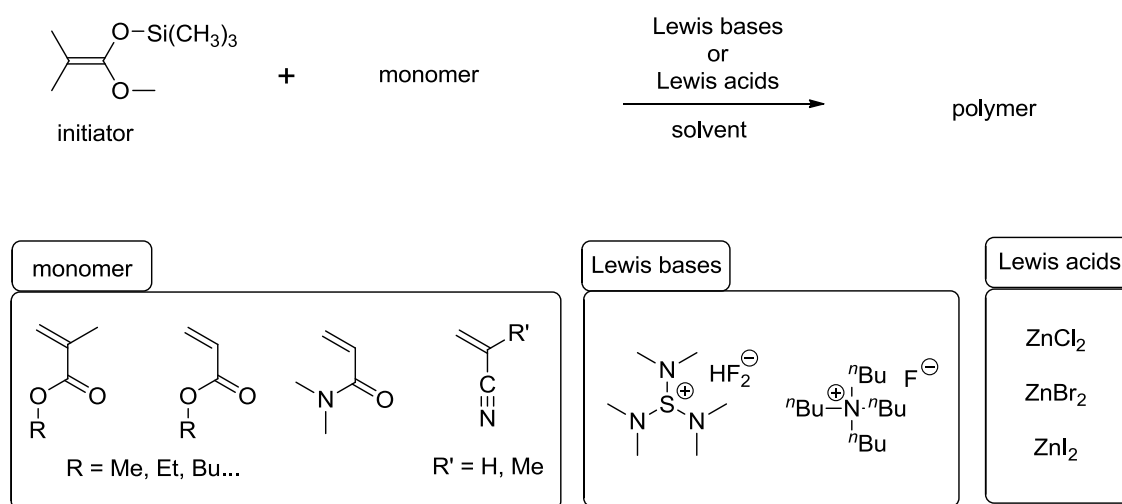
Scheme 1-12. General Schematic of Group Transfer Polymerization (GTP) with Applicable Monomers and Lewis Bases/Acids as Catalysts
