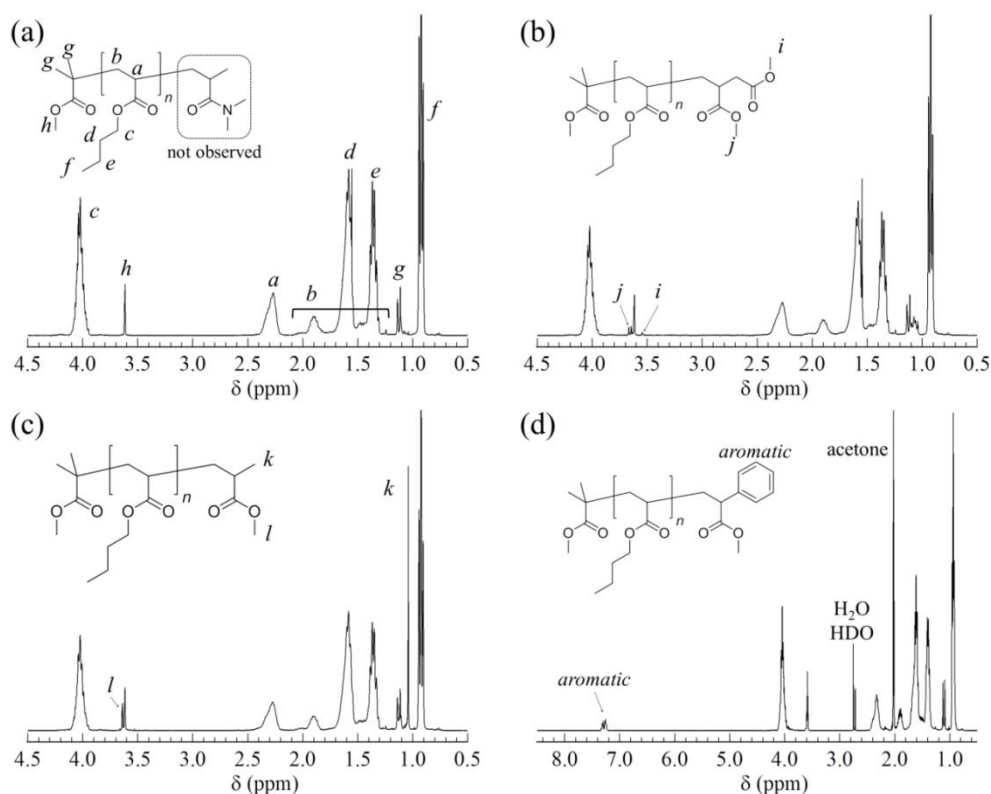
Figure 4-4. 1 H NMR spectra of the ω-functionalized P n BA obtained from termination with (a) DMMAm, (b) DMIIt, (c) MMA, and (d) MPhA (solvent: (a), (b), and (d), CDCl 3 ; (d), acetone- d 6 ).
