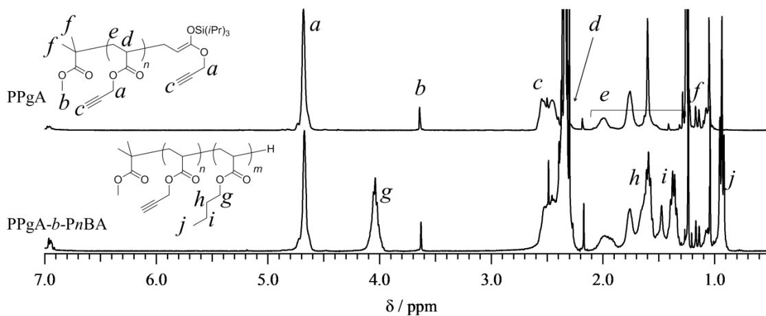
Figure 3-17. ^1\text{H} NMR spectrum of the block copolymers obtained from sequential GTP of PgA and n BA in \text{CDCl}_3 .
