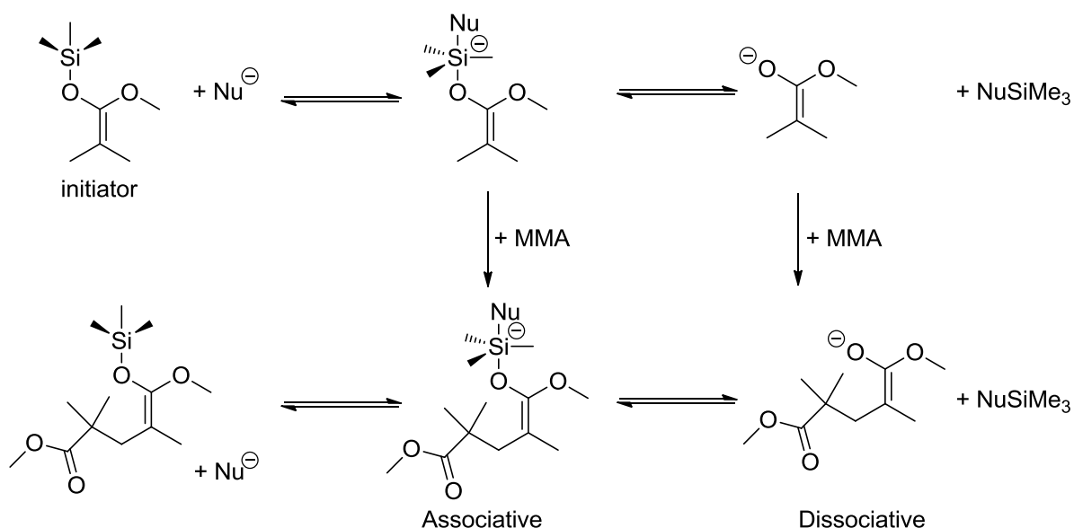
Scheme 1-10. Associative and Dissociative Mechanism of GTP of MMA in the Presence of Nucleophilic Catalyst
