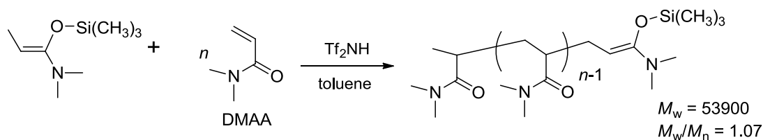
Scheme 1-21. Precise Synthesis of Poly( N,N -dimethylacrylamide)s by \text{TiF}_2\text{NH} -Promoted GTP using Specially Designed Initiator
