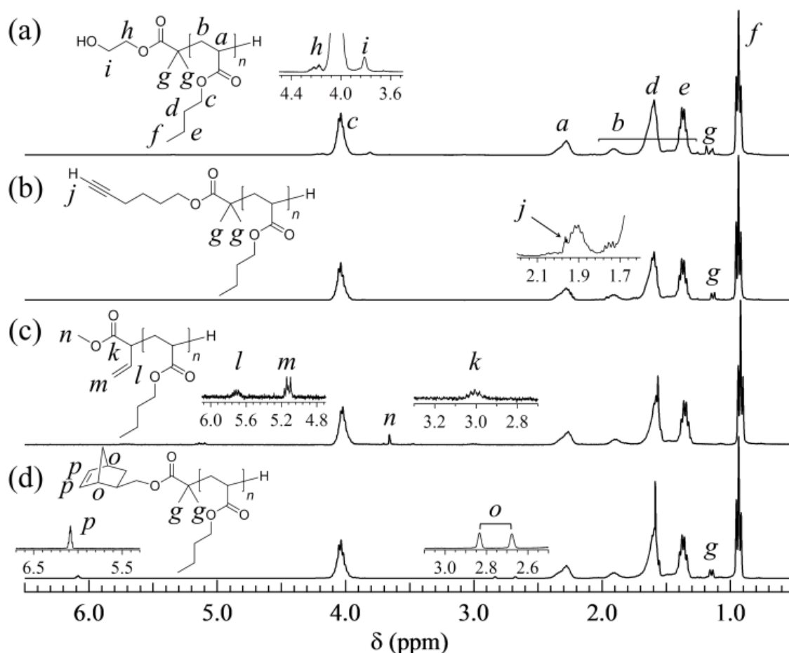
Figure 4-1. 1 H NMR spectra of (a) HO-PnBA, (b) HC \equiv C-PnBA, (c) H 2 C=CH-PnBA, and (d) NB-PnBA prepared by the GTP of n BA using FI-OH, FI-C \equiv CH, FI-CH=CH 2 , and FI-NB, respectively (solvent, CDCl 3 ).
