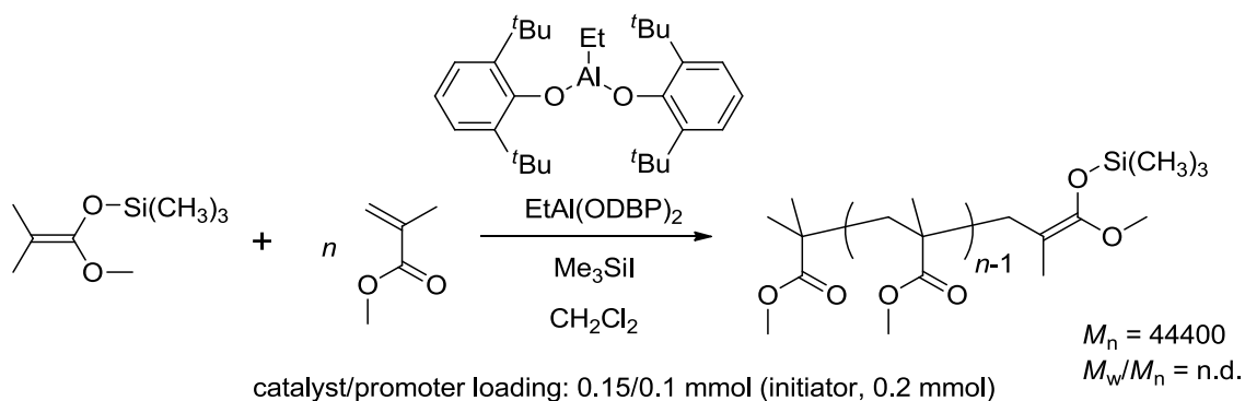
Scheme 1-14. Stereospecific GTP of Methyl Methacrylate using \text{RAl}(\text{OAr})_2/(\text{CH}_3)_3\text{SiI} as Catalyst/Promoter
