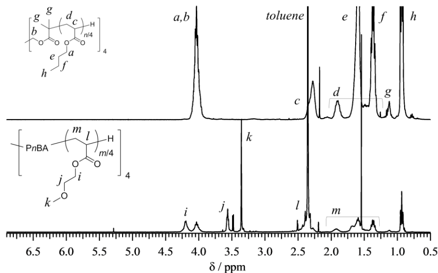
Figure 5-6. ^1\text{H} NMR spectra of the star-shaped PnBA (upper) and PnBA- b -PMEA (lower) in \text{CDCl}_3 at room temperature.
