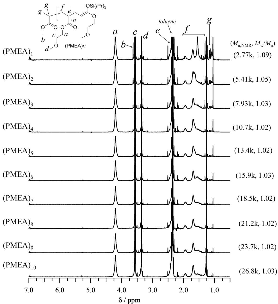
Figure 3-10. ^1\text{H} NMR spectra of the (PMEA)_n obtained from chain extension experiment (solvent, \text{CDCl}_3 ).
