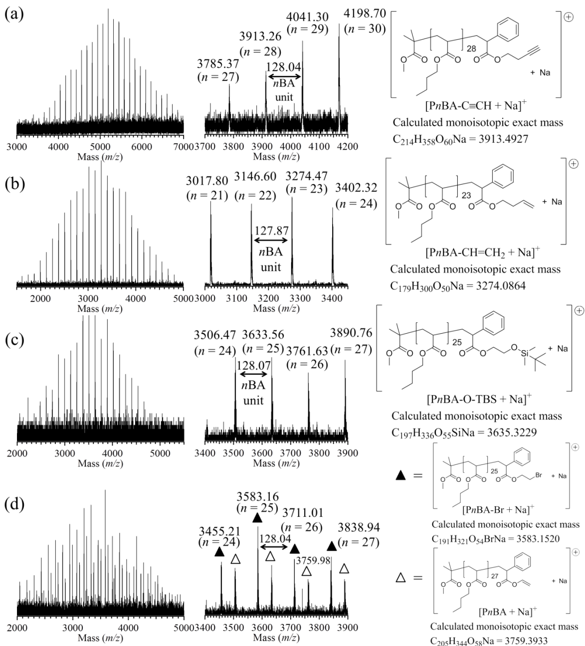
Figure 4-7. MALDI-TOF MS spectra of (a) PnBA-C\equiv CH ( M_{n,NMR} , 3.76 \text{ kg mol}^{-1} and M_w/M_n , 1.06), (b) PnBA-CH=CH_2 ( M_{n,NMR} , 3.64 \text{ kg mol}^{-1} and M_w/M_n , 1.10), (c) PnBA-OH with protecting group ( M_{n,NMR} , 3.71 \text{ kg mol}^{-1} and M_w/M_n , 1.07), and (d) PnBA-Br ( M_{n,NMR} , 3.78 \text{ kg mol}^{-1} and M_w/M_n , 1.10).
