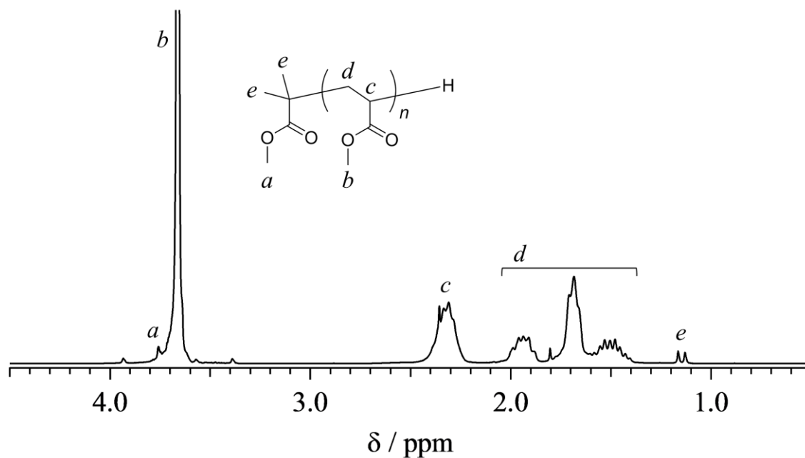
Figure 2-1. ^1\text{H} NMR spectrum of the obtained PMA measured in \text{CDCl}_3 .
