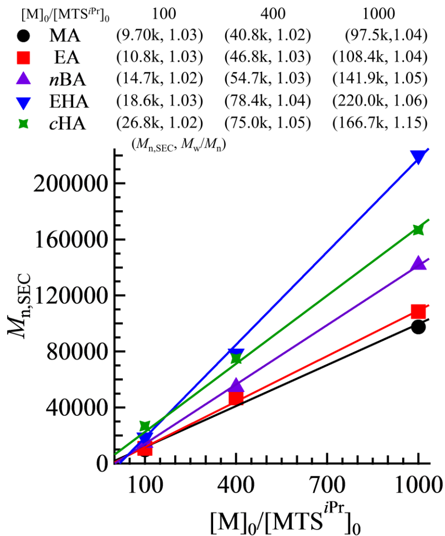
Figure 3-2. Plots for the molecular weights ( M_{n,SEC} ) of the obtained polymers vs. the initial molar ratios of the monomer and initiators ( [M]_0/[MTS^{iPr}]_0 ) MA; EA; n BA; EHA; and cHA along with the values of molecular weight and molecular weight distribution.
