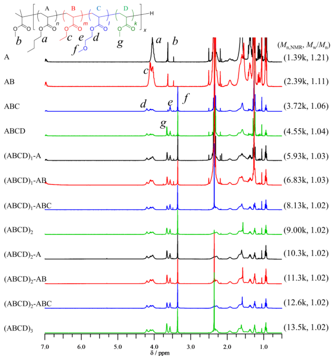
Figure 3-20. ^1\text{H} NMR spectra of the (\text{PnBA-}b\text{-PEA-}b\text{-PMEA-}b\text{-PMA})_3 -block quaterpolymers obtained from chain extension experiment of n BA (A), EA (B), MEA (C), and MA (D) (solvent, \text{CDCl}_3 ).
