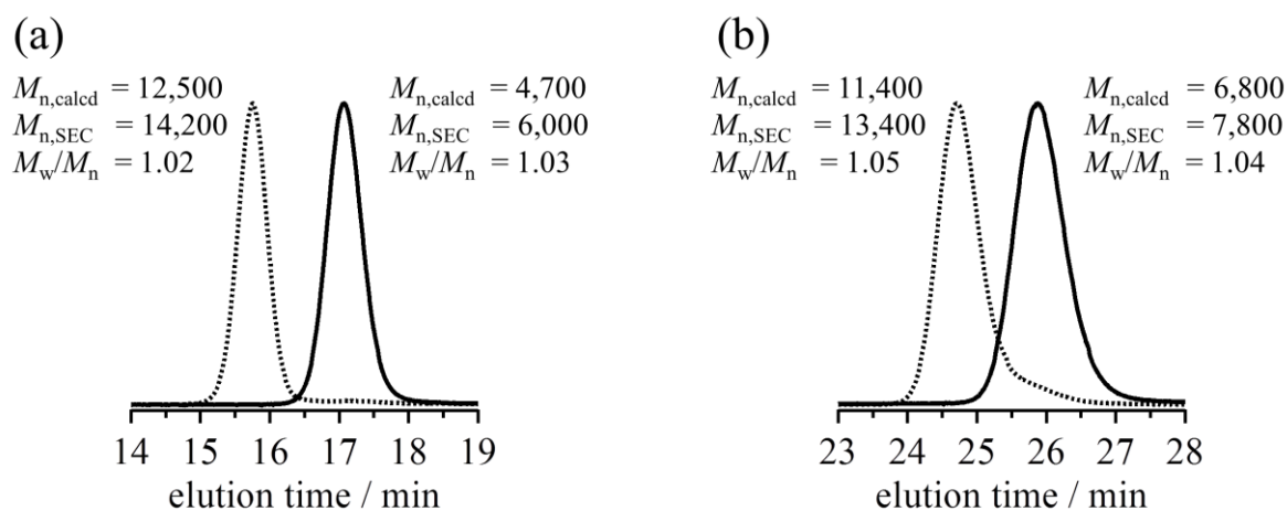
Figure 2-5. SEC traces of the products obtained from the first polymerization (solid line) and the second polymerization (dotted line) in (a) the block copolymerization of MA and n BA, and (b) that of n BA and MA (eluent, THF; flow rate, 1.0 mL min -1 ).
