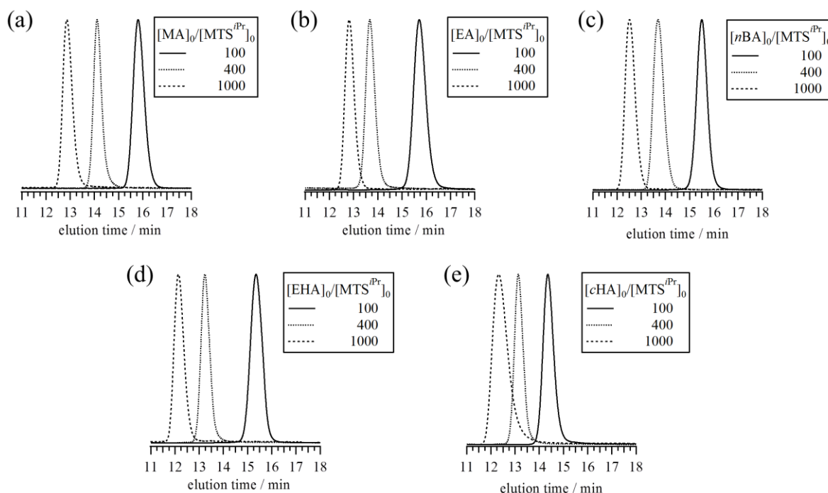
Figure 3-3. SEC traces of the obtained polyacrylates (a) PMA, (b) PEA, (c) n BA, (d), EHA, and (e) cHA (eluent, THF; flow rate, 1.0 mL min -1 ).
