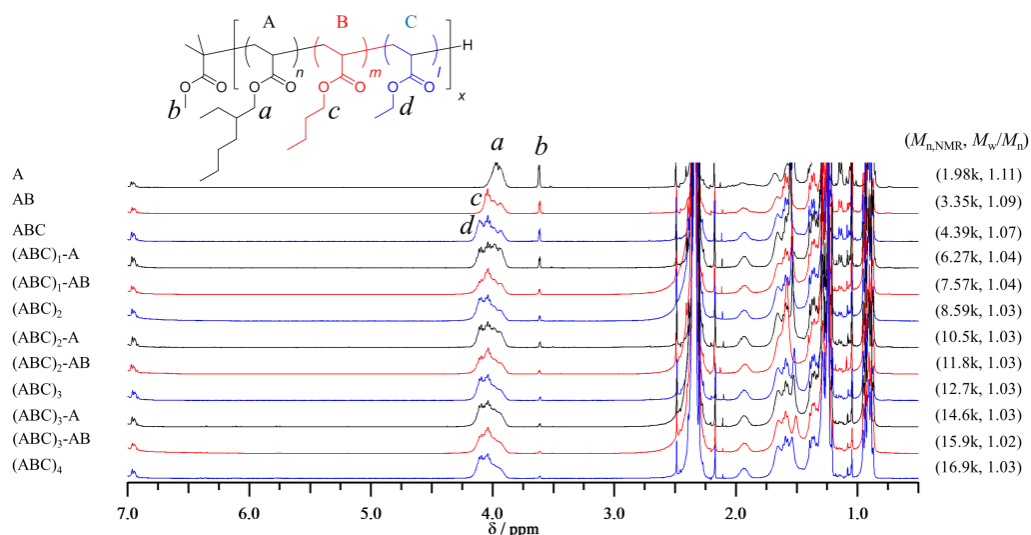
Figure 3-19. ^1\text{H} NMR spectra of the (\text{PEHA-}b\text{-PnBA-}b\text{-PEA})_4 -block terpolymers obtained from chain extension experiment of EHA (A), n BA (B), and EA (C) (solvent, \text{CDCl}_3 ).
