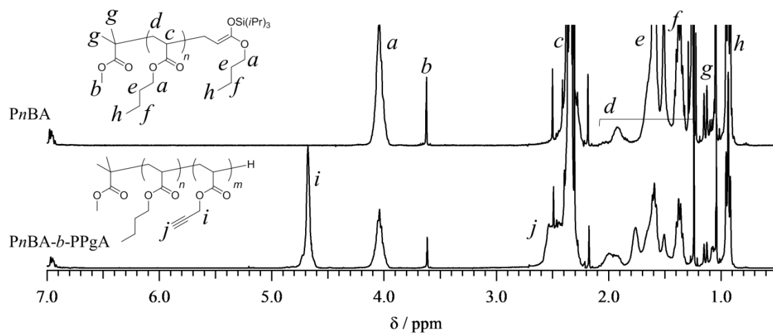
Figure 3-16. ^1\text{H} NMR spectrum of the block copolymers obtained from sequential GTP of n BA and PgA in \text{CDCl}_3 .
