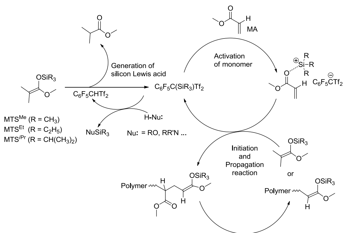
Scheme 2-2. A Proposed Mechanism for the \text{C}_6\text{F}_5\text{CHTf}_2 -Promoted GTP of MA
