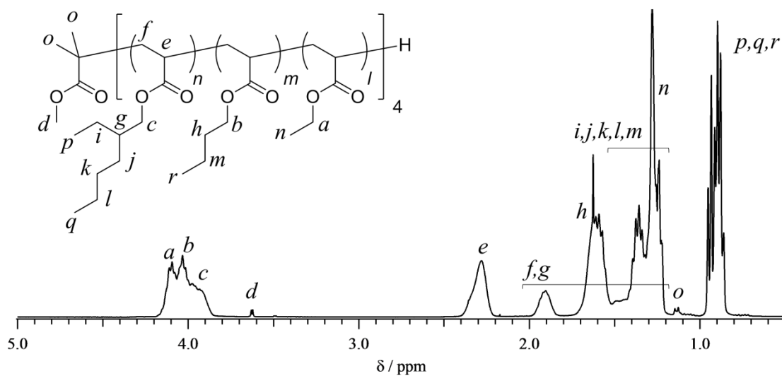
Figure 3-22. ^1\text{H} NMR spectrum of the (\text{PEHA-}b\text{-PnBA-}b\text{-PEA})_4 dodecablock terpolymers obtained from chain extension experiment of EHA, n BA, and EA (solvent, \text{CDCl}_3 ).
