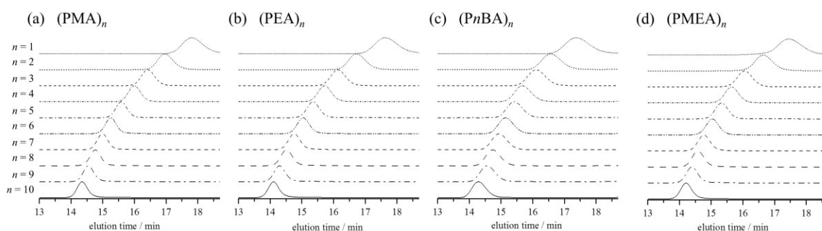
Figure 3-6. SEC traces of (a) (PMA) _n , (b) (PEA) _n , (c) (PnBA) _n , and (d) (PMEA) _n obtained from the sequential GTPs of MA, EA, n BA, and MEA (eluent, THF; flow rate, 1.0 mL min -1 ).
