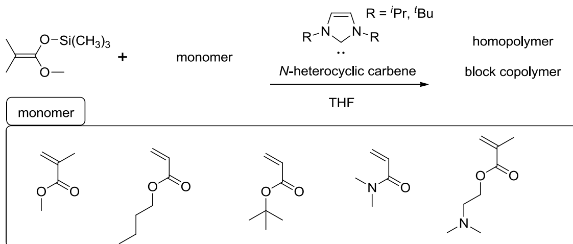
Scheme 1-16. Synthesis of Various Homopolymers and Block Copolymers using N -Heterocyclic Carbene-catalyzed GTP
