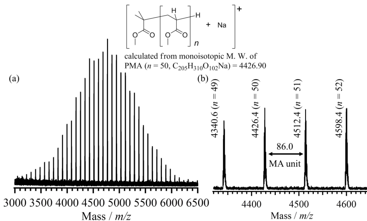
Figure 2-2. MALDI-TOF MS spectrum (reflector mode) of the obtained PMA ( [\text{MA}]_0/[\text{MTS}^{\text{iPr}}]_0/[\text{C}_6\text{F}_5\text{CHTf}_2]_0 , 50/1/0.02, conversion > 99%, M_{n,\text{SEC}} , 5800; M_w/M_n , 1.05).
