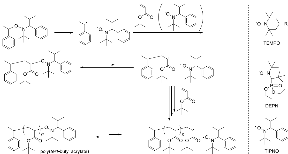
Scheme 1-2. The General Mechanism of NMP using TIPNO-type Nitroxide as an Initiator
