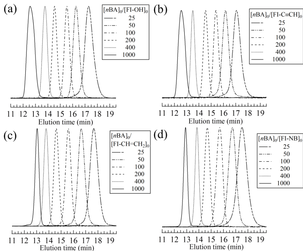
Figure 4-3. SEC traces of (a) HO-PnBA, (b) HC≡C-PnBA, (c) H 2 C=CH-PnBA, and (d) NB-PnBA obtained from GTP of n BA using functional initiators (eluent, THF; flow rate, 1.0 mL min -1 ).
