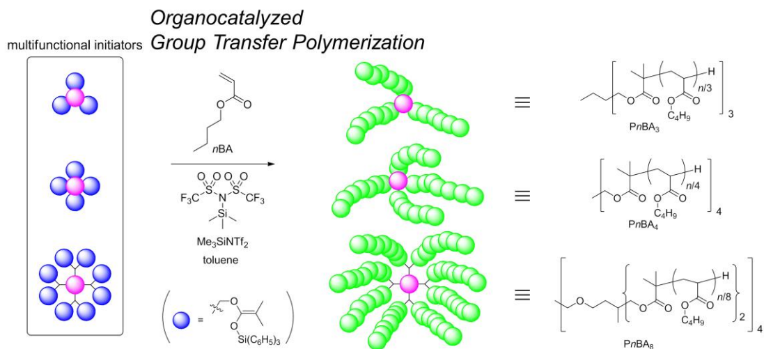
Figure 1-6. Synthesis of three-, four-, and eight-armed star-shaped poly( n -butyl acrylate), \text{PnBA}_3 , \text{PnBA}_4 , and \text{PnBA}_8 , by \text{Me}_3\text{SiNTf}_2 -catalyzed GTP using multifunctional initiators.
