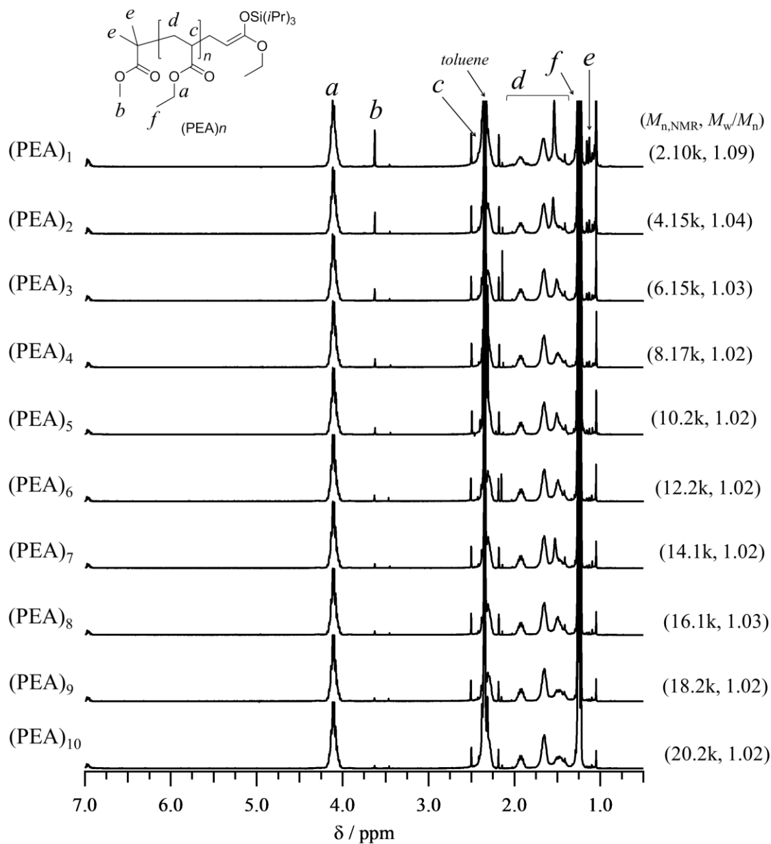
Figure 3-8. ^1\text{H} NMR spectra of the (PEA)_n obtained from chain extension experiment (solvent, \text{CDCl}_3 ).
