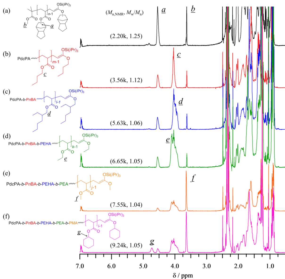
Figure 3-21. ^1\text{H} NMR spectra of the hexablock sestopolymer obtained by sequential \text{Me}_3\text{SiNTf}_2 -catalyzed GTP; (a) PdcPA, (b) PdcPA- b -PnBA, (c) PdcPA- b -PnBA- b -PEHA, (d) PdcPA- b -PnBA- b -PEHA- b -PEA, (e) PdcPA- b -PnBA- b -PEHA- b -PEA- b -PMA, and (f) PdcPA- b -PnBA- b -PEHA- b -PEA- b -PMA- b -PcHA (solvent, \text{CDCl}_3 ).
