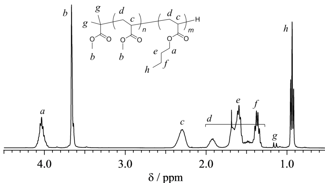
Figure 2-6. ^1\text{H} NMR spectrum of the obtained poly(methyl acrylate)- block -poly( n -butyl acrylate) measured in \text{CDCl}_3 .
