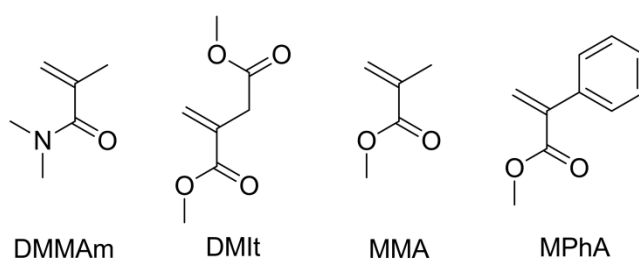
Chart 4-1. Terminators for the \text{Me}_3\text{SiNTf}_2 -Catalyzed GTP of n BA
