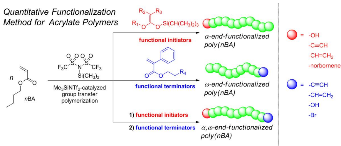
Figure 1-5. Synthesis of \alpha -, \omega -, and \alpha,\omega -end-functionalized acrylate polymers by organocatalyzed GTP through the initiation and termination approaches using functional initiators and terminators.
