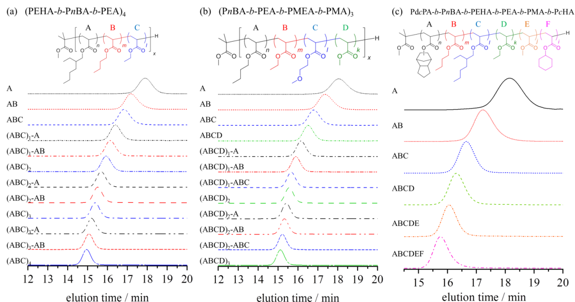
Figure 3-18. SEC traces for the synthesis of (a) (\text{PEHA-}b\text{-PnBA-}b\text{-PEA})_4 dodecablock terpolymer, (b) (\text{PnBA-}b\text{-PEA-}b\text{-PMEA-}b\text{-PMA})_3 dodecablock quaterpolymer, and (c) \text{PdcPA-}b\text{-PnBA-}b\text{-PEHA-}b\text{-PEA-}b\text{-PMA-}b\text{-PcHA} hexablock sestopolymer (eluent, THF; flow rate, 1.0 \text{ mL min}^{-1} ).
