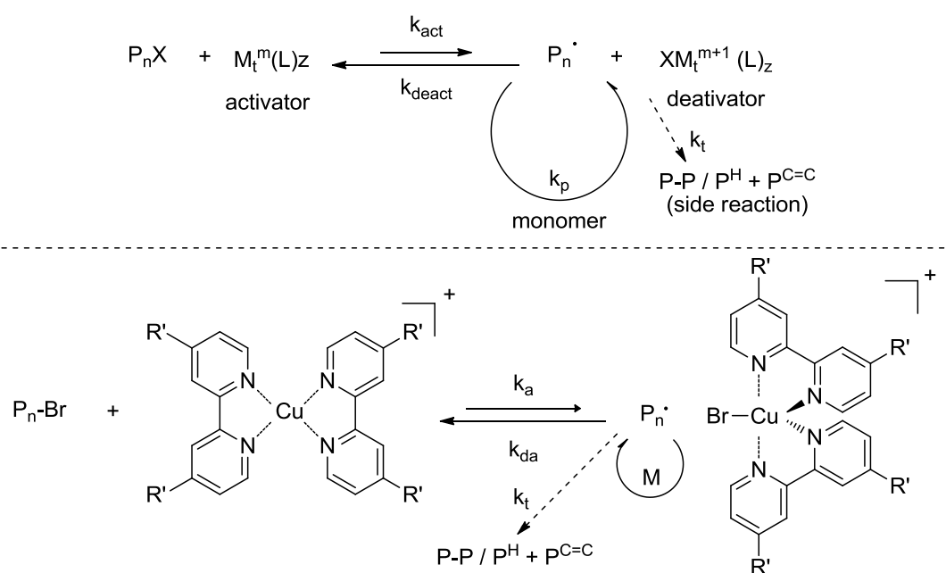
Scheme 1-3. The General Mechanism of ATRP
