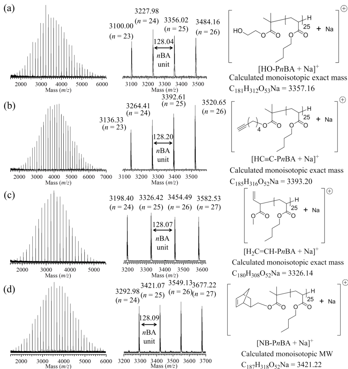
Figure 4-2. MALDI-TOF MS spectra of (a) HO-PnBA ( M_{n,\text{NMR}} , 3.41 \text{ kg mol}^{-1} and M_w/M_n , 1.10), (b) HC≡C-PnBA ( M_{n,\text{NMR}} , 3.69 \text{ kg mol}^{-1} and M_w/M_n , 1.10), (c) H 2 C=CH-PnBA ( M_{n,\text{NMR}} , 3.48 \text{ kg mol}^{-1} and M_w/M_n , 1.07), and (d) NB-PnBA ( M_{n,\text{NMR}} , 3.57 \text{ kg mol}^{-1} and M_w/M_n , 1.10).
