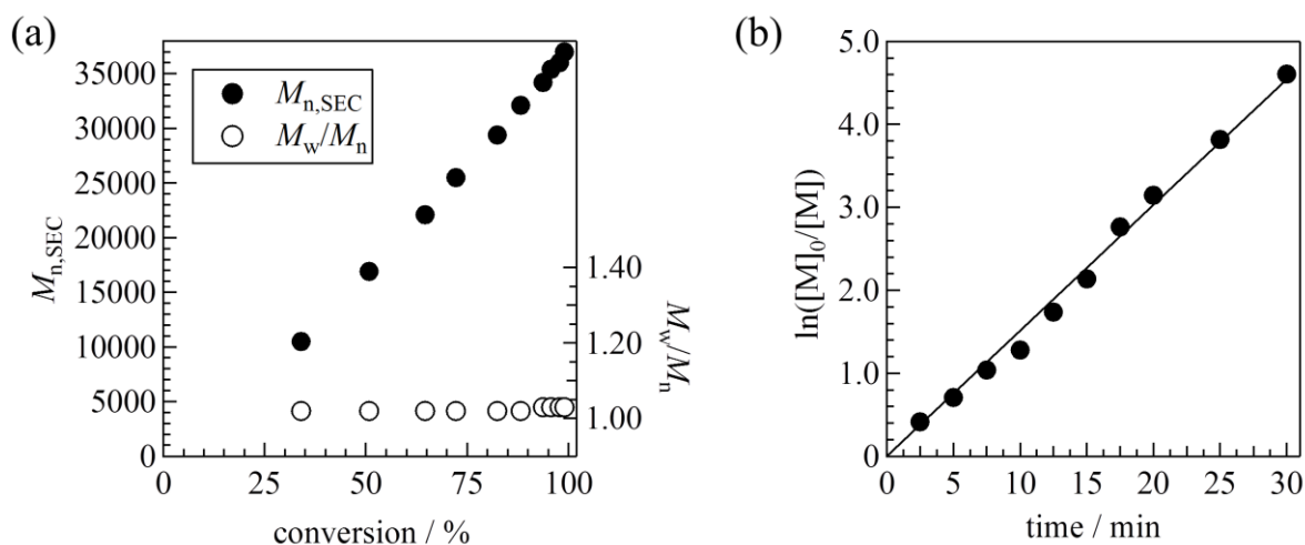
Figure 2-3. (a) Dependence of molecular weight ( M_{n,\text{SEC}} ) and polydispersity ( M_w/M_n ) on the monomer conversion and (b) first-order kinetic plots for the GTP of MA in toluene at 27^\circ\text{C} ( [\text{MA}]_0, 1.0 \text{ mol L}^{-1} ; [\text{MA}]_0/[\text{MTS}^{\text{iPr}}]_0/[\text{C}_6\text{F}_5\text{CHTf}_2]_0, 400/1/0.02 ).
