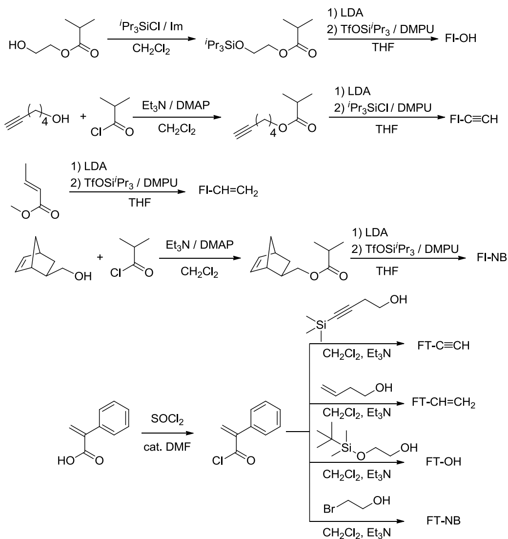
Scheme 4-2. Synthesis of Functional Initiators and Terminators of FI-OH, FI-C≡CH, FI-CH=CH 2 , FI-NB, FT-C≡CH, FT-CH=CH 2 , FT-OH, and FT-Br
