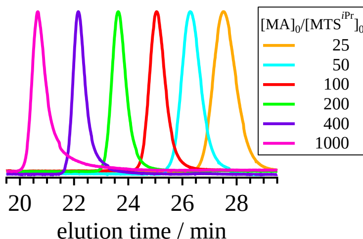
Figure 2-7. SEC traces of the obtained PMAs (eluent, THF; flow rate, 1.0 mL min -1 ).
