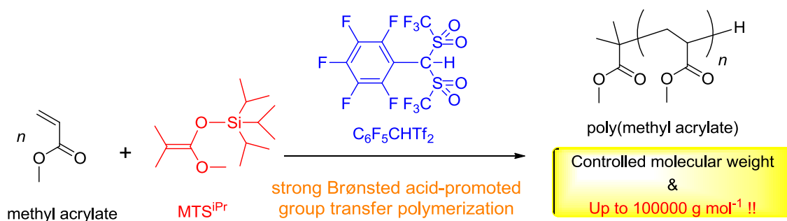
Figure 1-3. Synthesis of high-molecular-weight acrylate polymers by strong Brønsted acid-promoted GTP.
