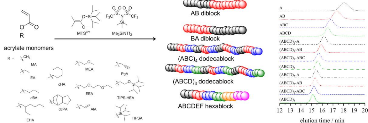
Figure 1-4. Synthesis of AB/BA diblock, (\text{ABC})_4 dodecablock, (\text{ABCD})_3 dodecablock, and ABCDEF hexablock polymers by organocatalyzed GTP using \text{MTS}^{\text{iPr}} as an initiator.
