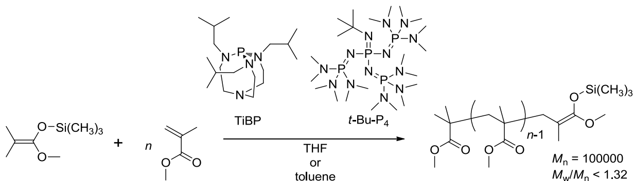
Scheme 1-17. Phosphazene Base-Catalyzed GTP of Methyl Methacrylate
