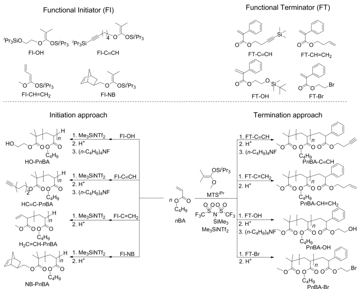
Scheme 4-1. Synthesis of \alpha - and \omega -End-Functionalized Poly( n -butyl acrylate)s (P n BA)s by N -(Trimethylsilyl)bis(trifluoromethanesulfonyl)imide ( \text{Me}_3\text{SiNTf}_2 )-Catalyzed Group Transfer Polymerization of n -Butyl Acrylate ( n BA) using Functional Initiator (FI) and Terminator (FT)
