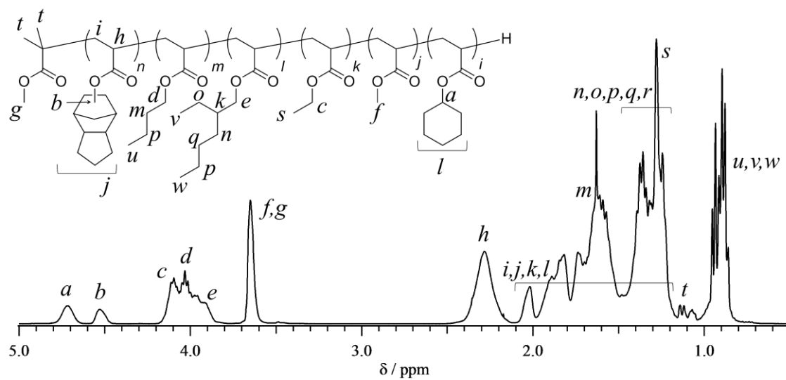
Figure 3-24. ^1\text{H} NMR spectram of the PdcPA- b -PnBA- b -PEHA- b -PEA- b -PMA- b -PcHA hexablock sesterpolymers obtained from chain extension experiment of dcPA, n BA, EHA, EA, MA, and cHA (solvent, \text{CDCl}_3 ).
