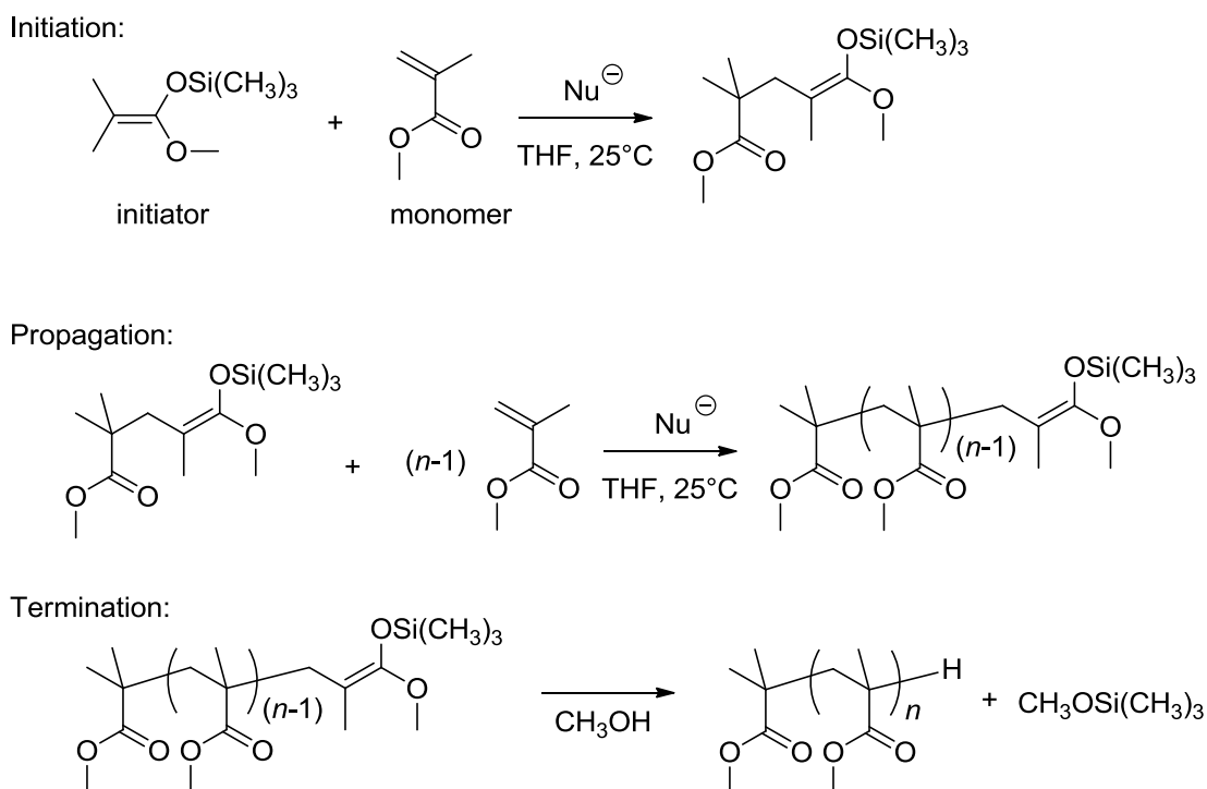
Scheme 1-9. GTP of MMA with Nucleophilic Catalysts
