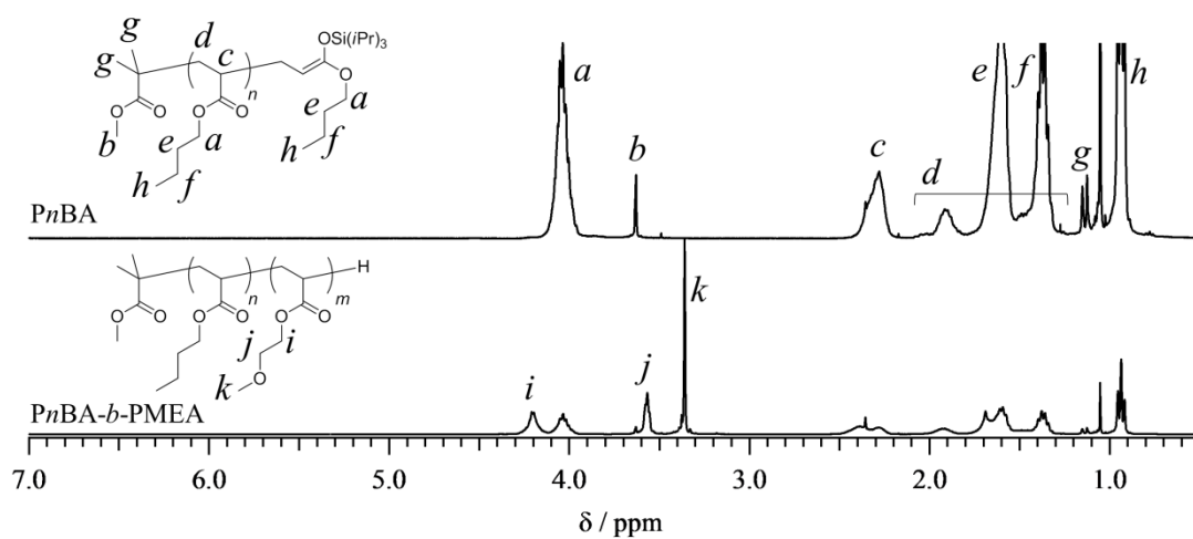
Figure 3-12. ^1\text{H} NMR spectrum of the block copolymers obtained from sequential GTP of n BA and MEA in \text{CDCl}_3 .
