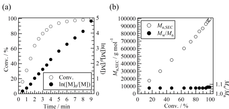
Figure 5-3. (a) Zero-order (○) and first-order (●) kinetic plots of \text{Me}_3\text{SiNTf}_2 -catalyzed GTP of n\text{BA} in toluene at 27 °C under conditions of [nBA]_0/[\text{MTS}^{\text{Ph}}_4]_0/[\text{Me}_3\text{SiNTf}_2]_0 , 800/1/0.05 and [nBA]_0 , 1.0 mol L ^{-1} and (b) relationship among the monomer conversion (Conv.), number average molecular weight ( M_{n,\text{SEC}} ) (○) and molecular weight distributions ( M_w/M_n ) (●).
