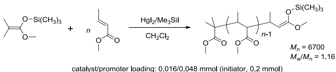
Scheme 1-13. GTP of Methyl Crotonate using \text{HgI}_2/(\text{CH}_3)_3\text{SiI} as Catalyst and Promoter
