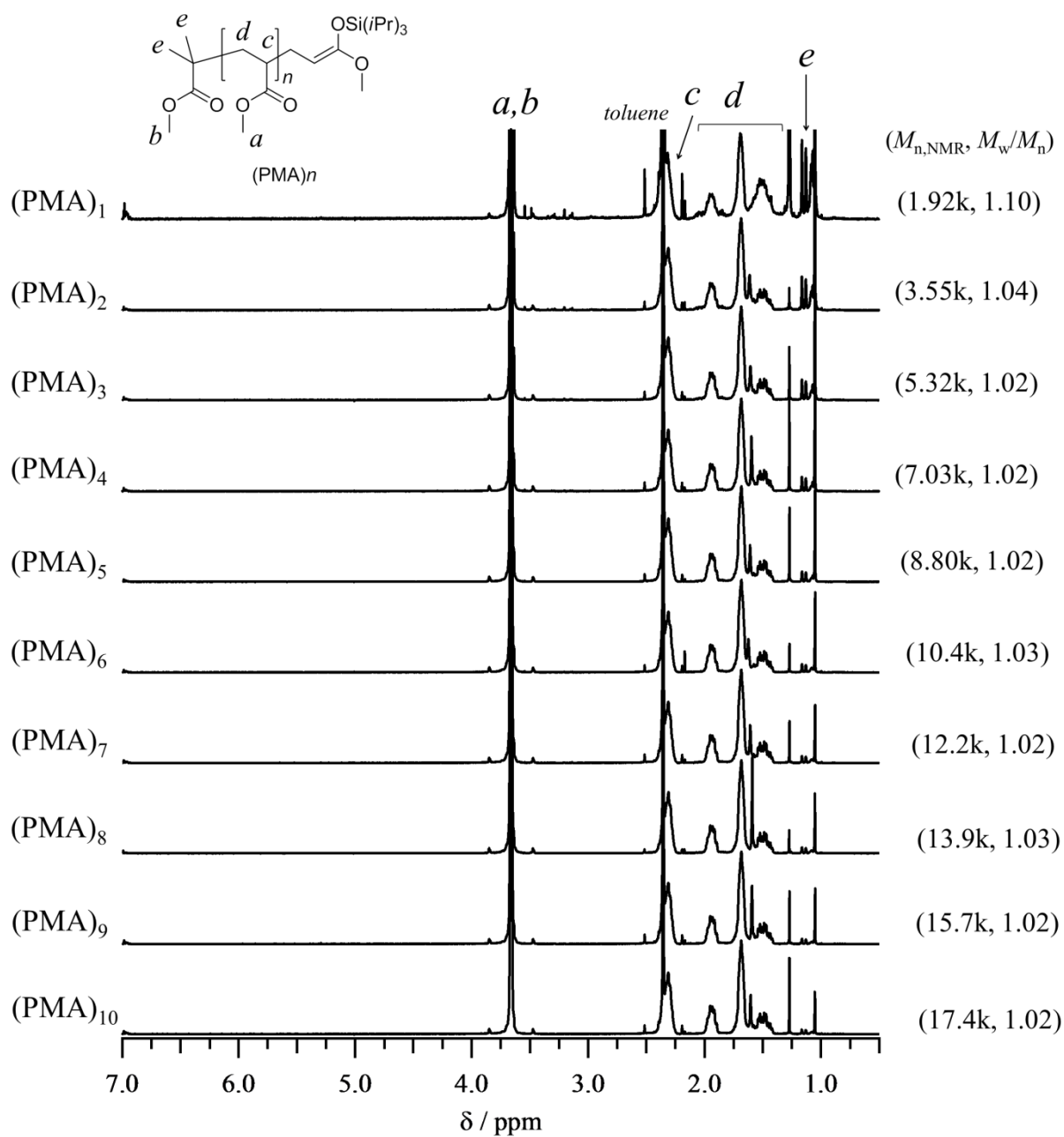
Figure 3-7. ^1H NMR spectra of the (PMA)_n obtained from chain extension experiment (solvent, CDCl_3 ).
