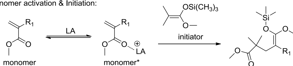
Scheme 1-11. Mechanism of the Lewis Acid (LA)-Catalyzed GTP
