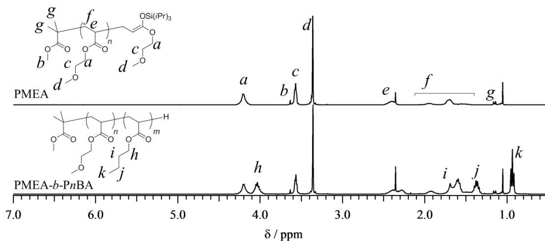
Figure 3-13. ^1\text{H} NMR spectrum of the block copolymers obtained from sequential GTP of MEA and n BA in \text{CDCl}_3 .
