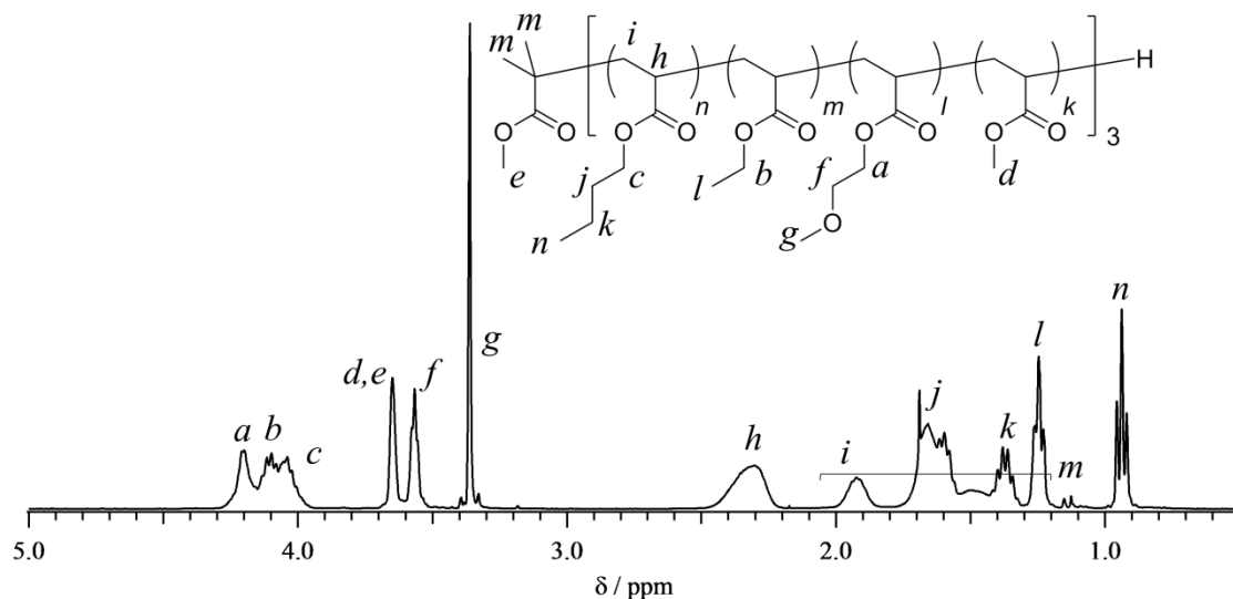
Figure 3-23. ^1\text{H} NMR spectrum of the (\text{PnBA-}b\text{-PEA-}b\text{-PMEA-}b\text{-PMA})_3 dodecablock quintopolymers obtained from chain extension experiment of n BA, EA, MEA, and MA (solvent, \text{CDCl}_3 ).
