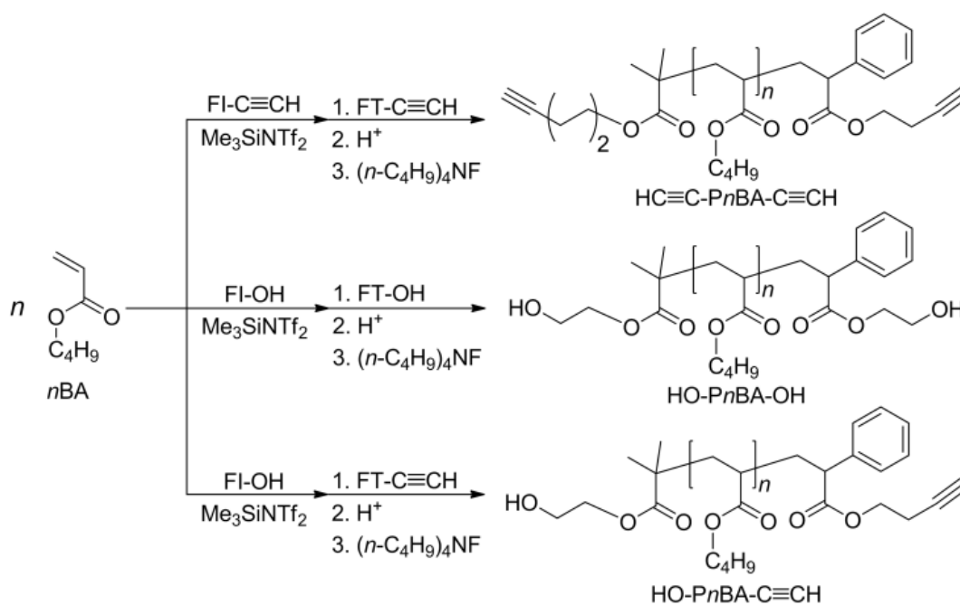
Scheme 4-3. Synthesis of \alpha,\omega -End-Functionalized PnBAs by GTP of n BA using Functional Initiators (FIs) and Terminators (FTs)
