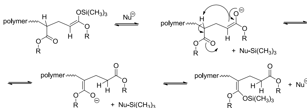
(b) C-O isomerization (acrylate monomer)
