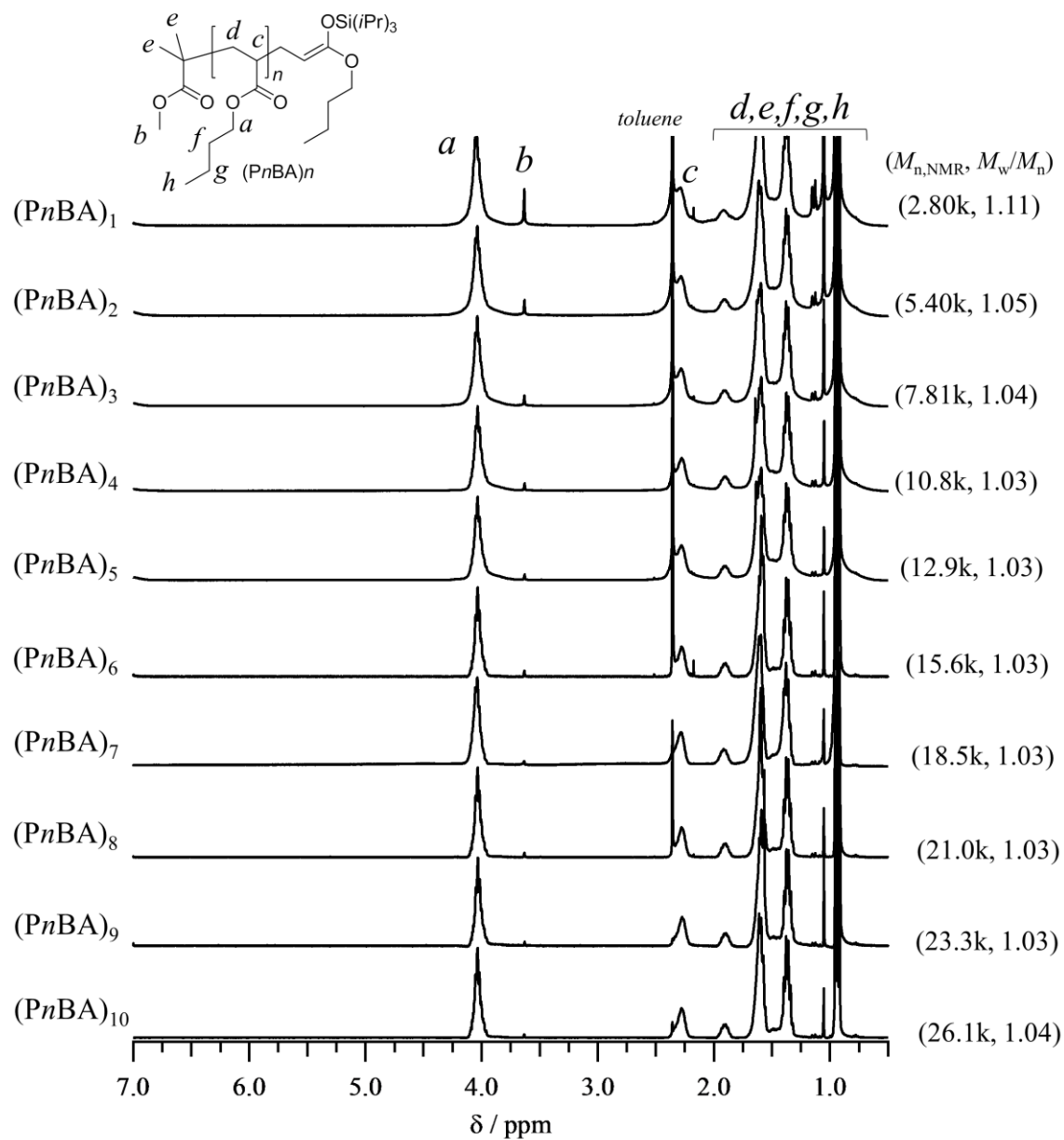
Figure 3-9. ^1H NMR spectra of the (PnBA)_n obtained from chain extension experiment (solvent, CDCl_3 ).
