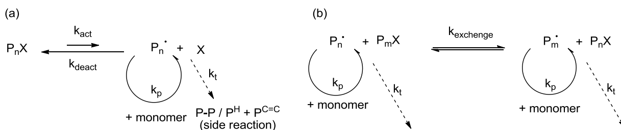
Scheme 1-1. Mechanism of the Controlled/living Radical Polymerization
