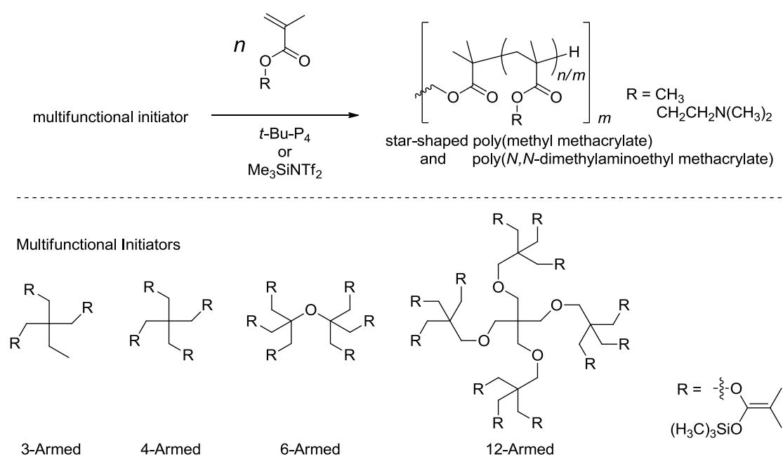
Scheme 1-24. Synthesis of Three-, Four-, Six-, and Twelve-armed Star-Shaped Methacrylate Polymers by the t -Bu-P 4 - or Me 3 SiNTf 2 -Catalyzed GTP with Core-First Method
