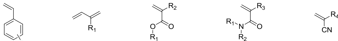
Chart 1-1. Applicable Monomers for Anionic Polymerization and Propagating Anions of Corresponding Monomers
