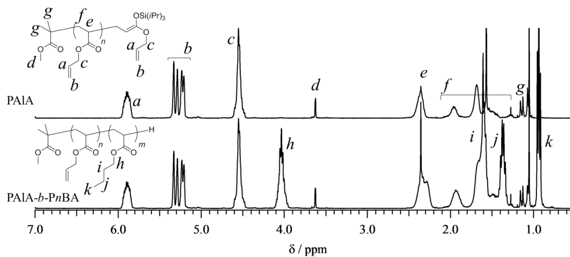
Figure 3-15. ^1\text{H} NMR spectrum of the block copolymers obtained from sequential GTP of AIA and n BA in \text{CDCl}_3 .
