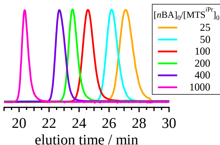
Figure 2-8. SEC traces of the obtained PnBAs (eluent, THF; flow rate, 1.0 mL min -1 ).
