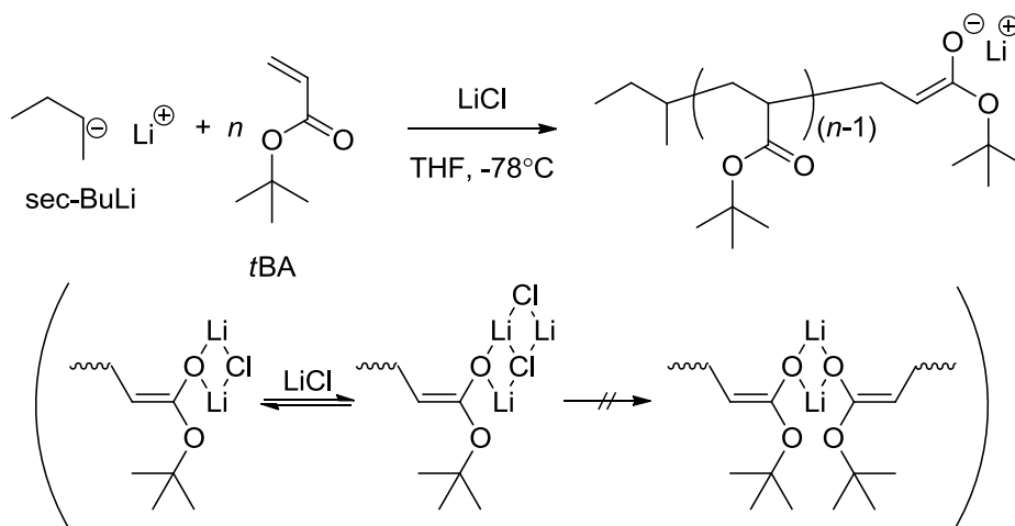
Scheme 1-7. Anionic Polymerization of tert -Butyl Acrylate ( t BA) Initiated by sec -Butyllithium ( sec -BuLi) in the Presence of Lithium Chloride (LiCl) in THF
