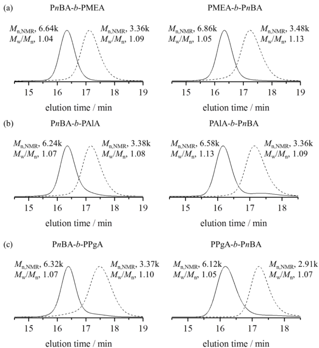
Figure 3-11. SEC traces of the diblock copolymers of (a) n BA and MEA, (b) n BA and AlA, and (c) n BA and PgA ( [M_{first} + M_{second}]_0/[MTS^{iPr}]_0/[Me_3SiNTf_2]_0 , 25+25/1/0.02; [M]_0 , 1.0 mol L -1 ) (dashed line, first polymer; solid line, block copolymer; eluent, THF; flow rate, 1.0 mL min -1 ).
