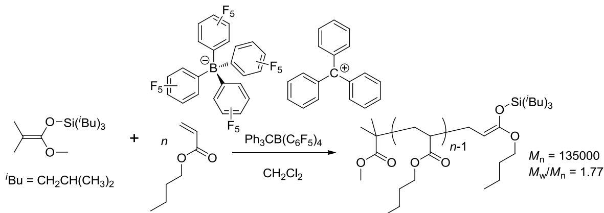
Scheme 1-20. GTP of n -Butyl Acrylate using \text{Ph}_3\text{CB}(\text{C}_6\text{F}_5)_4 as a Catalyst and Triisobutylsilyl Ketene Acetal as an Initiator
