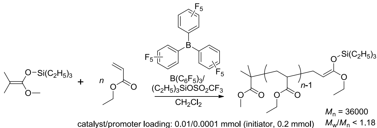
Scheme 1-15. GTP of Ethyl Acrylate using B(C_6F_5)_3/(C_2H_5)_3SiOSO_2CF_3 as Catalyst/Promoter
