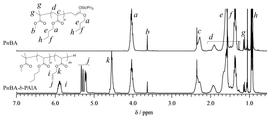
Figure 3-14. ^1\text{H} NMR spectrum of the block copolymers obtained from sequential GTP of n BA and AIA in \text{CDCl}_3 .
