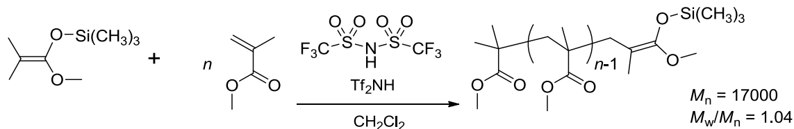
Scheme 1-18. Trifluoromethanesulfonimide (Tf 2 NH)-Promoted GTP of Methyl Methacrylate
