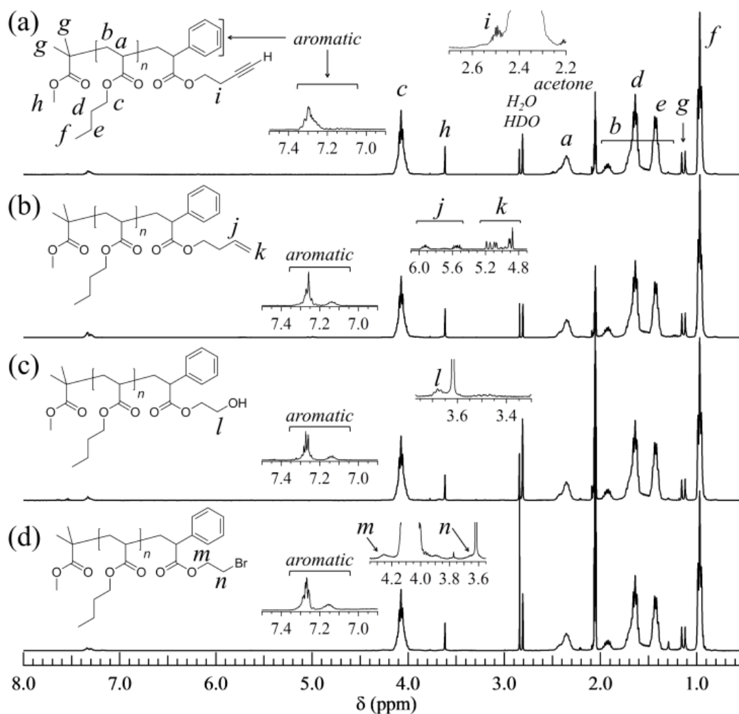
Figure 4-6. ^1\text{H} NMR spectrum of PnBAs obtained from GTP of n BA terminated by (a) FT-C \equiv CH, (b) FT-CH=CH _2 , (c) FT-OH, and (d) FT-Br (solvent, acetone- d_6 ).
