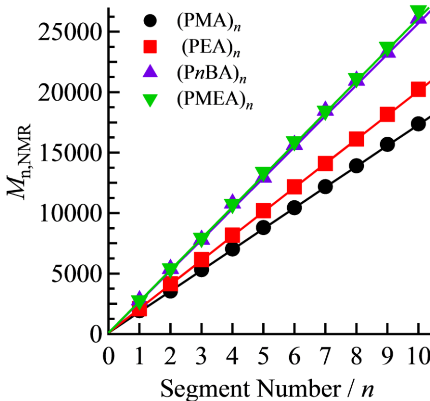
Figure 3-5. Chain extensions of MA, EA, n BA, and MEA produced by the sequential GTPs (PMA (●), PEA (■), PnBA (▲), and PMEA (▼)).
