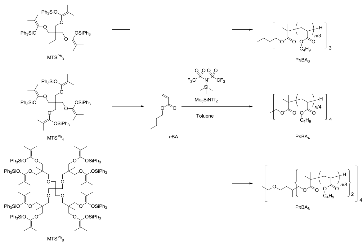
Scheme 5-1. Synthesis of Three-, Four-, and Eight-Armed Star-Shaped Poly( n -butyl acrylate)s, PnBA_3 , PnBA_4 , and PnBA_8 by the Me_3SiNTf_2 -Catalyzed GTP of n BA Using Multifunctional Initiators
