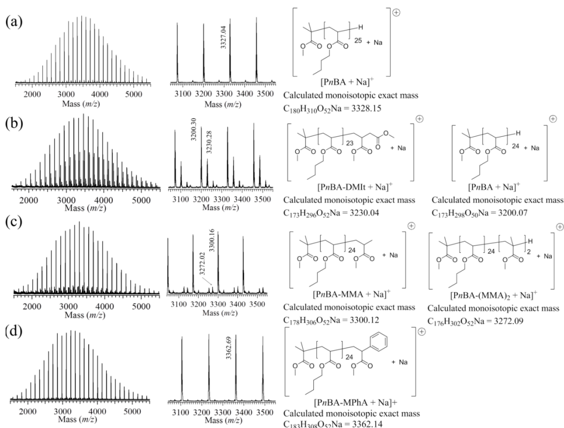
Figure 4-5. MALDI-TOF MS spectra of the obtained PnBA using (a) DMMAm, (b) DMIt, (c) MMA, and (d) MPhA as terminating agents for the Me_3SiNTf_2 -catalyzed GTP of n BA.
