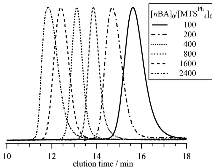
Figure 5-4. SEC traces of the obtained PnBA 4 s (eluent, THF; flow rate, 1.0 mL min -1 ).
