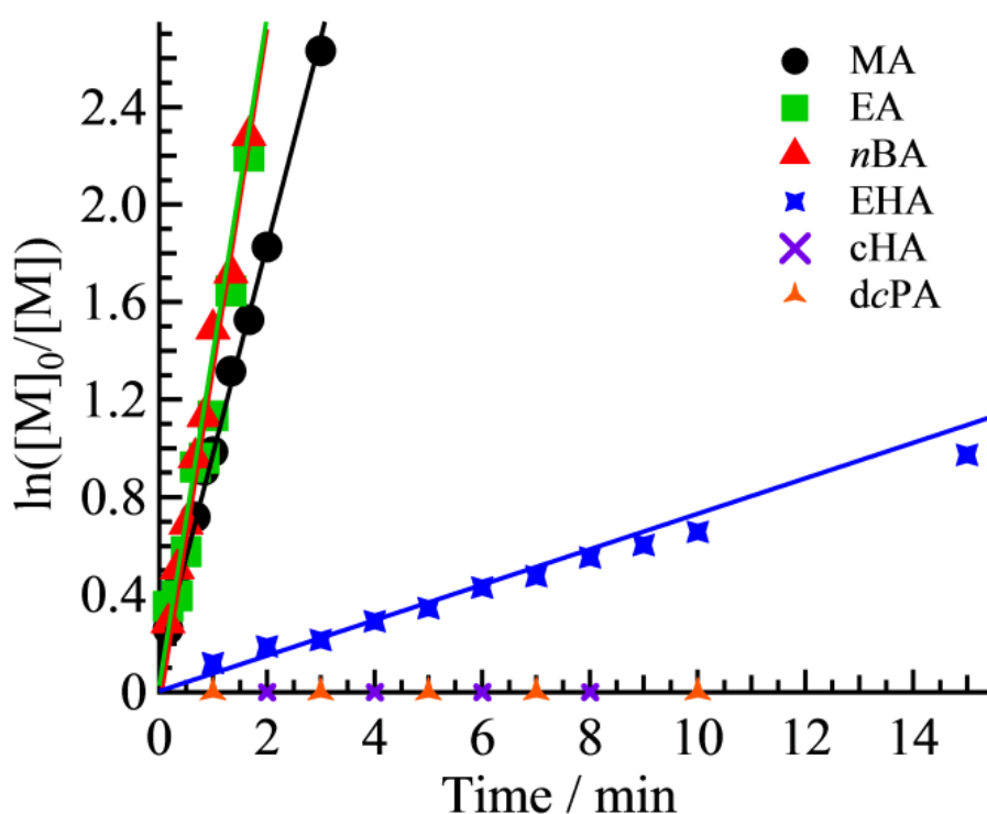
Figure 3-1. Kinetic plots for the \text{Me}_3\text{SiNTf}_2 -catalyzed GTP of MA, EA, n BA, EHA, c HA, and dc PA using \text{MTS}^{\text{iPr}} in toluene ( [\text{M}]_0/[\text{MTS}^{\text{iPr}}]_0/[\text{Me}_3\text{SiNTf}_2]_0 , 200/1/0.02; [\text{M}]_0 , 1.0 mol \text{L}^{-1} ; temperature, 27 °C).
