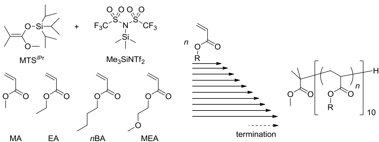
Scheme 3-2. Chain Extension Experiments of MA, EA, nBA, and MEA by \text{Me}_3\text{SiNTf}_2 -Catalyzed GTP
