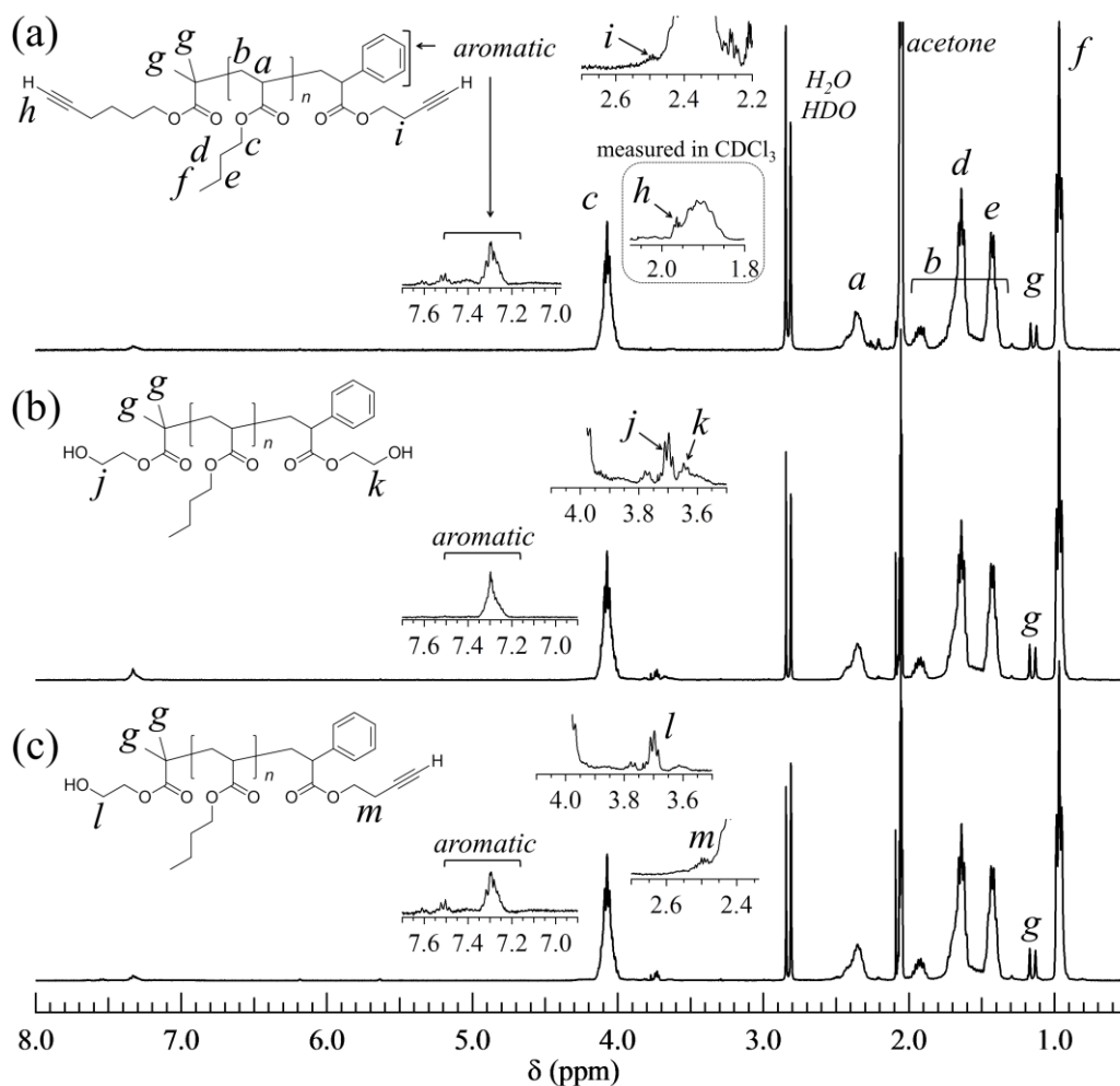
Figure 4-8. ^1\text{H} NMR spectrum of the PnBAs obtained from GTP of n BA using functional initiator and terminator (a) FI- \text{C}\equiv\text{CH} and FT- \text{C}\equiv\text{CH} , (b) FI-OH and FT-OH, and (c) FI-OH and FT- \text{C}\equiv\text{CH} , (solvent, acetone- d_6 ).
