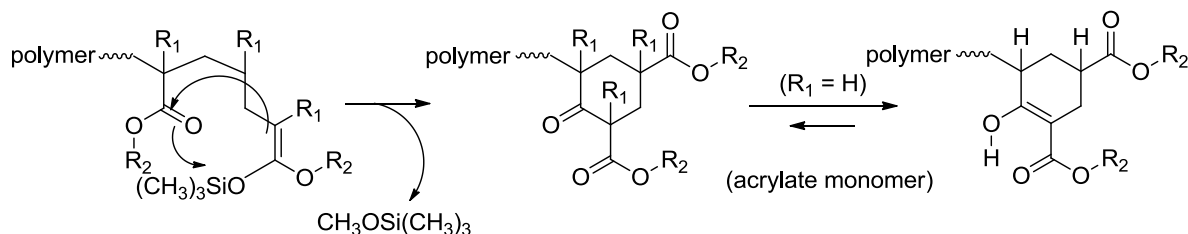
(a) Backbiting Reaction
