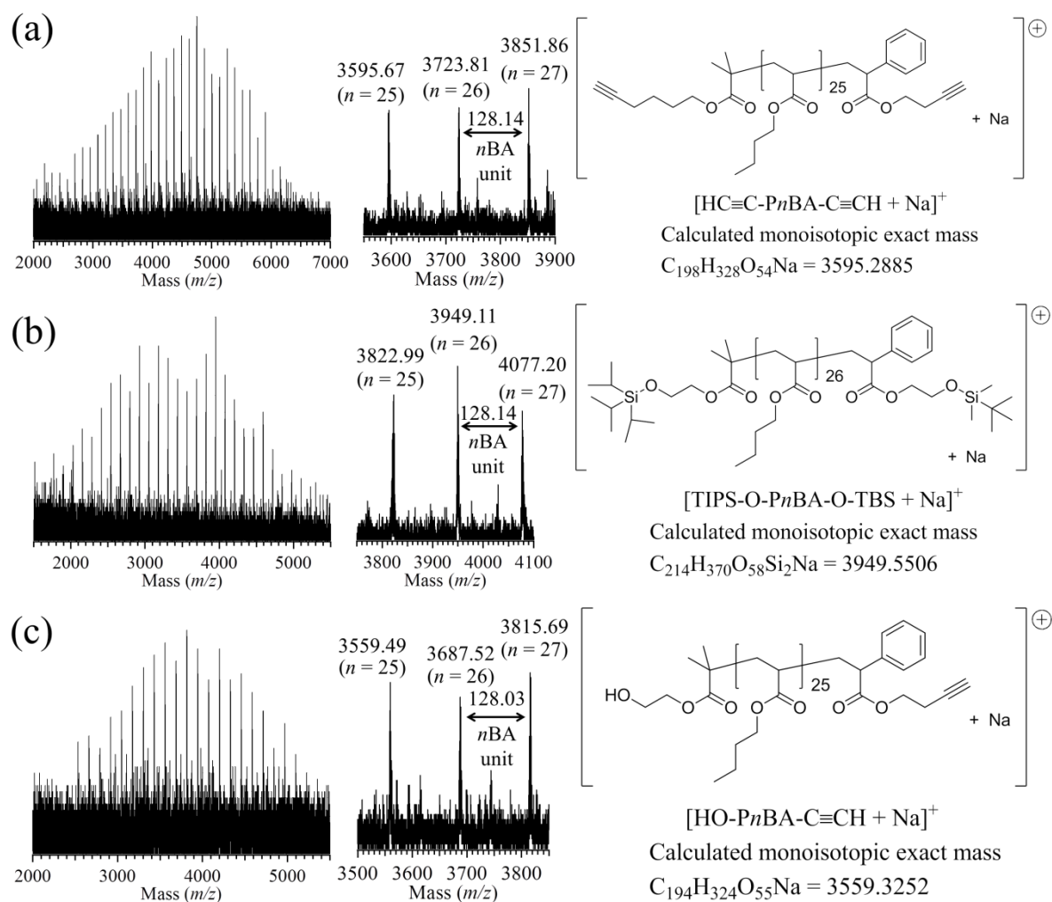
Figure 4-9. MALDI-TOF MS spectra of (a) \text{HC}\equiv\text{C-P}n\text{BA-C}\equiv\text{CH} , (b) \text{HO-P}n\text{BA-OH} with protecting group, and (c) \text{HO-P}n\text{BA-C}\equiv\text{CH} .
