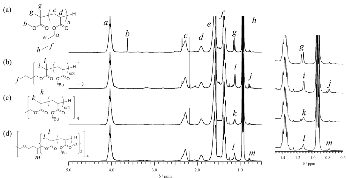
Figure 5-2. ^1\text{H} NMR spectra of (a) linear \text{PnBA} , (b) \text{PnBA}_3 , (c) \text{PnBA}_4 , and (d) \text{PnBA}_8 obtained from GTP (solvent, \text{CDCl}_3 ).
