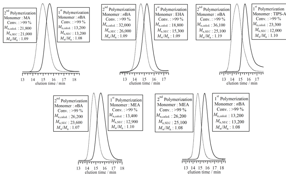
Figure 5-5. SEC traces of the polymers obtained from the first polymerization (solid line) and the second polymerization (dotted line) in the block copolymerization of various monomers (eluent, THF; flow rate, 1.0 \text{ mL min}^{-1} ).
