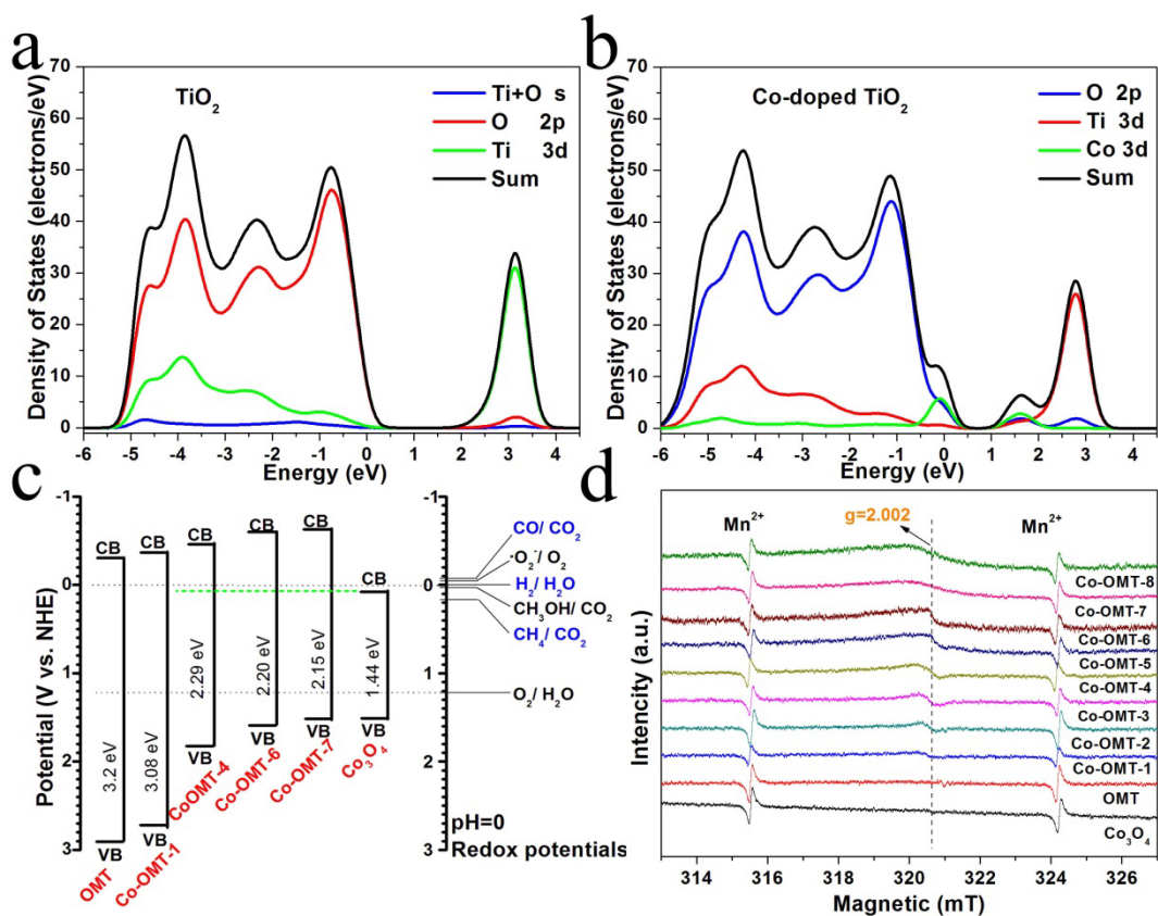
Fig. 7 DOS of (a) anatase \text{TiO}_2 and (b) \text{Co}_x\text{Ti}_{1-x}\text{O}_2 ( x=0.0625 ). (c) schematic illustration of the band structures of the samples. (d) ESR spectra of the samples, and \text{Mn}^{2+} is used as position correction.
