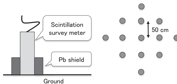
Fig. 1. Measuring method for the surface dose of ground (left) and the layout of 13 points surveyed (right).
