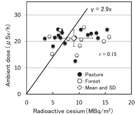
Fig. 3. Relationship between the ambient dose rate and the contamination level of soil. Solid line: relationship based on the conversion factor reported by IAEA (2000)
