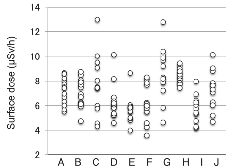
Fig. 4. Variation of the surface dose rate of ground in each section.
