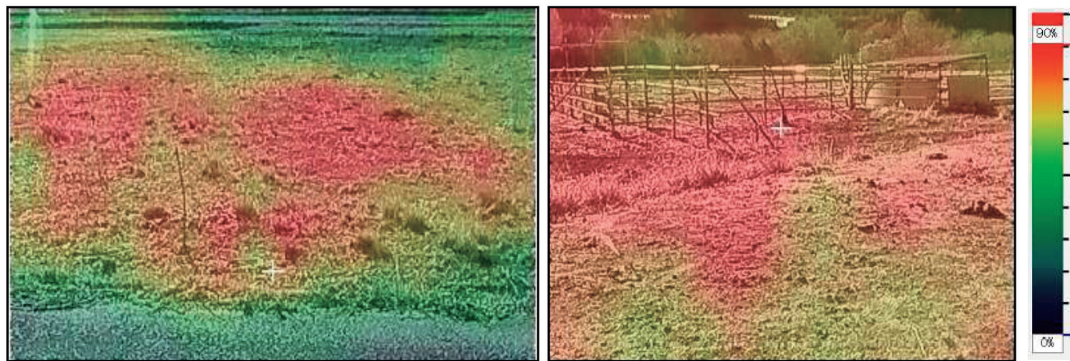
Fig. 5. Gamma ray photographs at this farm. The color expresses relative intensity of gamma ray.
