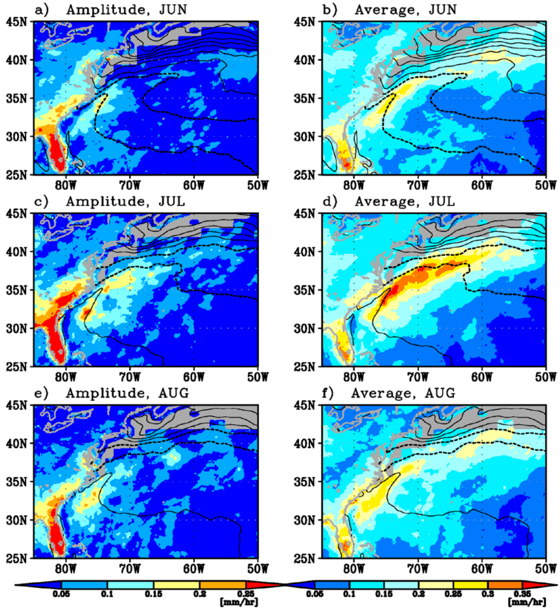
Fig. 4. Amplitudes of 24-hour diurnal cycle (left) and mean rain rate (right) of precipitations over the Gulf Stream region in June (top), July (middle) and August (bottom). Gray areas in left panels are excluded from the analysis, because missing data rate due to presence of ice is larger than 20%. Contours in each panel indicate SSTs with a contour interval of every 2°C and dashed contours for 24° and 26°C.
