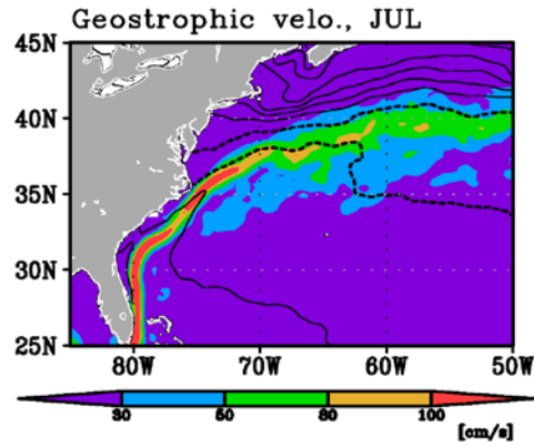
Fig. 5. Climatological absolute surface geostrophic velocity derived from satellite altimeter (color) and SSTs (contours) with a contour interval of every 2°C and dashed contours for 24° and 26°C in July.
