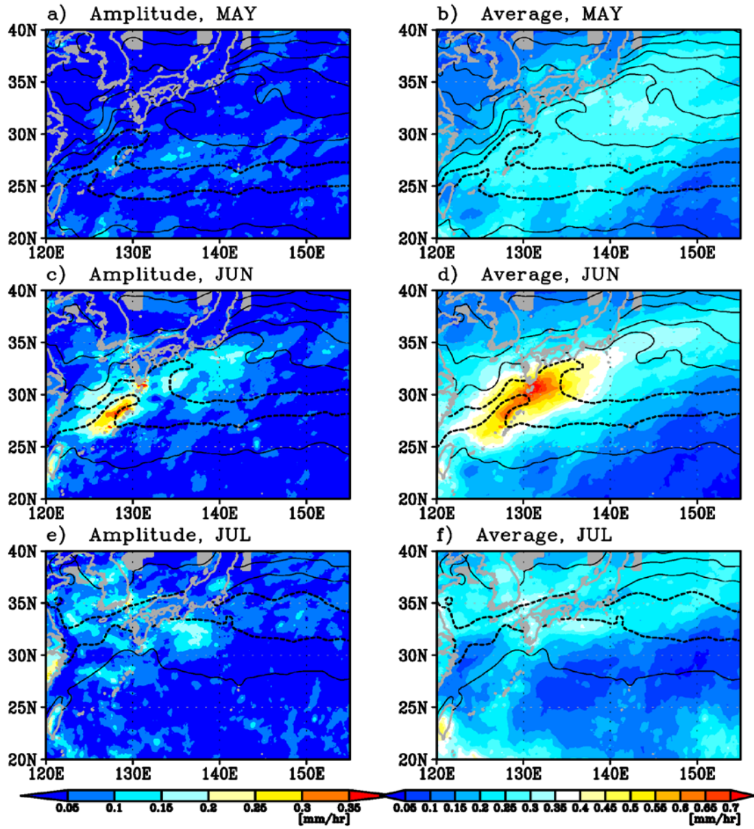
Fig. 10. Same as Fig. 4, but for the Kuroshio region in May (top), June (middle) and July (bottom). Note that the color-scale values are larger than those in Fig. 4.
