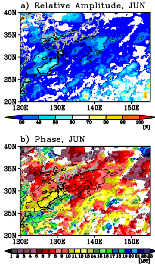
Fig. 12. Same as Fig. 6, but for the Kuroshio region in June. Contours indicate 0.1 (thin contour) and 0.2 mm/hr (thick contour) of the amplitude shown in Fig. 10 (c).
