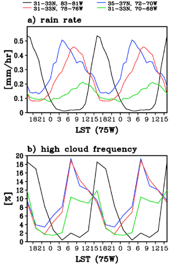
Fig. 9. Climatological time series of (a) rain rate and (b) high cloud frequency in July averaged over different areas. Black line indicates a box over land (31°–33°N, 83°–81°W), blue line indicates a box for the off-shore diurnal precipitation maximum (35–37°N, 72–70°W), red line indicates a box for the near-shore diurnal precipitation maximum (31°–33°N, 76°–78°W), and green line indicates a box to the east of the near-shore maximum (east of the Gulf Stream) (31°–33°N, 72°–78°W).
