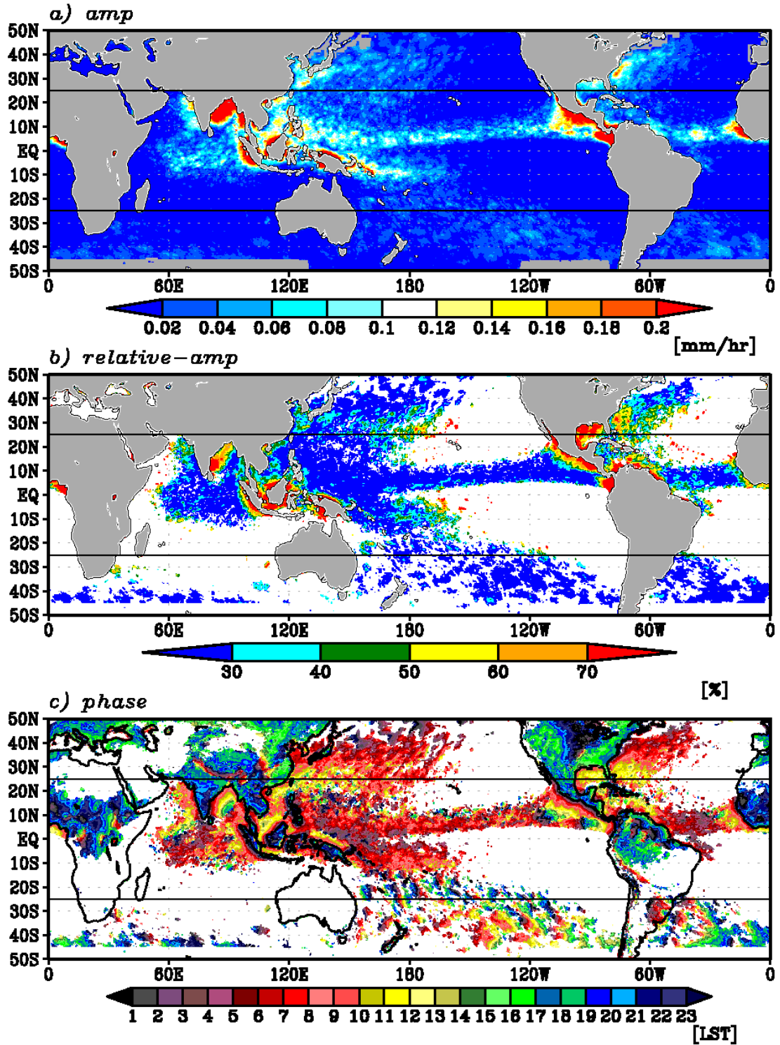
Fig. 2 a) Amplitude, b) relative amplitude and c) phase of diurnal precipitation cycle in boreal summer (June-August). Gray areas over the ocean in panel (a) are excluded from the analysis, because missing data rate due to presence of ice is larger than 20%. The values in panels (b, c) are drawn for the region where the amplitudes are larger than 0.02 mm/hr. Horizontal lines indicate 25°N/S.
