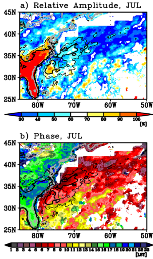
Fig. 6. a) Relative amplitudes and b) phases of the precipitation diurnal cycle over the Gulf Stream region in July. Phases shown by the time of maximum value of 24-hour cycle in LST. Contours indicate 0.1 (thin contour) and 0.15 mm/hr (thick contour) of the amplitudes shown in Fig. 4 (c). White regions are either missing data, due to presence of ice being larger than 20%, or the amplitudes shown in Fig. 4 (c) are smaller than 0.02 mm/hr.
