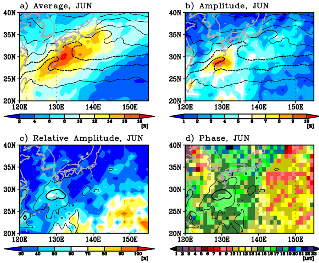
Fig. 13. Same as Fig. 8, but for the Kuroshio region. Note that the color-scale values for panel (a) is wider than those for Fig. 8a.
