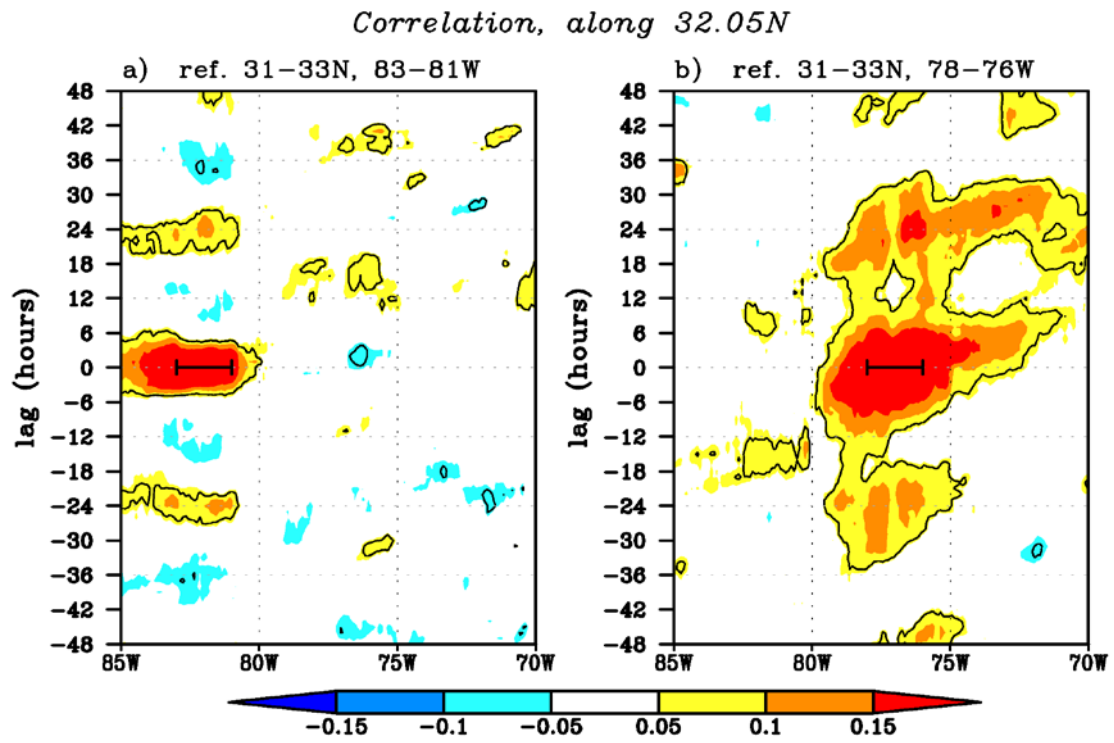
Fig. 7. Lag correlation coefficients at each grid point along 32.05N onto the reference area-averaged precipitation time series (a) in a region 83–81°W, 31–33°N over land and (b) in a region 78–76°W, 31–33°N over the ocean. Positive lags indicate reference time series leading to data at each grid point.
