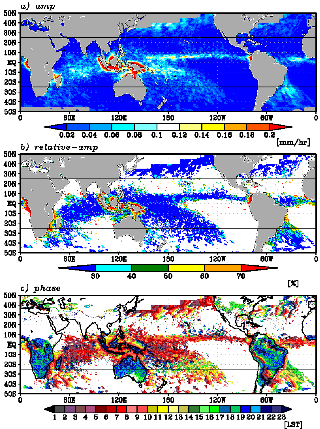
Fig. 3. Same as Fig. 2, but for the boreal winter (December–February).
