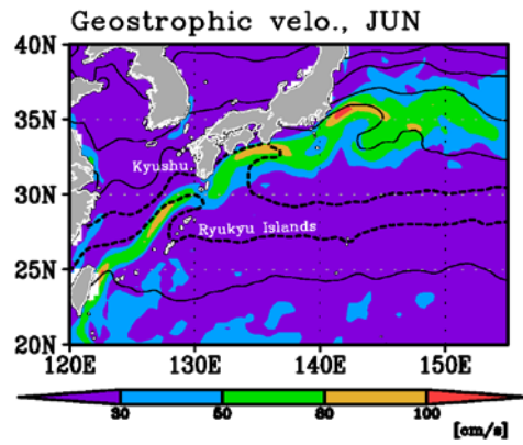
Fig. 11. Same as Fig. 5, but for the Kuroshio region. Kyushu Island and Ryukyu Island are denoted.
