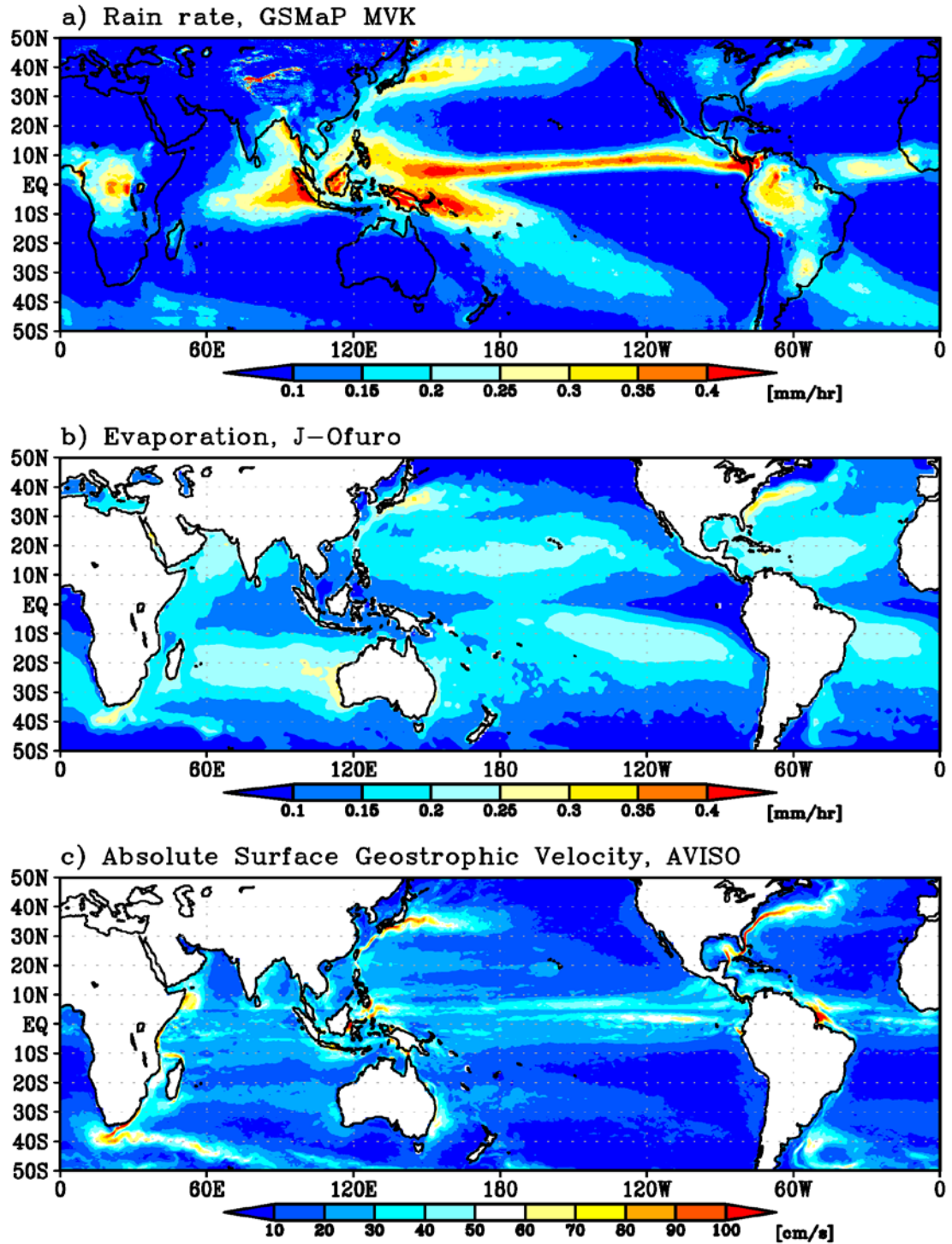
Fig. 1. Annual mean climatology of a) rain rate from GSMaP MVK from March 2000 to November 2010, b) evaporation from the J-Ofuro dataset from January 2000 to December 2006, c) surface geostrophic current velocities provided by AVISO from January 2000 to December 2010.
