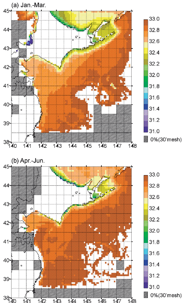
図4：沿岸親潮水の平均塩分。(a)は1～3月、(b)は4～6月。 Figure 4: Mean salinity of the Coastal Oyashio Water within a water column (a) from January to March, and (b) from April to June.
