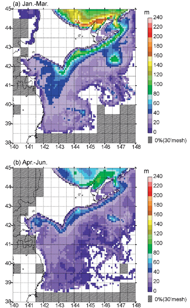
図3：沿岸親潮水の平均層厚。(a)は1～3月、(b)は4～6月。 Figure 3: Mean thickness of the Coastal Oyashio Water within a water column (a) from January to March, and (b) from April to June.
