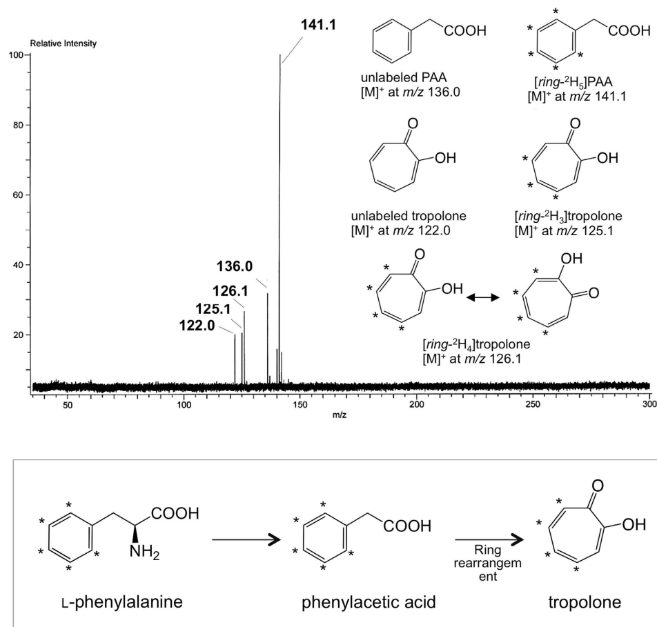
Figure 4. Identification of isotopomeric tropolones and phenylacetic acids from L-[ ring - ^2H_5 ] phenylalanine. FI-MS spectrum of metabolites corresponding to PAA and tropolone obtained from B. plantarii supplemented with L-[ ring - ^2H_5 ]phenylalanine as shown in the top panel. The structures of tropolone, PAA and their isotopomers deduced from the molecular weights are also shown in the same panel. In the conversion of L-[ ring - ^2H_5 ]phenylalanine into [ ring - ^2H_4 ]tropolone via [ ring - ^2H_5 ]PAA, one deuterium at the C-2 or C-6 position was replaced with a proton during the ring rearrangement (bottom panel). Asterisk indicates the position of the deuterated carbon.
