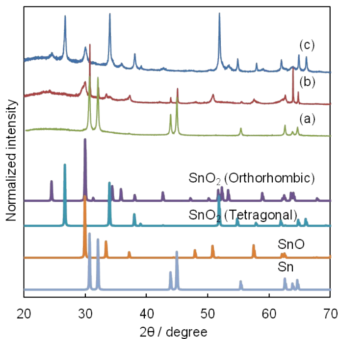
Figure S3. (a) XRD pattern of the as-synthesized Sn NPs using 0.1781 g PVP and of samples after heating to (b) 400 °C and (c) 800 °C. The reference patterns of orthorhombic \text{SnO}_2 (JCPDS no. 29-1484), tetragonal \text{SnO}_2 (JCPDS no. 41-1445), \text{SnO} (JCPDS no. 85-0423), and \text{Sn} (JCPDS no. 04-0673) are shown.
