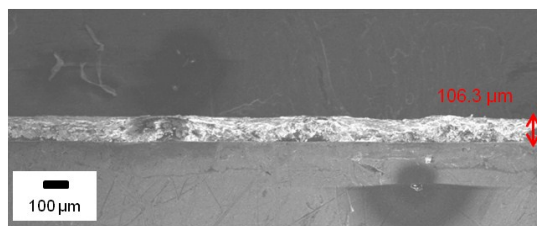
Figure S6. Cross-sectional SEM image of a conductive pattern formed using Sn NPs synthesized using 0.0089 g PVP. The thickness of the pattern was 106.3 \mu\text{m} .
