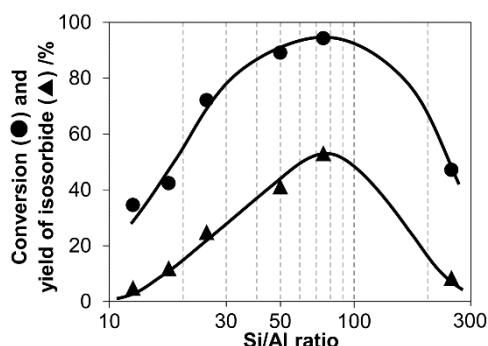
Fig. 1 Effect of Si/Al ratio of H \beta on the dehydration of sorbitol at 400 K for 1 h.
