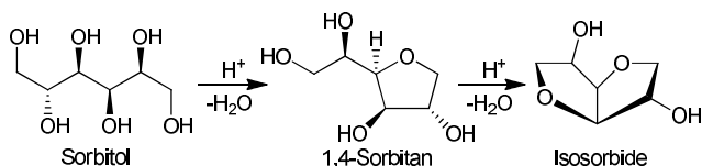
Scheme 1 Dehydration of sorbitol to isosorbide.
