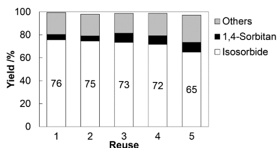
Fig. 2 Reuse experiments of Hβ(75) in the dehydration of sorbitol at 400 K for 2 h.
