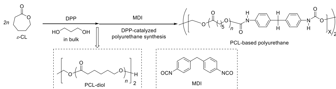
Scheme 3. One-pot synthesis of PCL-based polyurethane using organophosphate-catalyzed bulk ROP system
