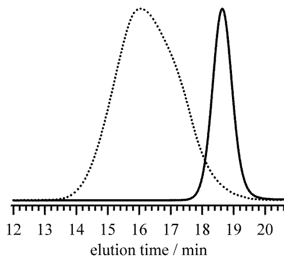
Figure 3. SEC traces of the PCL-diol obtained from the 1st polymerization with the [\epsilon\text{-CL}]_0/[1,3\text{-propanediol}]_0/[DPP]_0 ratio of 25/1/0.05 ( M_{n,SEC} = 5,400 , \bar{D}_M = 1.09 ; solid line) and the obtained PCL-based polyurethane ( M_{n,SEC} = 32,800 , \bar{D}_M = 2.03 ; dotted line) (eluent, CHCl 3 ; flow rate, 1.0 mL min -1 ).
