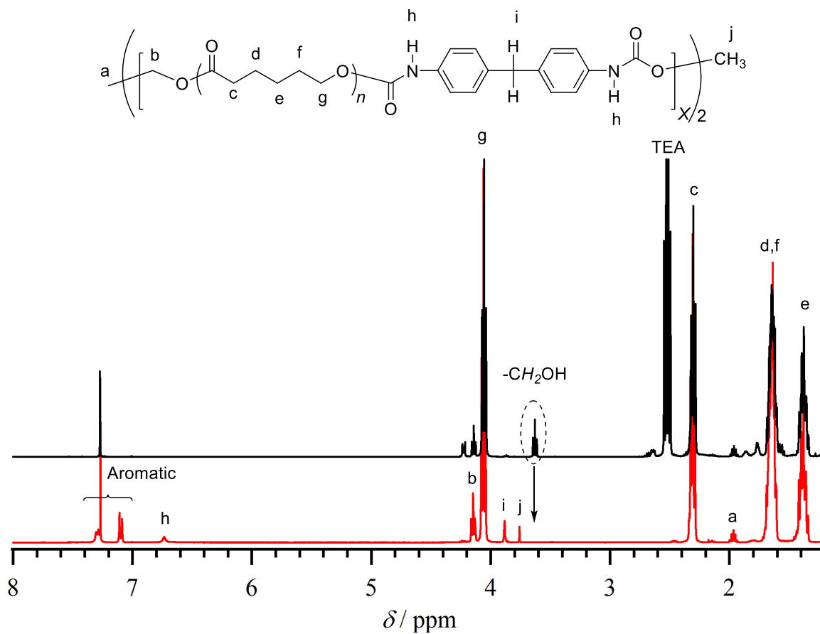
Figure 4. 1 H NMR spectra of the PCL-based polyurethane (red line) and corresponding PCL-diol obtained before adding MDI (conv. = 95.0%; black line) in CDCl 3 .
