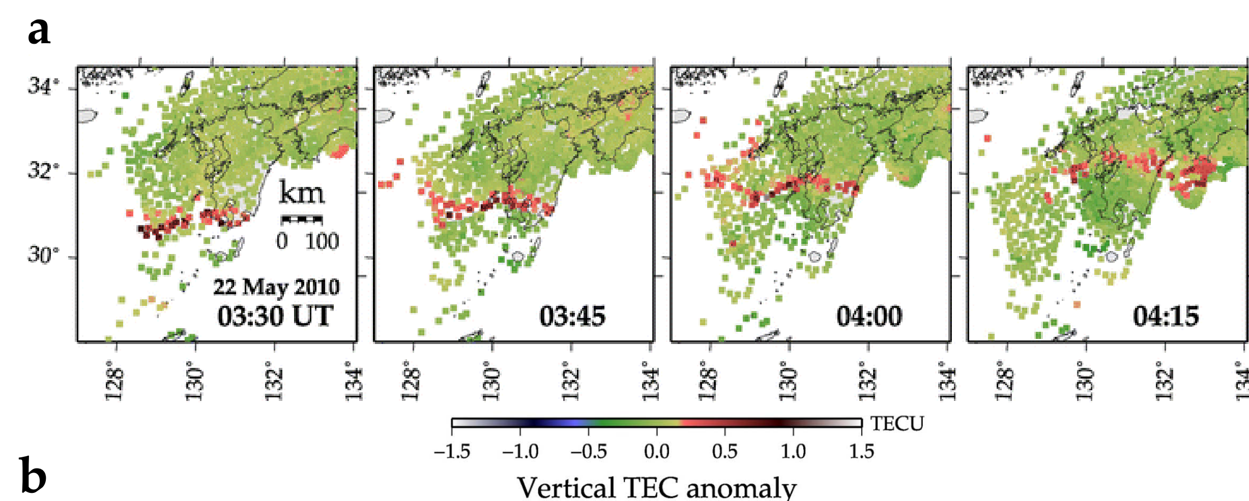
Fig.5 a. Snapshots of vertical TEC anomaly map showing an example of northward propagation of a frontal structure elongated in the E-W direction. In this case, it is clear that the frontal structure propagated to the direction perpendicular to its elongation. Speed and distance of the movement are 40-50 m/s and ~100 km, respectively. b. Local time dependence of the directions of N-S propagation of Es observed in 2010 (histogram). In the histogram, orange and gray represent the numbers of northward and southward movements, respectively. Curves show occurrence rates of Es derived from foEs data obtained during 2003-2012 (dashed) and 2010 (solid) at the Kokubunji ionosonde (with foEs > 10 MHz). Atmospheric tide is considered to control the direction of Es movement.
