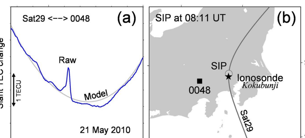
Fig.1 a. Slant TEC time series (observed / model) b. SIP at 08:11 UT (when TEC pulse was observed)
