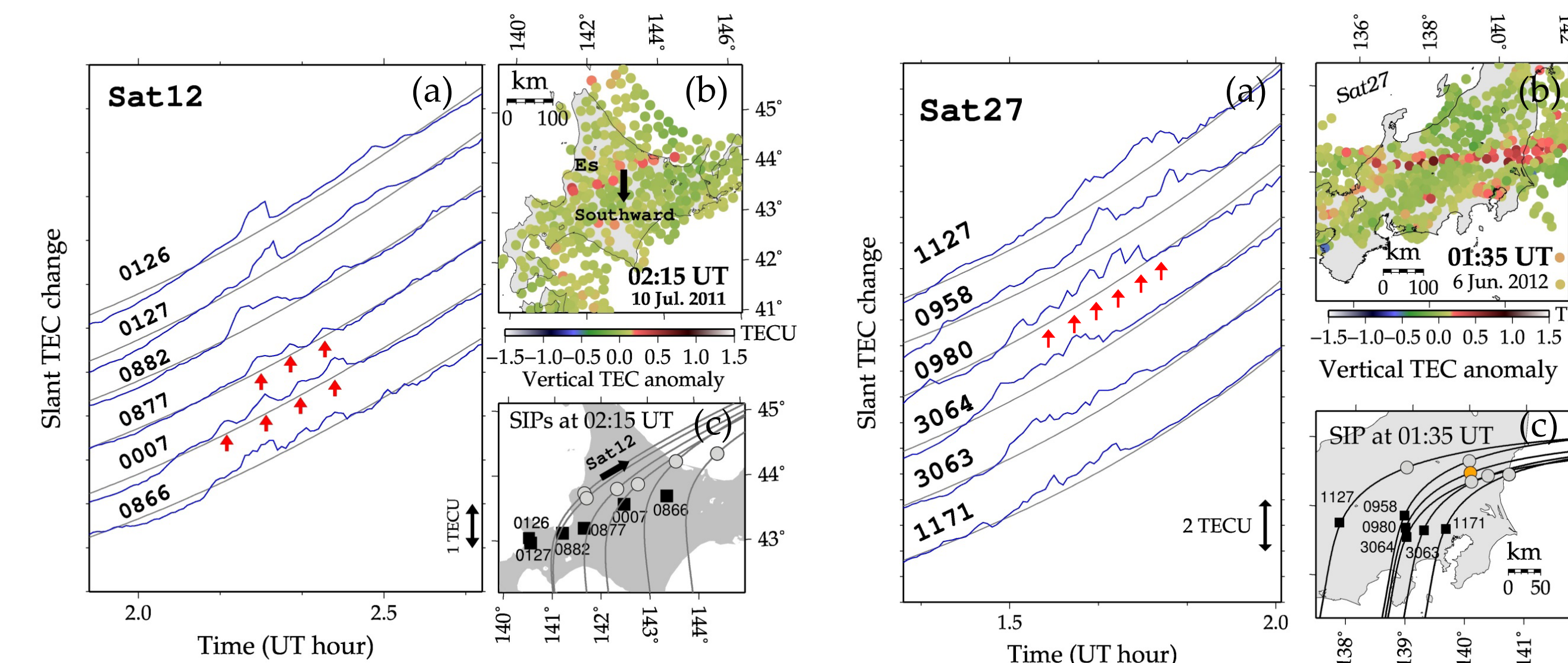
Fig.6 (Left) a. Slant TEC time series drawn by Satellite 12 and six GPS stations, showing typical quasi-periodic (QP) TEC enhancement (especially clear with GPS station 0877 and 0007, pointed by red arrows). b. Vertical TEC anomaly map at 02:15 UT, in which a frontal structure is evident. It elongates in the E-W direction. c. SIP positions with Satellite 12 and six GPS stations at 02:15 UT. SIPs moved east-northeastward, almost tracing the E-W elongation of the frontal structure. These results demonstrate that QP TEC signatures are localized in the central part of the frontal structure. The horizontal separation of QP structure is ~15 km. (Right) a. Another example of along-elongation QP structure observed over the central part of Japan. b. Vertical TEC anomaly map at 01:35 UT, showing an E-W frontal structure which was stationary during the observation. c. SIP positions with Satellite 27 and six GPS stations at 01:35 UT. In a, QP TEC enhancement is clearly observed with the GPS station 0980 while other stations show irregular TEC changes. The location of SIP of 0980 is shown as an orange circle in the SIP map. In this case, either, the QP structure is quite localized in a small region. The horizontal spacing of the QP structure is ~10 km.
