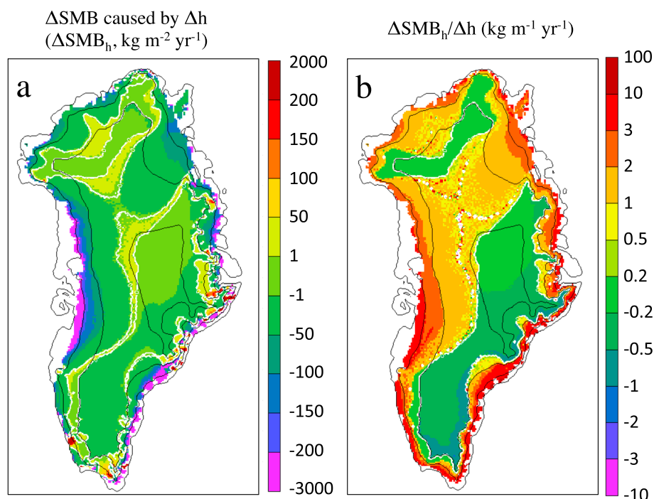
Figure 3. (a) The 2080–2099 SMB anomaly ( \text{kg m}^{-2} \text{yr}^{-1} ) with respect to 1980–1999 associated with elevation change under RCP8.5. (b) Ratio between Figure 3a and elevation change, quantifying the elevation-SMB feedback ( \text{kg m}^{-1} \text{yr}^{-1} ). The zero contours and elevation contours at 1000 m intervals are shown in white and black, respectively.
