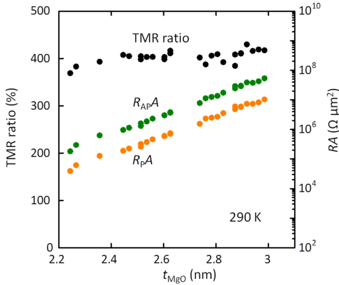
FIG. 2. Typical dependence of R_P A , R_{AP} A , and TMR ratio on MgO barrier thickness ( t_{\text{MgO}} ) at 290 K for CMFS MTJs with \text{Co}_2\text{Mn}_{1.24}\text{Fe}_{0.16}\text{Si}_{0.84} electrodes fabricated on a 20 \times 20 \text{ nm}^2 MgO(001) substrate for a t_{\text{MgO}} range from 2.2 to 3.0 nm, where A is the nominal junction area of 10 \times 10 \mu\text{m}^2 . The MgO tunnel barrier had a wedge structure, and its nominal thickness was varied from 1.4 to 3.2 nm on each 20 \times 20 \text{ nm}^2 substrate by linearly moving the shutter during the deposition by electron-beam evaporation.
