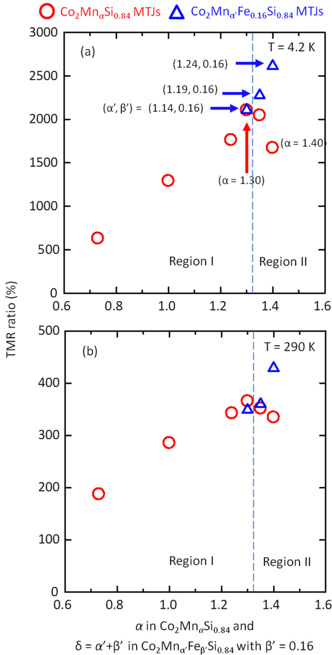
FIG. 10. TMR ratios at (a) 4.2 K and (b) 290 K for CMFS MTJs as a function of \delta = \alpha' + \beta' in \text{Co}_2\text{Mn}_{\alpha'}\text{Fe}_{\beta'}\text{Si}_{0.84} electrodes with \beta' = 0.16 ranging from 1.30 ( \alpha' = 1.14 ) to 1.40 ( \alpha' = 1.24 ). TMR ratios at (a) 4.2 K and (b) 290 K for identically fabricated CMS MTJs as a function of \alpha in \text{Co}_2\text{Mn}_\alpha\text{Si}_{0.84} electrode are shown for comparison [47].
