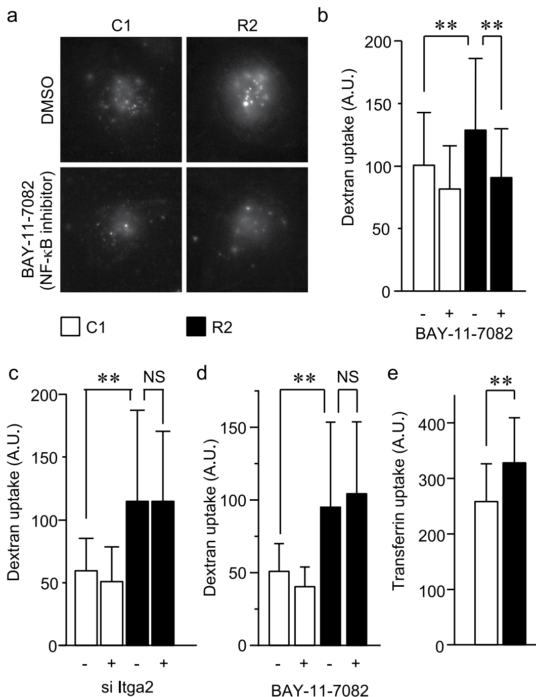
Figure 6. RANKL enhanced endocytosis in a NF- \kappa B-dependent and integrin \alpha 2-independent manner.
