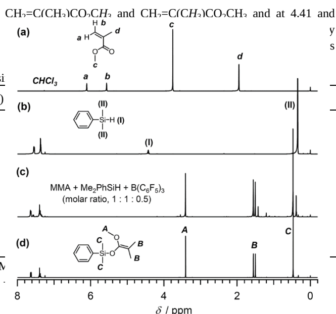
Figure 5. 1 H NMR spectra of (a) MMA, (b) Me 2 PhSiH, (c) MMA + Me 2 PhSiH + B(C 6 F 5 ) 3 , and (d) 1-methoxy-2-methyl-1-dimethylphenylsiloxyprop-1-ene (SKA Me 2 Ph ) in CDCl 3 . chemical shift was observed because the interaction between Me 2 PhSiH and B(C 6 F 5 ) 3 was very weak. Nonetheless, based on the facts that mixing Me 2 PhSiH, B(C 6 F 5 ) 3 , and MMA in CDCl 3 produced SKA Me 2 Ph , while mixing Me 2 PhSiH and MMA in CDCl 3 did not, it is rather clear that B(C 6 F 5 ) 3 catalyzed the in situ 1,4-hydrosilylation of MMA with Me 2 PhSiH.
