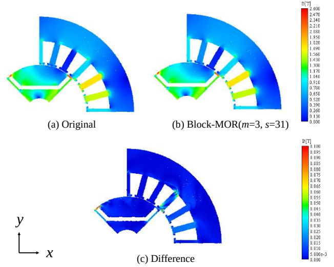
Fig. 7. Distribution of flux density when \theta=45^\circ .
