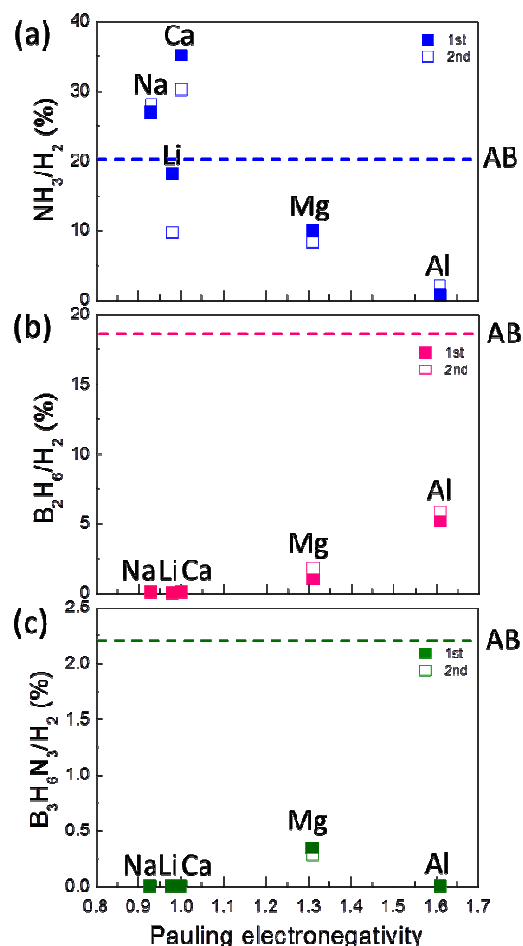
Fig. 1 The amounts of by-product gases desorbed from AB- \text{MH}_n mixtures classified by the Pauling electronegativity of M; (a) ammonia ( \text{NH}_3 ), (b) diborane ( \text{B}_2\text{H}_6 ) and (c) borazine ( \text{B}_3\text{H}_6\text{N}_3 ). The heating rate was 2^\circ\text{C min}^{-1} . The filled squares show the results of 1st measurement and the white square shows the results of 2nd measurement.
