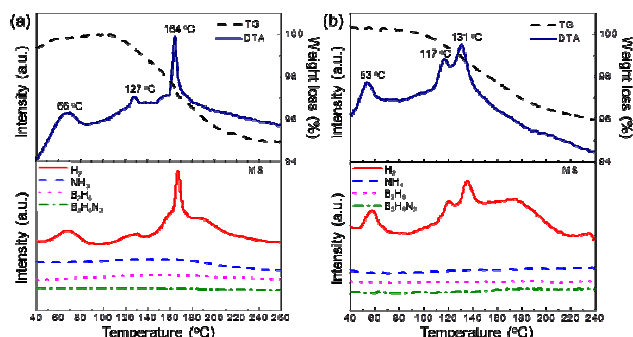
Fig. 2 TG-DTA-MS profiles of ball-milled AB-MAIH 4 (M = Na, Li) mixtures; (a) AB-NaAlH 4 , (b) AB-LiAlH 4 mixture. The heating rate was 5 °C min -1 .
