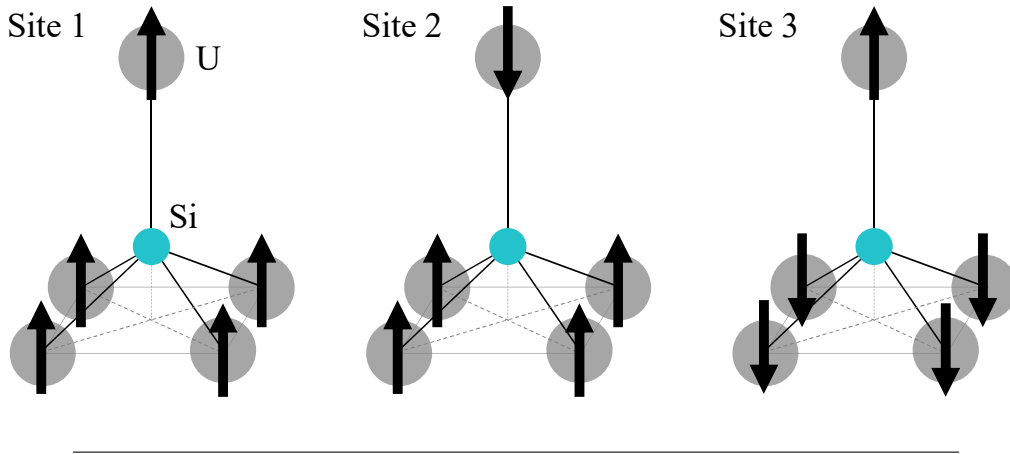
FIGURE A.3: Schematic view of spin configurations around three magnetically-nonequivalent Si sites in the magnetic structure of \mathbf{q}=(0, 0, 2/3) .
