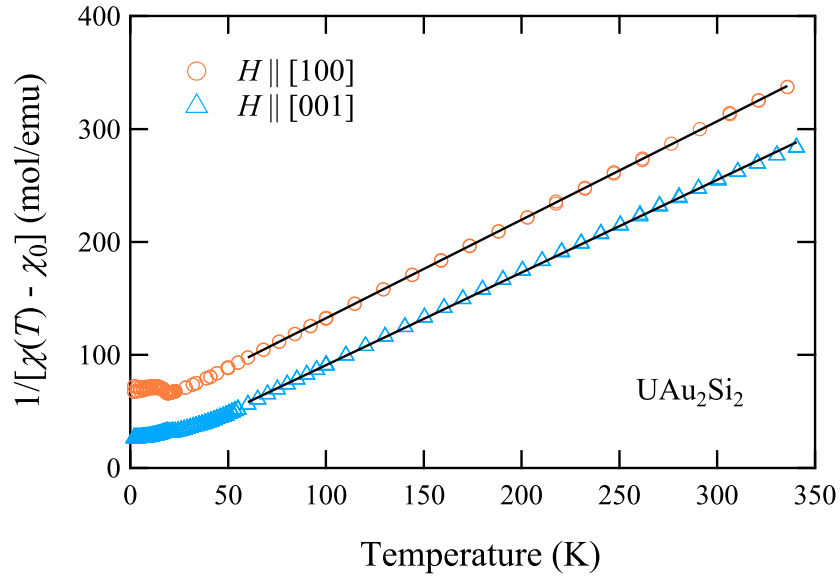
FIGURE 4.6: Temperature dependence of the inverse susceptibility from which the constant contribution is subtracted by using the formula described in the text.
