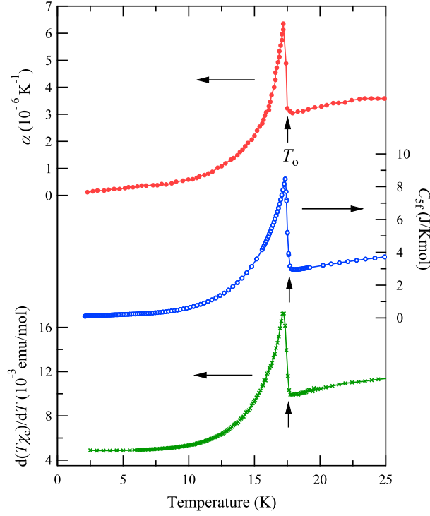
FIGURE 3.7: Temperature variations of 5f-electronic specific heat C_{5f} [64], linear thermal-expansion coefficient \alpha_V [47] and a temperature derivative of c -axis susceptibility \chi_c multiplied by temperature[64].
