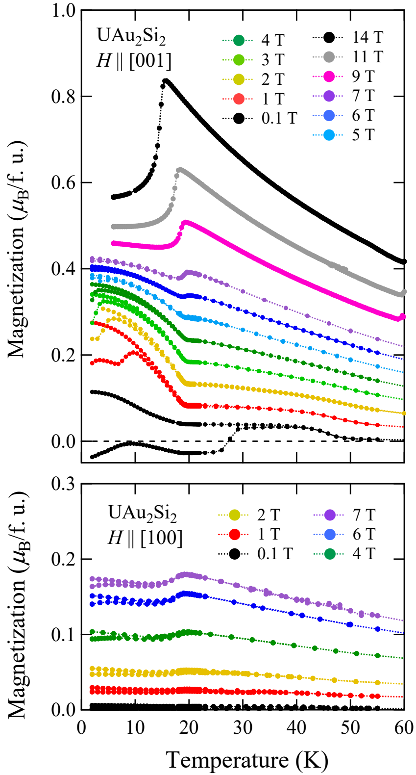
FIGURE 4.9: The temperature dependence of magnetization in \text{UAu}_2\text{Si}_2 in magnetic fields up to 14 T.
