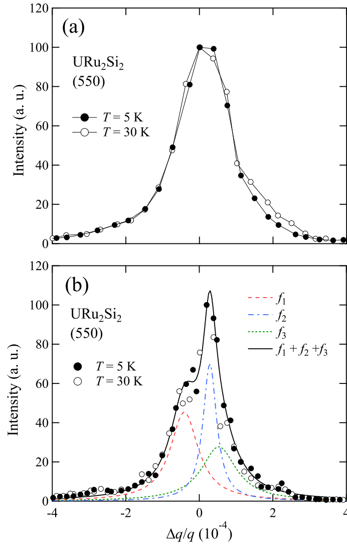
FIGURE 3.6: The (5 5 0) peak profiles of \text{URu}_2\text{Si}_2 measured in (a) normal resolution mode and (b) high-resolution mode at 5 and 30 K. Broken and solid curves represent the best fit of the high-resolution profile with a sum of three Lorentzians.
