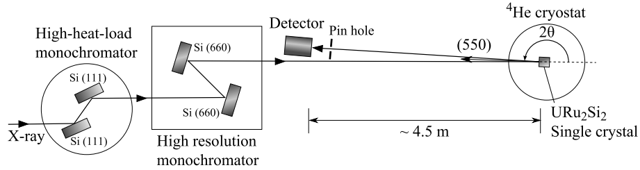
FIGURE 3.1: Schematic view of the experimental set-up.
