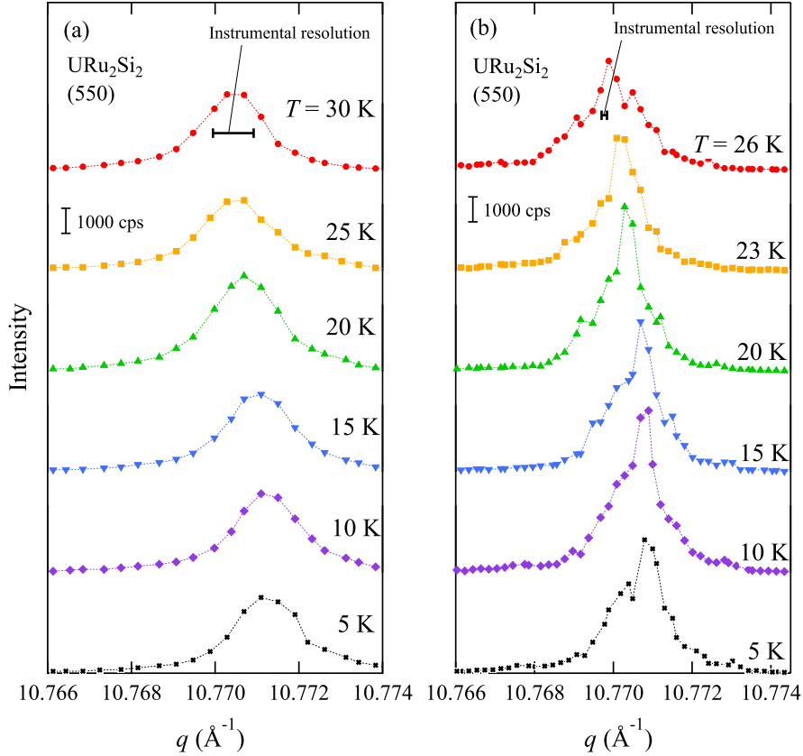
FIGURE 3.4: Examples of the (5 5 0) peak profiles of \text{URu}_2\text{Si}_2 measured in (a) the normal-resolution mode and (b) the high-resolution mode.
