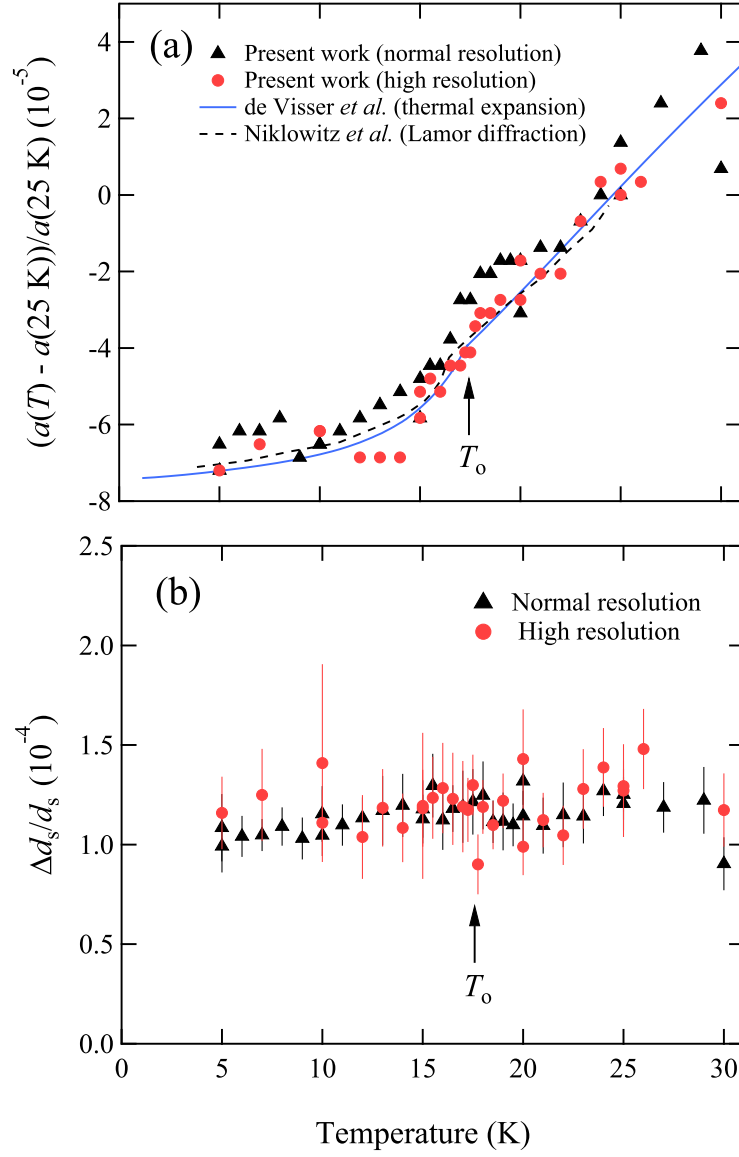
FIGURE 3.5: Parameters obtained from the fitting of the (5 5 0) radial-scan profiles of \text{URu}_2\text{Si}_2 . (a) Temperature dependence of the relative change in the (1 1 0) interplanar spacing and the a -axis lattice parameters extracted from the previous studies of thermal-expansion[47] and neutron Larmor diffraction[56, 57]. (b) Temperature dependence of the relative deviation of the (1 1 0) interplanar spacing. The error bars indicate the standard deviation \sigma of the fitting. The data points in the high-resolution mode are scattered more widely than those in the low-resolution mode. This is due to a worse-fit convergence caused by a fine structure observed in the high-resolution peak profiles.
