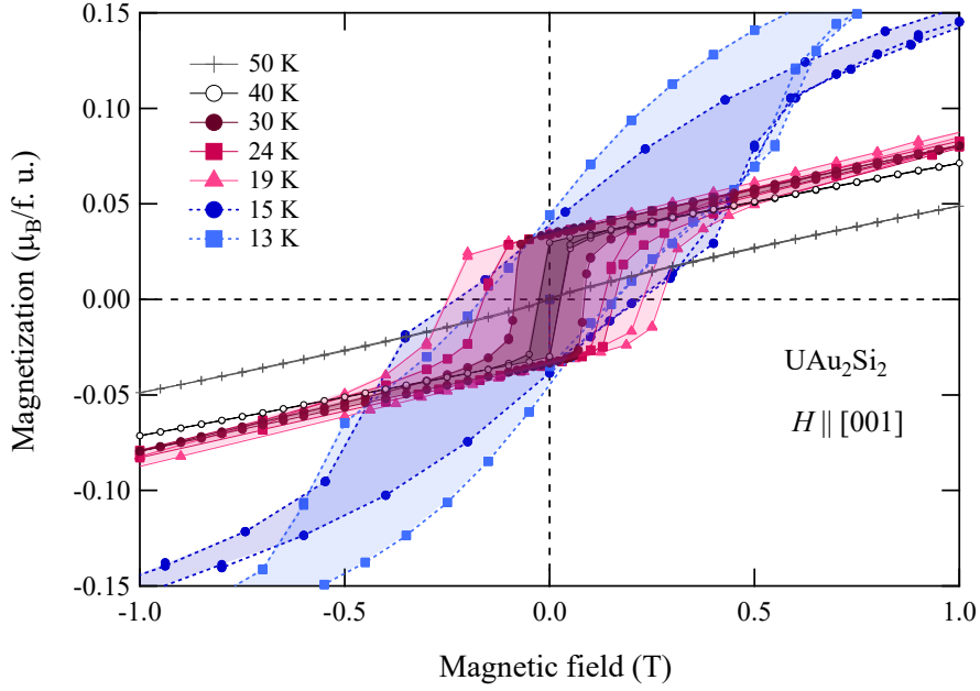
FIGURE 4.8: The hysteresis loops in the magnetization processes in single-crystalline \text{UAu}_2\text{Si}_2 at several temperature points from 13 K to 50 K.
