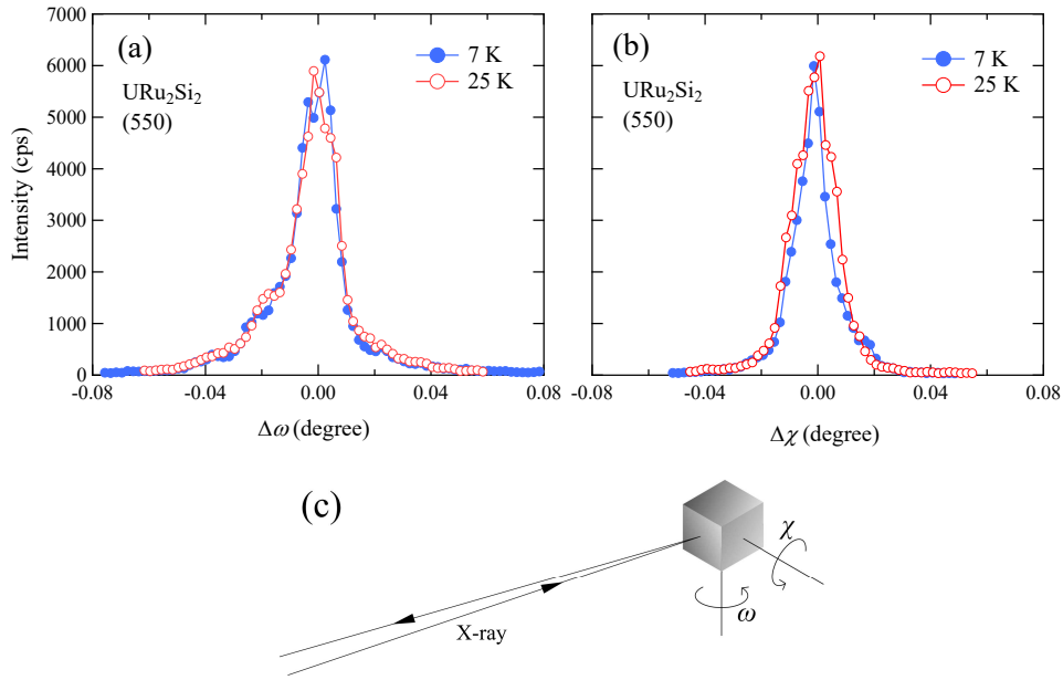
FIGURE 3.3: Experimental results of (a) \omega scan and (b) \chi scan of \text{URu}_2\text{Si}_2 at 7 and 25 K, and (c) schematic view of the definition of two orthogonal tilt angles.
