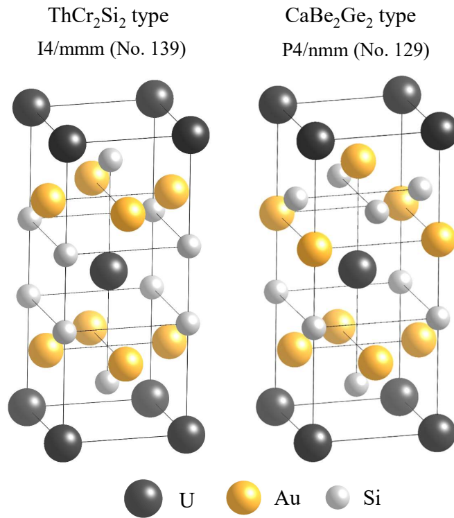
FIGURE 1.1: Two types of crystal structure in which \text{UT}_2\text{Si}_2 systems crystallize.
