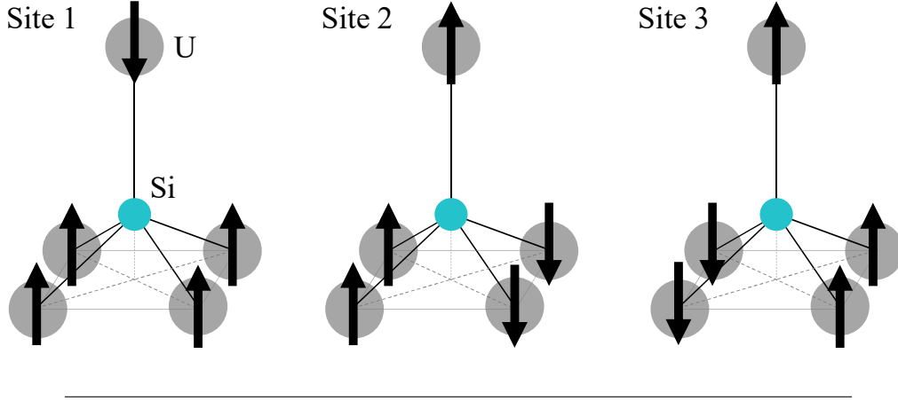
FIGURE A.2: Schematic view of spin configurations around three magnetically-nonequivalent Si sites in the magnetic structure of q=(2/3, 0, 0) .
