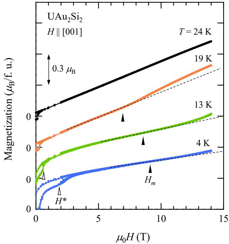
FIGURE 4.10: The magnetization processes in \text{UAu}_2\text{Si}_2 up to 14 T along the [001] direction. The broken line is a guide to the eye.
