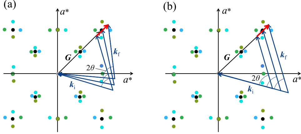
FIGURE 3.2: Schematic view of two different radial-scan methods: (a) a usual \theta - 2\theta scan and (b) a scan by tuning wavelength. Black and color dots in backgrounds indicate the reciprocal lattice points in the basal planes of tetragonal and orthorhombic structures, respectively: Four different colors correspond to four domains.
