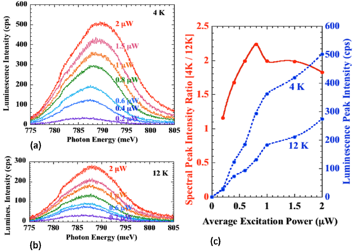
Fig. 5.2 (a) Excitation power dependence of time-averaged luminescence spectra measured at 4K under pulsed excitation. Time-averaged power is given for the pulsed-laser excitation (1 \mu\text{W} corresponds to the pulse peak power of 2.6 mW). cps represents photon counts per second. (b) Excitation power dependence of time-averaged luminescence spectra measured at 12K under pulsed excitation. (c) Excitation power dependence of peak intensity of time-averaged luminescence spectrum at 4K and 12K and the ratio of the peak intensities at 4K to 12 K.
