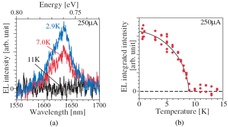
Fig. 2.3 Temperature dependence of (a) EL spectra and (b) EL integrated intensity where the solid line is guide to the eye. T_C of Nb \sim 8.4 K [16].
