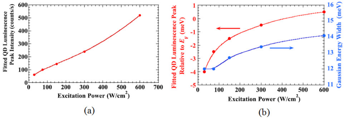
Fig. 4.8 Excitation power dependence of the Gaussian-function parameters used for fitting the spectra in Fig. 4. (a) The QD PL peak intensity. (b) The QD PL peak energy relative to the electron Fermi energy (given by the energy separation \delta ) and Gaussian half energy width (given by \sqrt{2\Delta E} ).
