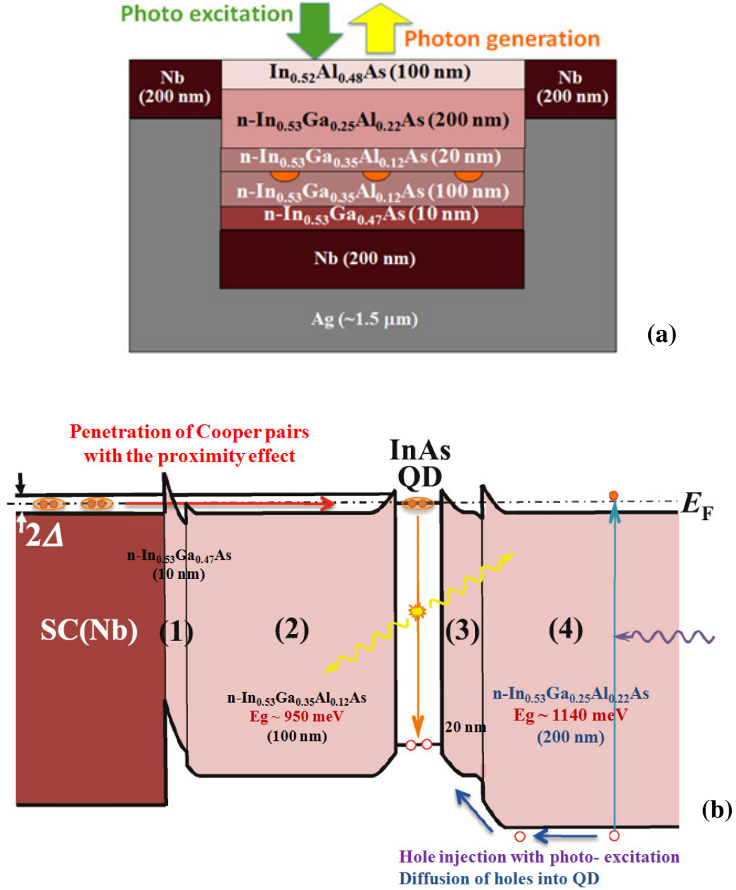
Fig. 3.7 (a) Schematic of Ag-embedded InAs QD heterostructure sample and (b) Schematic band structure of the sample.
