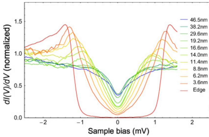
Fig. 3.9 Development of measured local tunneling conductance spectra (normalized) as a function of the distance from the island edge [14].
