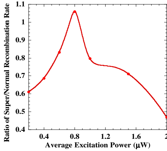
Fig. 5.7 Average excitation power dependence of the ratio of Cooper-pair superconductive to normal radiative recombination rates.
