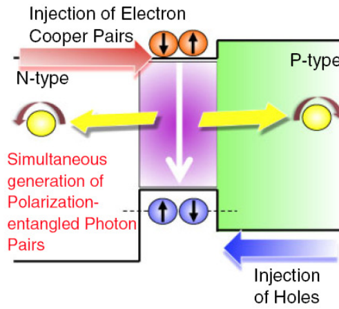
Fig. 6.1 Fundamental band diagram and operation principle of SQLED [7]
