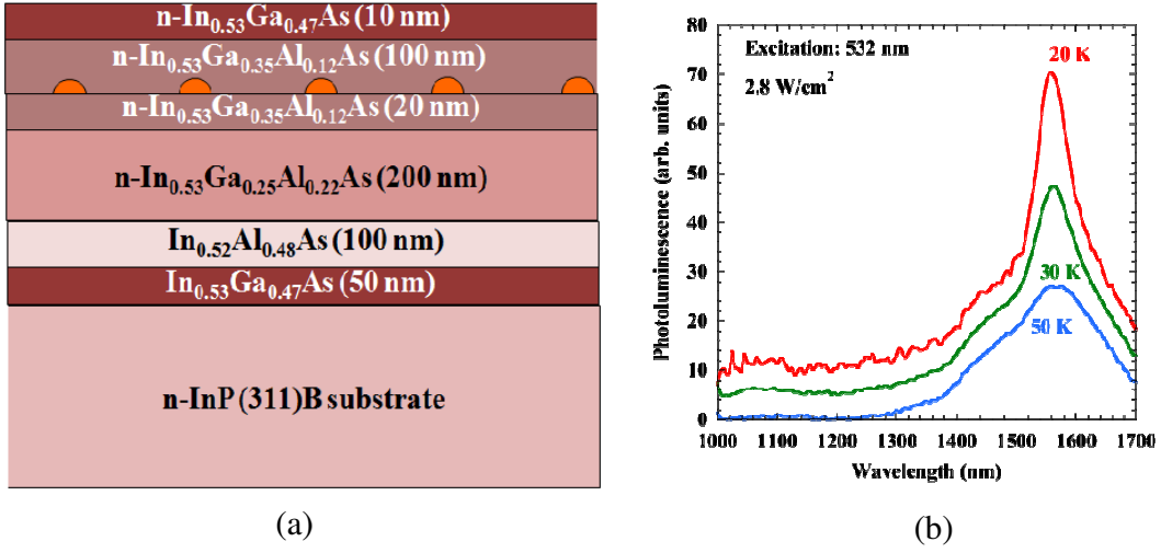
Fig. 3.1 (a) Schematic of InAs QD-based heterostructure sample and (b) Photoluminescence (PL) spectra measured on the heterostructure.
