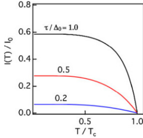
Fig. 2.2 Temperature dependence of theoretically calculated normalized luminescence intensity below the superconducting critical temperature ( T_c ) [9].
