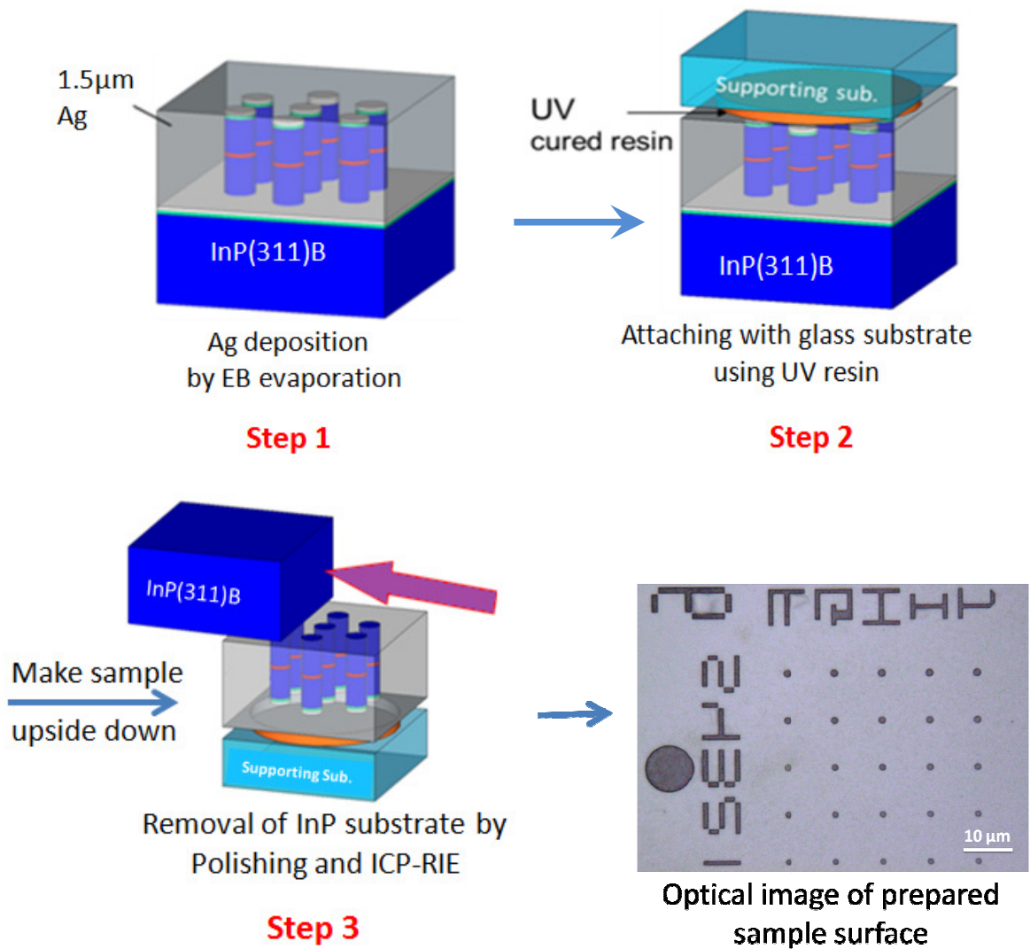
Fig. 3.5 Substrate removal procedure to obtain Ag embedded pillars for higher photon extraction efficiency.
