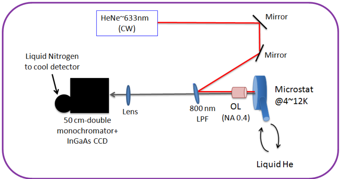
Fig. 4.1 Experimental setup for photoluminescence spectroscopy with CW laser.
