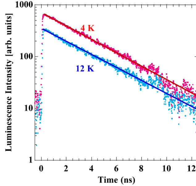
Fig. 5.3 Time decay of luminescence peak intensity from InAs QD emission measured at the wavelength of 1570 nm (790 meV) with the bandwidth of 20 nm (10.1 meV). The average excitation power is 0.8 \mu W (pulse peak power is 2.1 mW). The solid lines are the fitting curves obtained with a single exponential function.
