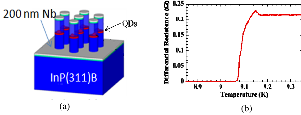
Fig. 3.4 (a) Deposition of Nb superconductor on the fabricated pillars and (b) Determination of the critical temperature ( T_C ) of the Nb layer.
