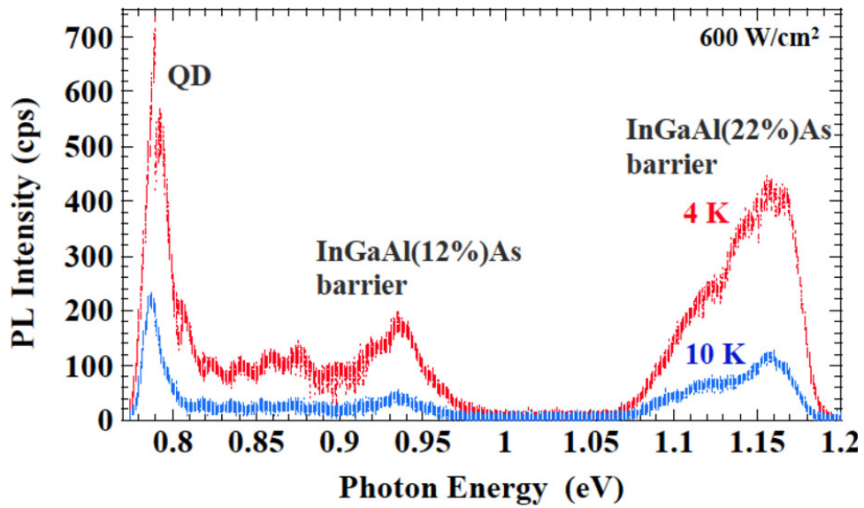
Fig. 4.2 Photoluminescence spectra of the prepared sample measured on one of the pillars with diameter 1.5 \mu\text{m} , below and above SC T_C of Nb ( \sim 9.09 K).
