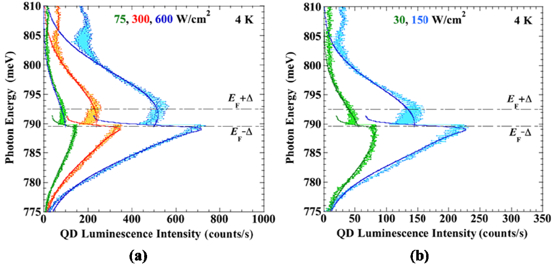
Fig. 4.6 Measured excitation power dependence of QD luminescence spectra. The measured photon counts are connected with neighboring counts with thin lines: (a) 75, 300, and 600 W/cm 2 ; (b) 30 and 150 W/cm 2 . The solid lines are fitting with the parameters of E_F = 791.0 meV and \Delta = 1.42 meV.
