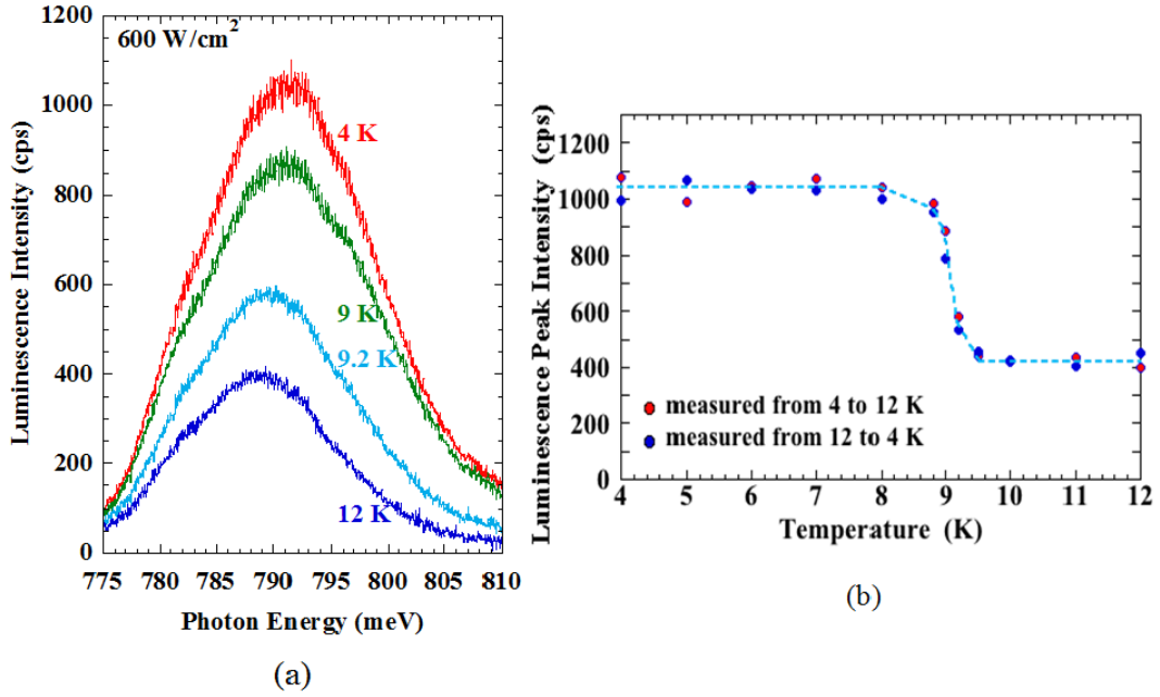
Fig. 4.3 (a) Temperature dependence of InAs-QD luminescence spectra and (b) Temperature dependence of QD luminescence peak intensity. To confirm the relation to T_C of Nb \sim 9.09 K, measured data for the temperature rising and falling sequences are shown.
