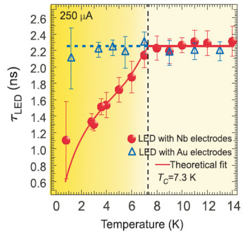
Fig. 2.4 Temperature dependence of the measured LED decay time, \tau_{LED} [17].
