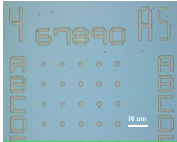
Fig. 3.3 Pillars pattern drawn on the sample by e-beam lithography.
