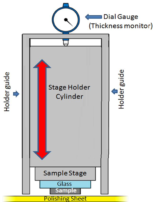
Fig. 3.6 Manual polishing machine used for polishing the InP substrate.
