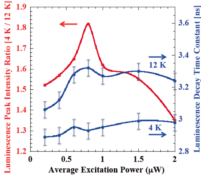
Fig. 5.6 Excitation power dependence of the ratio of the transient QD luminescence peak intensities at 4 K to that at 12 K (left axis) and the luminescence decay time constants with error bars at 4 K and 12 K (right axis).
