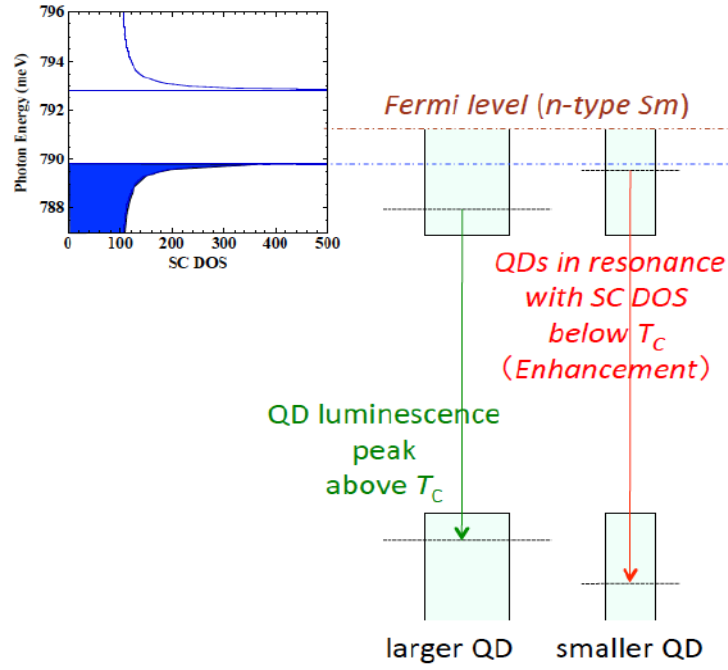
Fig. 4.4 Schematic to show the relation between the SC DOS induced by the proximity effect and the luminescence of QDs. The energy-condensed DOS enhances the luminescence from the smaller QDs, of which conduction-band energy state is near in resonance with the SC DOS.
