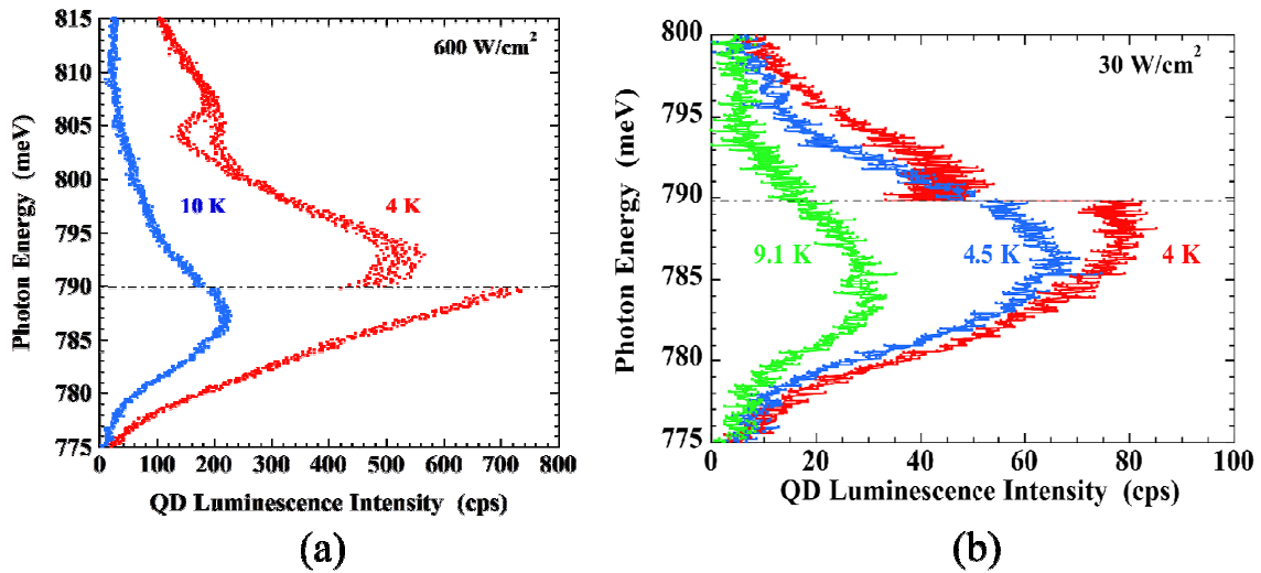
Fig. 4.5 Luminescence spectra of InAs QDs observed from another pillar with the diameter of 1.5\ \mu\text{m} at temperatures below and above SC T_C ( \sim 9.09\ \text{K} ), (a) with strong ( 600\ \text{W/cm}^2 ) and (b) with weak ( 30\ \text{W/cm}^2 ) excitation power. The alternate long and short dashed black line in both figures is the guide to the eye, indicating the luminescence intensity sharp edge.
