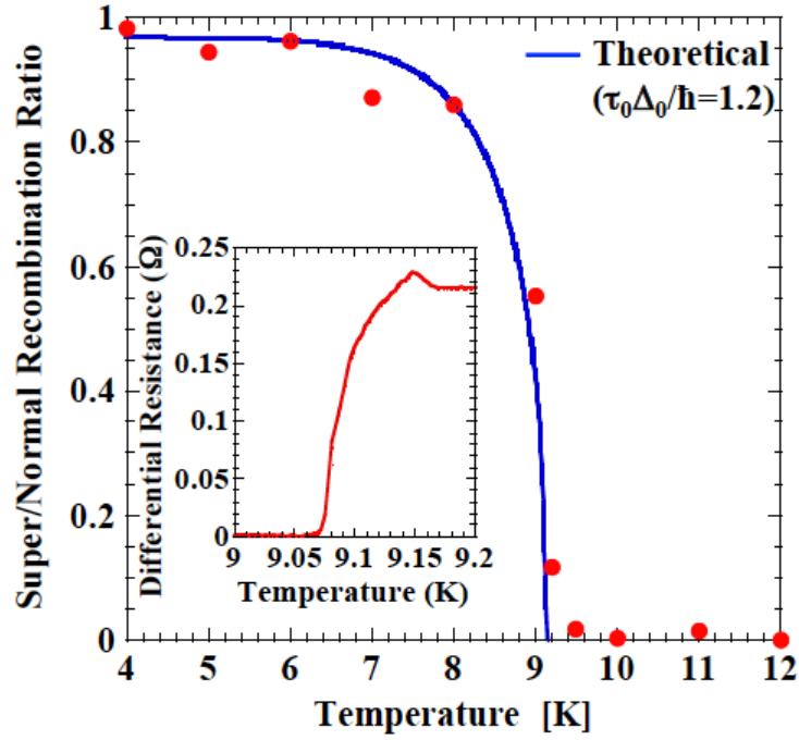
Fig. 5.5 Temperature dependence of the ratio of superconductive to normal radiative recombination rate. Closed circles are data from measurements. The solid line is theoretical based on Ref. 9. \Delta_0 is half of the SC gap (pair potential) at zero temperature and \tau_0 is the relaxation time due to elastic impurity scattering. The inset graph is the temperature dependence of the differential resistance measured on the evaporated Nb layer expanded near T_C .
