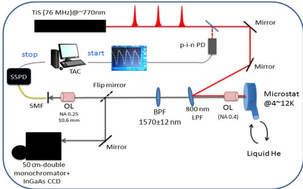
Fig. 5.1 Experimental setup for time resolved photoluminescence spectroscopy.
