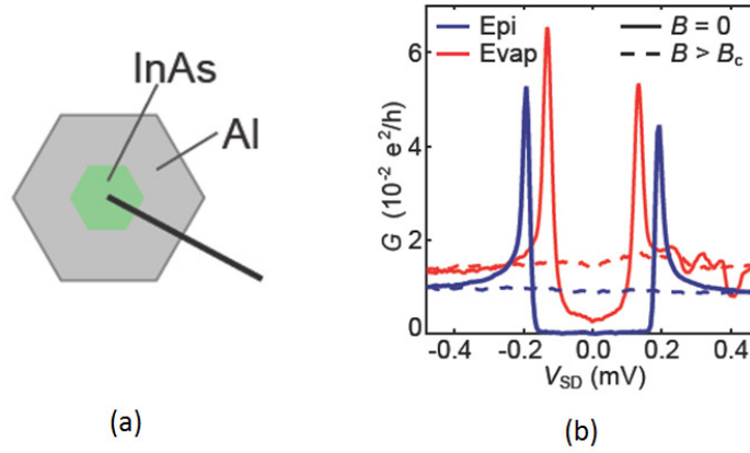
Fig. 3.10 (a) Schematic cross section of epitaxial full-shell nanowire with InAs core and Al shell and (b) Differential conductance as a function of source-drain voltage of an epitaxial full-shell device and an evaporated control device [15].
