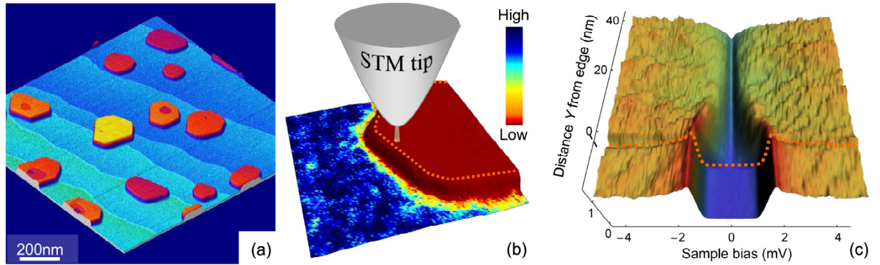
Fig. 3.8 (a) STM image of Pb superconductor islands in wetting layer on undoped Si substrate. (b) Color-coded STS tunneling conductance map superimposed onto 3D topographic STM image. The colors correspond to the conductance variations. (c) Spatial variations of the local dI(V)/dV spectra as a function of the distance from the island edge. The dashed line corresponds to the spectrum taken at the island edge [14].
