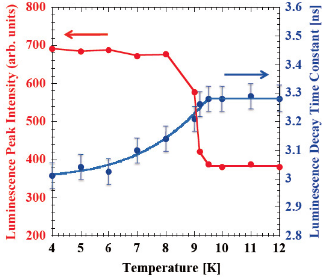
Fig. 5.4 Temperature dependence of transient luminescence peak intensity and luminescence decay time constant with error bars measured at an average excitation power of 0.8 \mu\text{W} .
