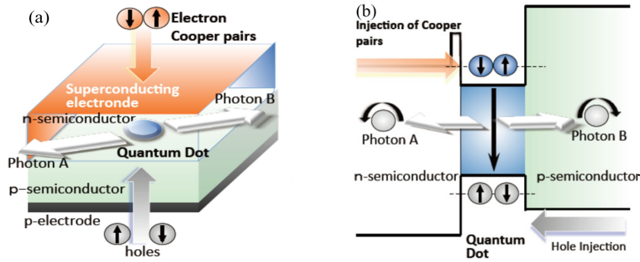
Fig. 2.1 Schematic of (a) SQLED and (b) the relevant band structure. Electron Cooper pairs are injected from the SC n-type electrode to a QD. The hole population in the valence QD state limits the recombination rate.
