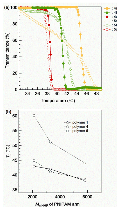
Figure 6. (a) The transmittance dependence on temperature for polymer 5 and its macroligand 4 in aqueous solutions and (b) the T_c dependence on M_{n,NMR} of the PNIPAM arm for polymers 1 , 4 , and 5 in aqueous solutions.
