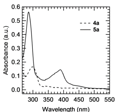
Figure 4. UV-Vis absorption spectra of 4a (dashed line) and 5a (solid line).
