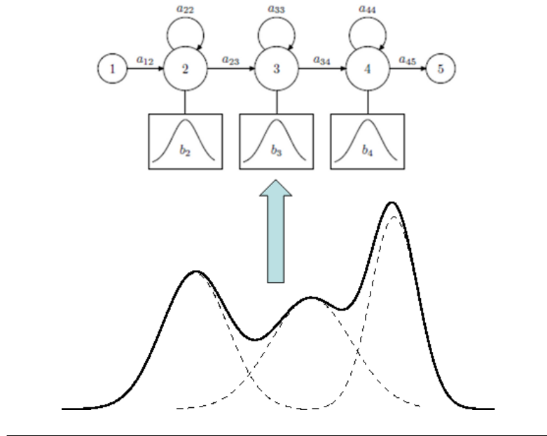
FIGURE 3.5: Illustration of Gaussian mixture modeling.
