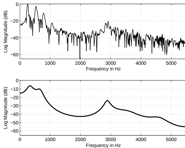
FIGURE 4.4: FFT and spectral estimate from LPC
