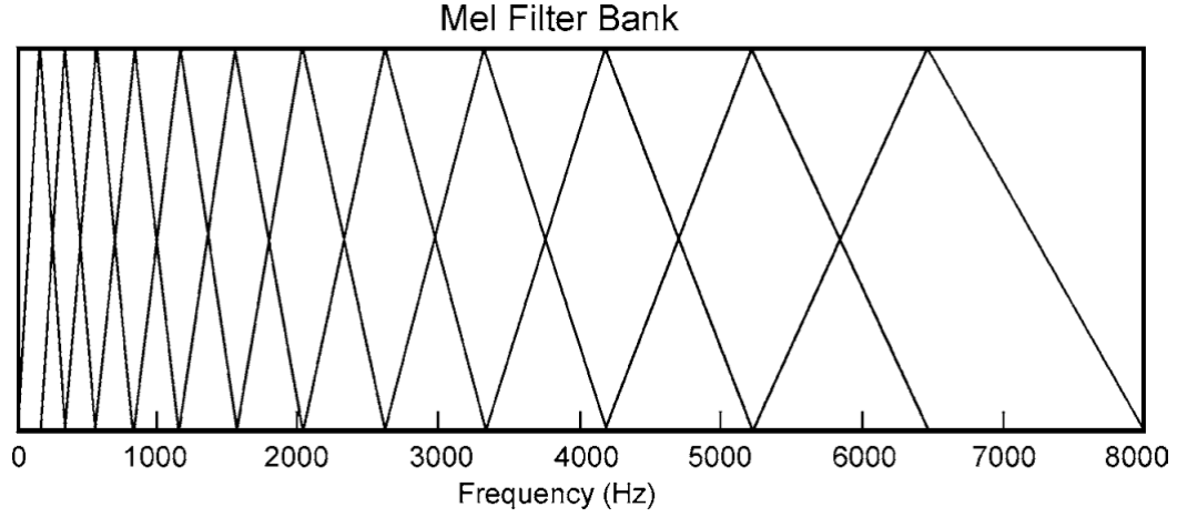
FIGURE 3.3: Triangular filterbank example for mel-frequency computation.
